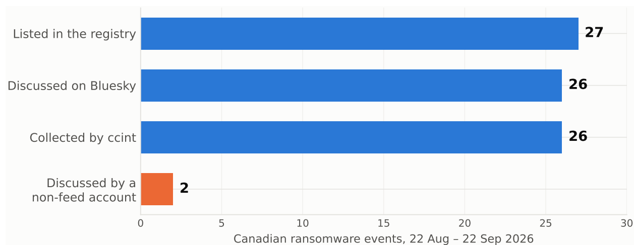
Figure 3: The same 27 Canadian ransomware events at four successive gates. The attrition is almost entirely at the last one, and the last one is not a property of this system.
