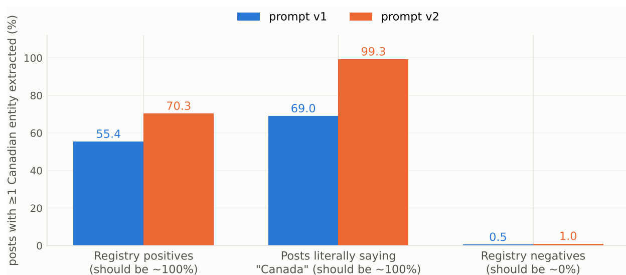
Figure 2: Entity-extraction recall on three probe sets before and after the prompt revision. The middle set is the diagnostic one: these are posts that literally contain the word Canada , so any answer below 100% is a failure of the instrument rather than a hard judgement call.
