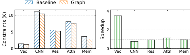
Fig. 2. Existing workload comparison. Graph preprocessing preserves makespan on solved workloads and reduces model constraints; solve-time speedup is workload-dependent.
