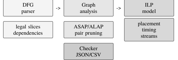
Fig. 1. Solver flow. Graph preprocessing narrows issue windows and removes safe operation-pair constraints before the shared ILP model is solved and checked.
