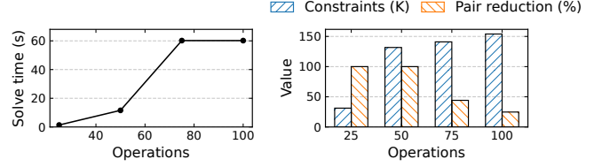
Fig. 3. Generated scalability workloads. The 75- and 100-operation cases reach feasible schedules at the 60 s limit and pass the domain checker.
