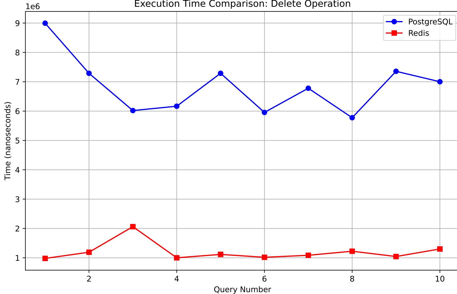
Execution Time Comparison: Delete Operation
