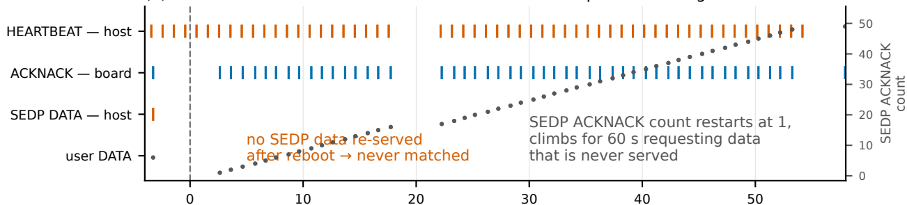
(a) Stalled run: SEDP ACKNACKs never answered — endpoint matching deadlocks
