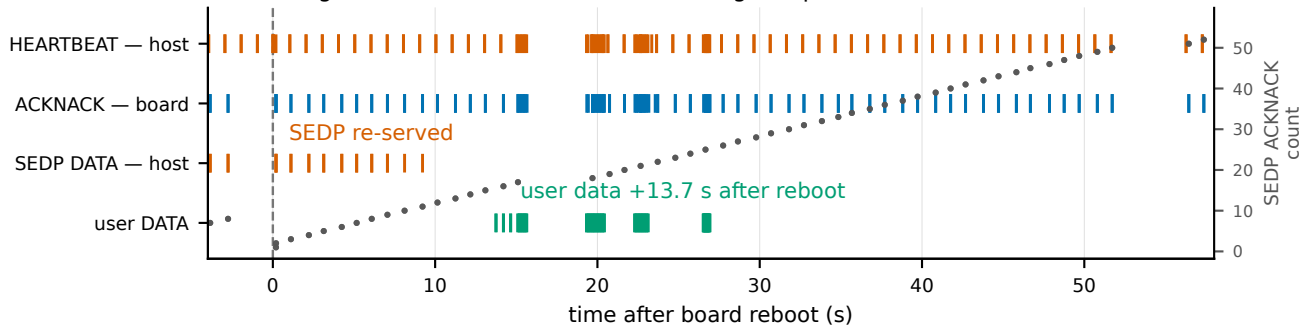
(b) Passing run: SEDP data re-served, matching completes, user data flows
