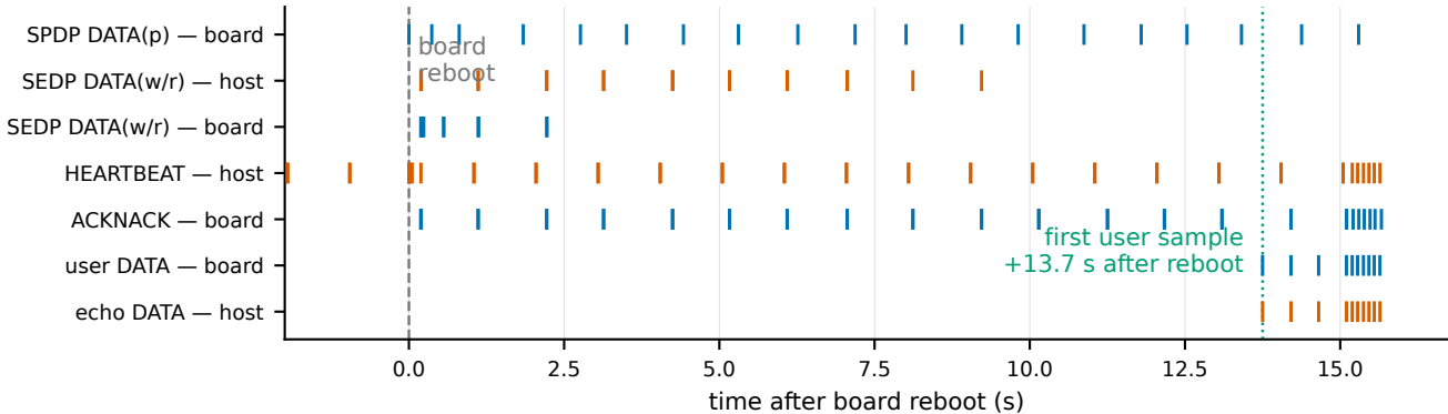
Post-reset discovery handshake: ESP32 (embeddedRTPS) ↔ ROS 2 host (Fast DDS)
