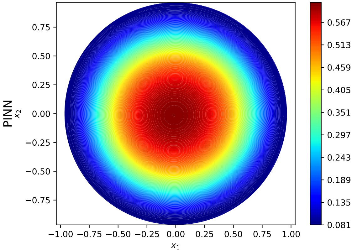
Numerical solution
