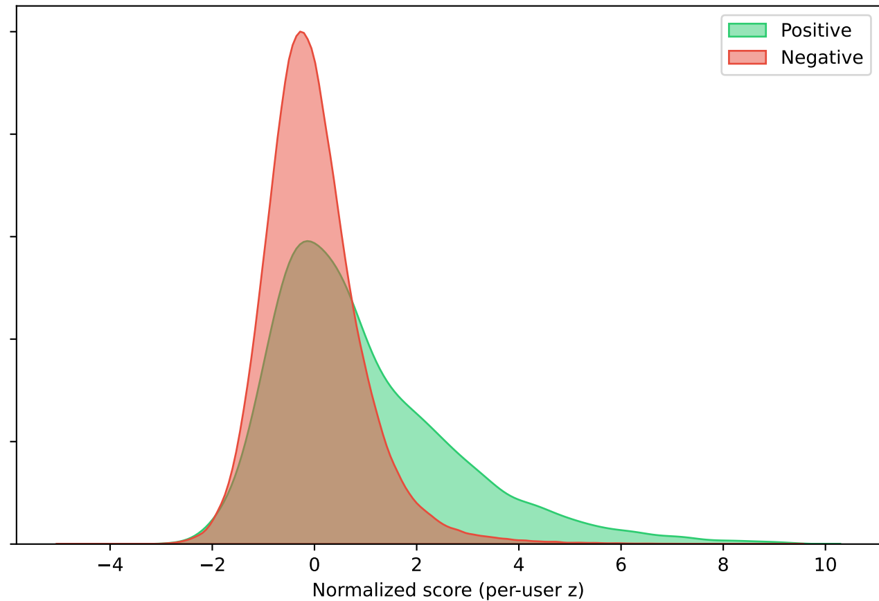
Full: gap = 0.964
