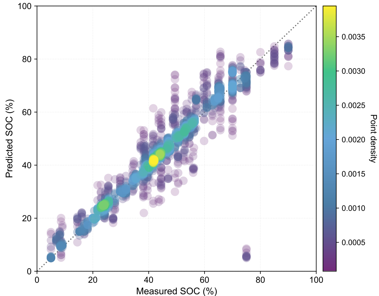
SOC Test Median APE = 5.431%
