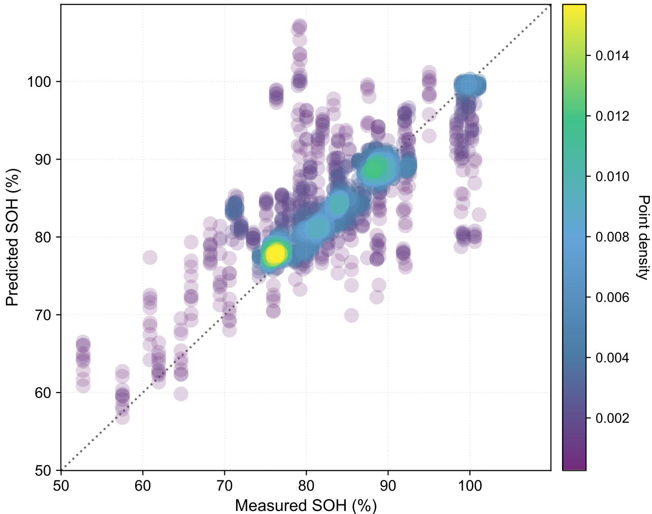
SOH Test Median APE = 2.821%
