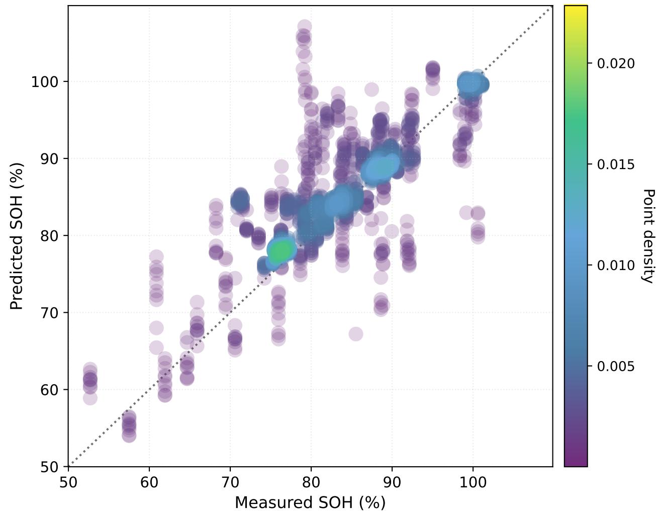
SOH Test Median APE = 2.615%
