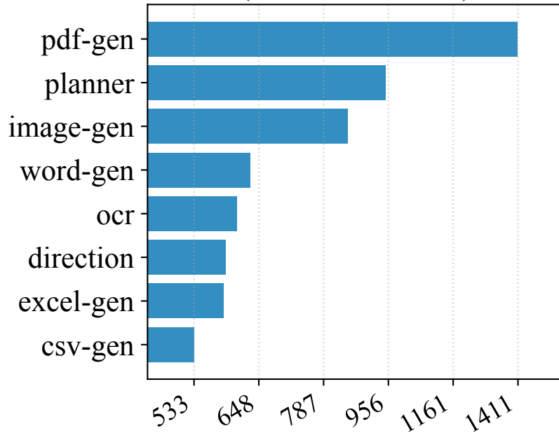
Mean Memory usage (MB) (max/min \approx 3\times )
