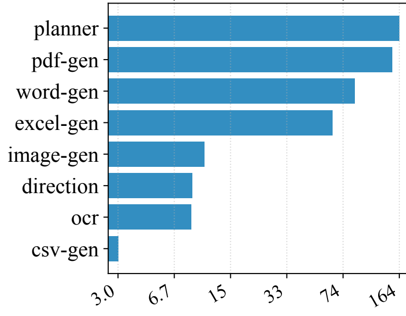
Median Execution time (s) (max/min \approx 55\times )
