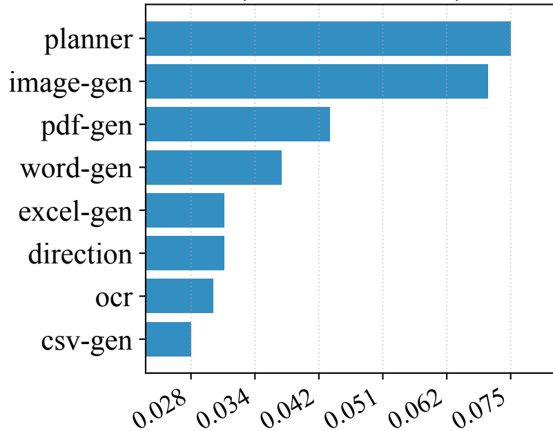
Mean CPU usage (cores) (max/min \approx 3\times )
