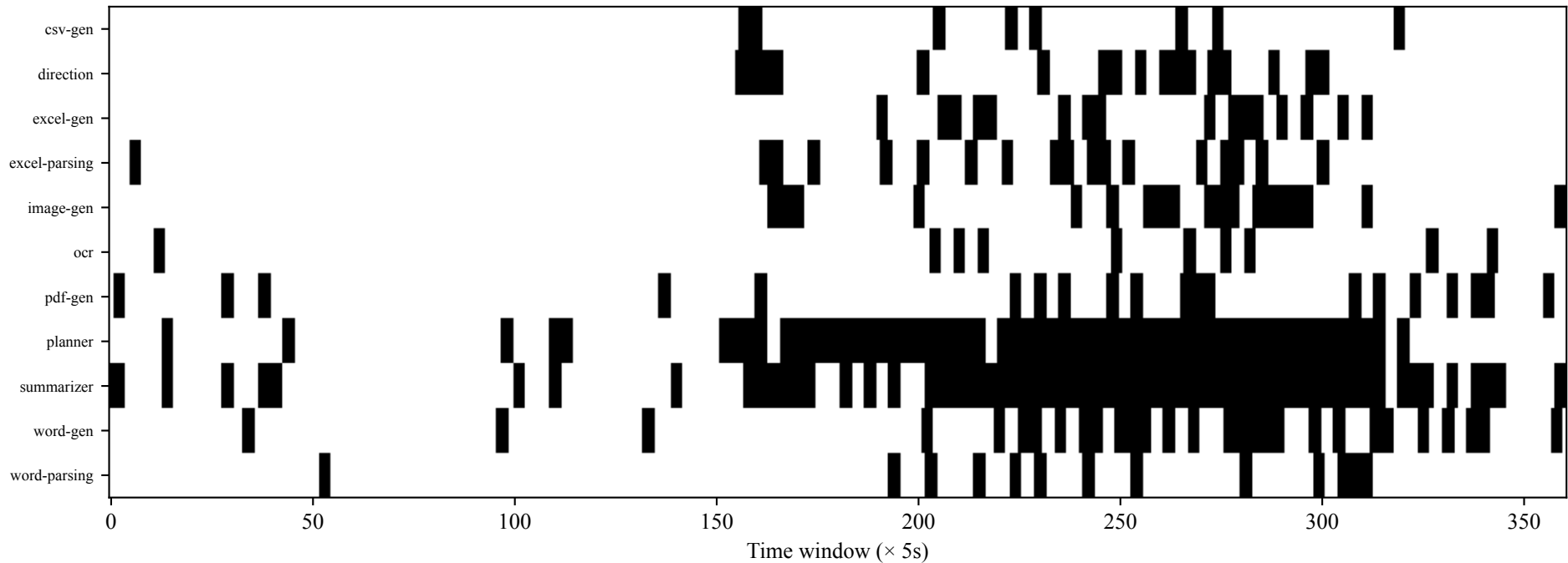
Observability of the p90 latency metric across different agent services at a user load of 5 (Black = value present, White = missing).
