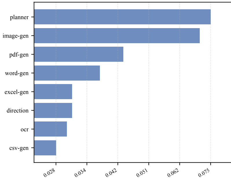
Mean CPU usage (cores) (max/min \approx 3\times )
