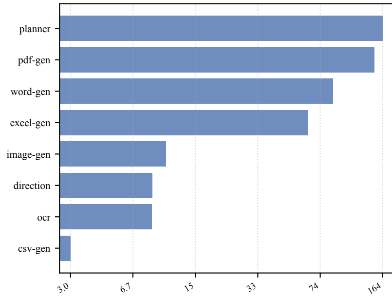
Median Execution time (s) (max/min \approx 55\times )
