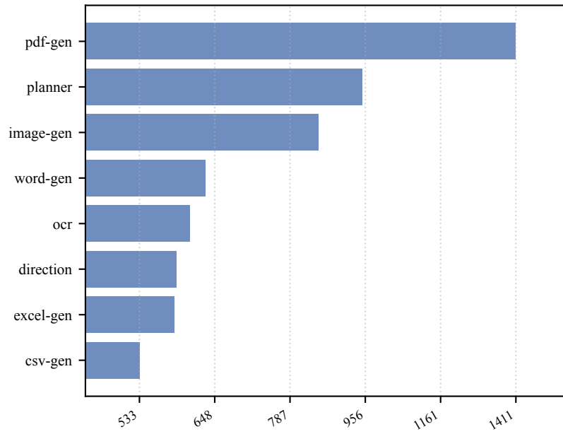
Mean Memory usage (MB) (max/min \approx 3\times )
