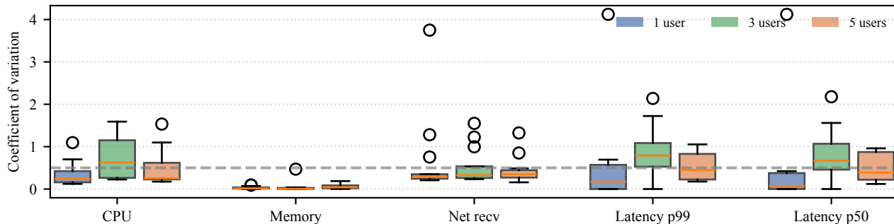
(a) Variability of metrics under normal workload
