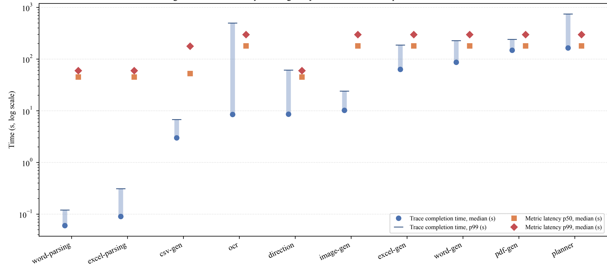
The histogram-bucketed latency metric grossly distorts the real completion time at a user load of 5.
