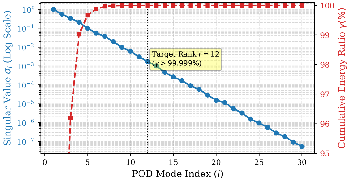
POD Singular Value Spectrum & Energy Decay
