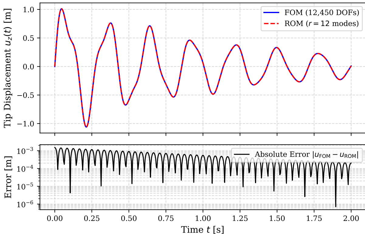
Transient Elastodynamic Tip Displacement & Approximation Error
