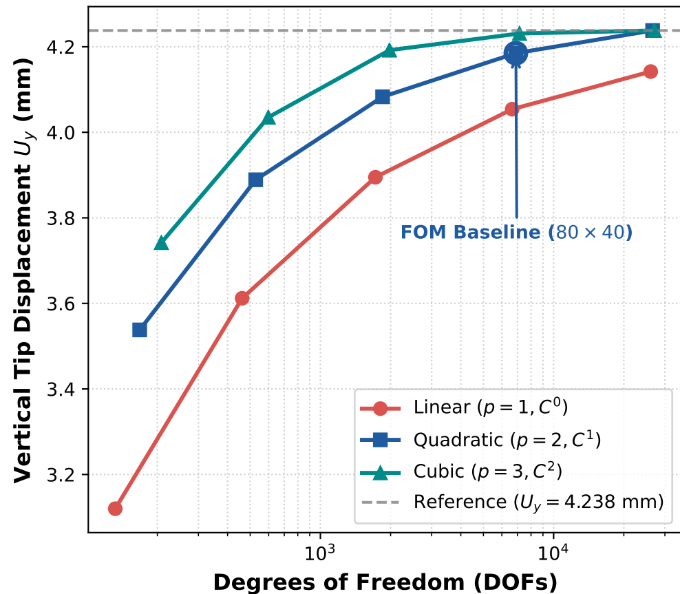
(a) Displacement Convergence under Static Load
