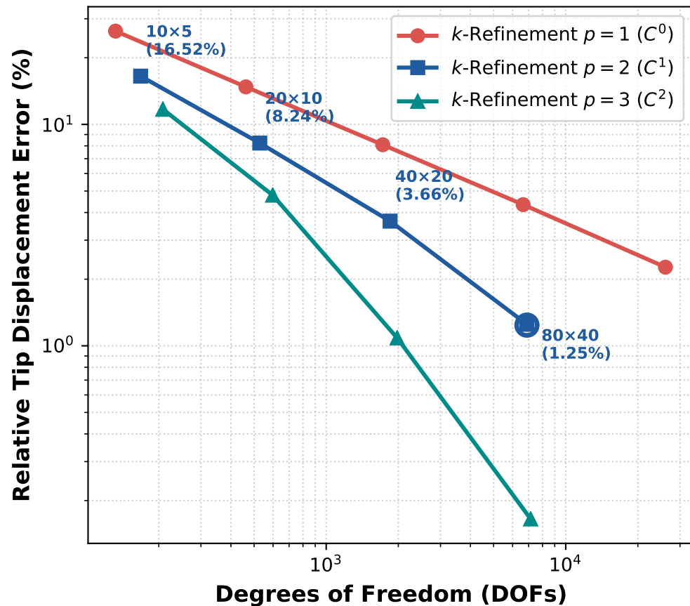
(b) Error Convergence across Refinement Orders ( k -Refinement)
