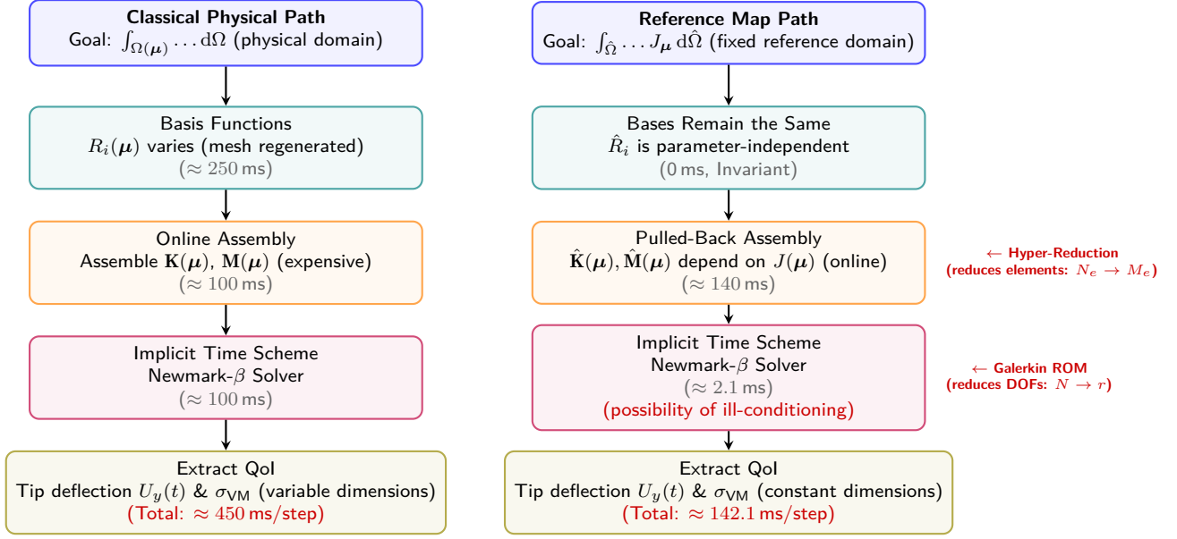
Figure 5.1: Visual workflow comparing physical-domain mesh regeneration (Classical) against reference-configuration pullback mapping, illustrating that online stiffness matrix assembly remains a computational bottleneck prior to model reduction.
