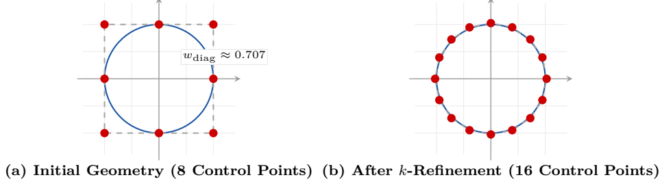
Figure 3.7: k -refinement (order elevation) schema demonstrating exact circle CAD geometry preservation with increased control point density and maximum inter-element continuity C^{p-1} .
