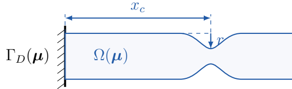
Figure 2.1: Schematic of the parameterized notched cantilever beam configuration \Omega(\boldsymbol{\mu}) showing Dirichlet boundary support \Gamma_D(\boldsymbol{\mu}) , notch location x_c , and notch depth r .
