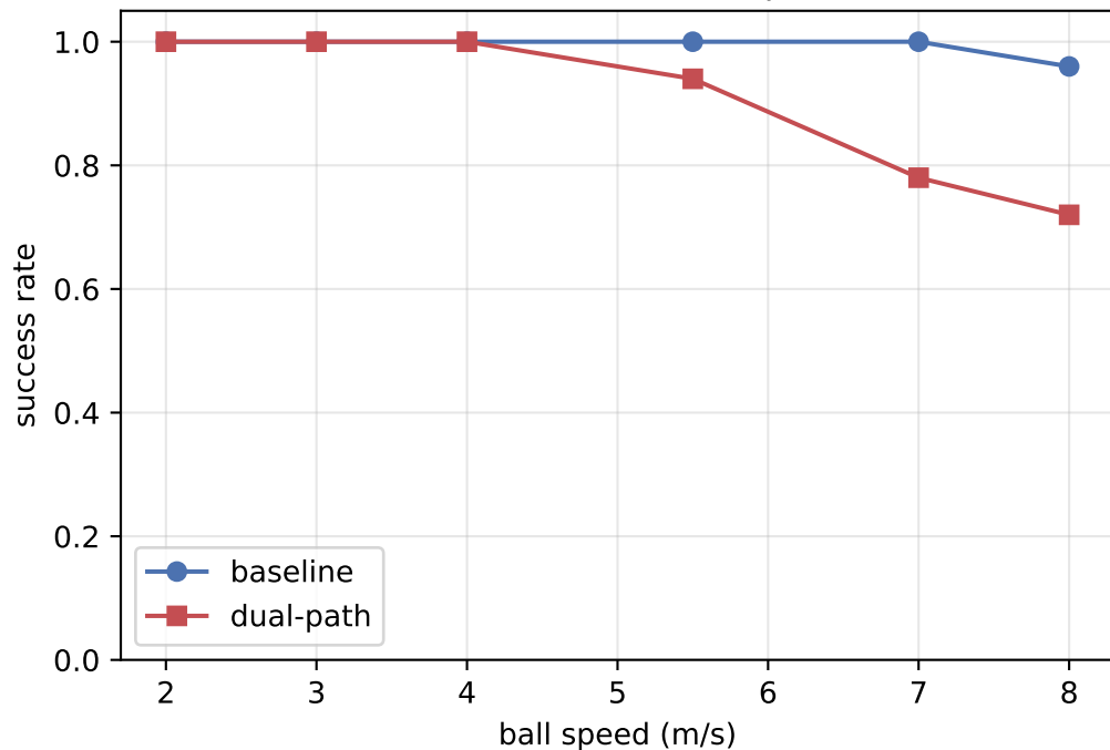
Success rate vs ball speed
