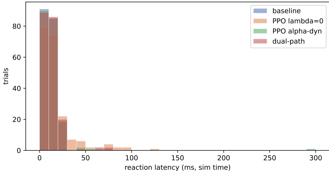
Reaction latency profile (stim -> first valid action)
