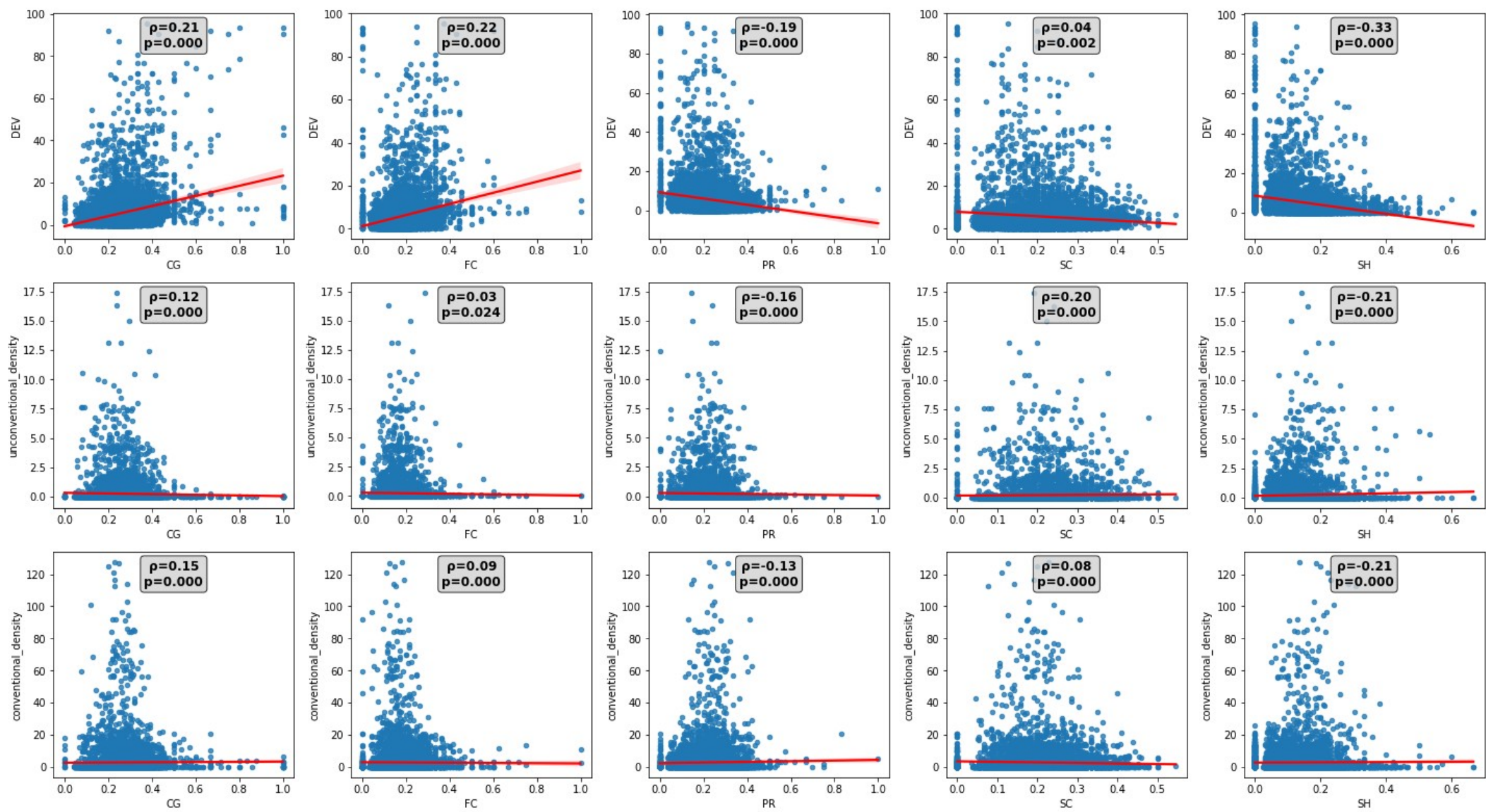
predictors (DLC, UOGD and COGD) vs predictands (functional metrics)
