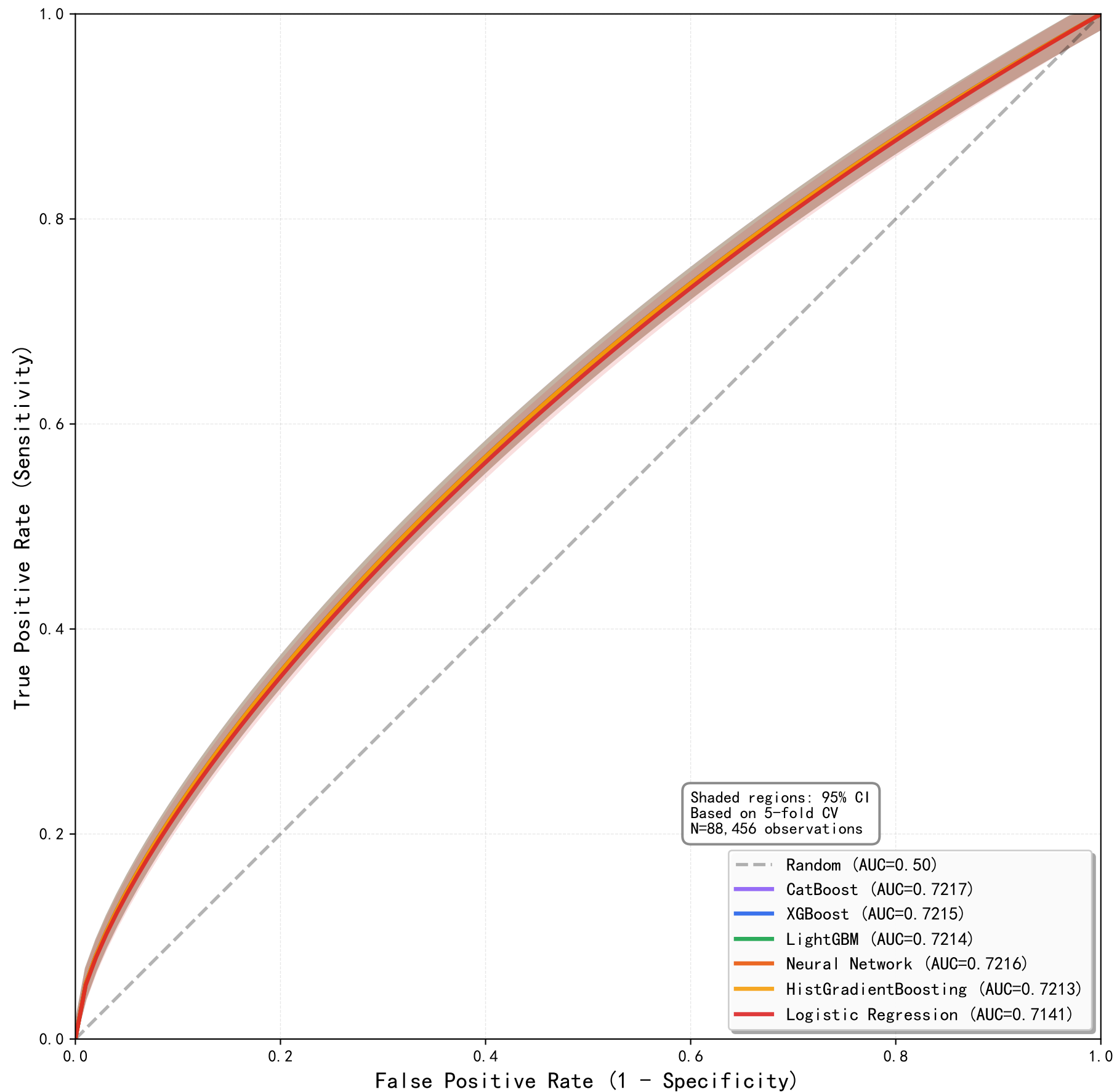
Figure 2: ROC Curves Comparing Six Machine Learning Models Predicting Healthy Aging from Digital-Social Connectedness
