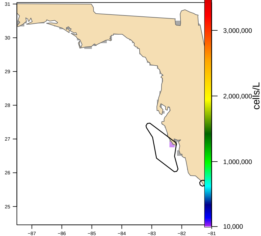
Hull-clipped (2 footprint(s), 8,360 km2) bloom area 229 km2
