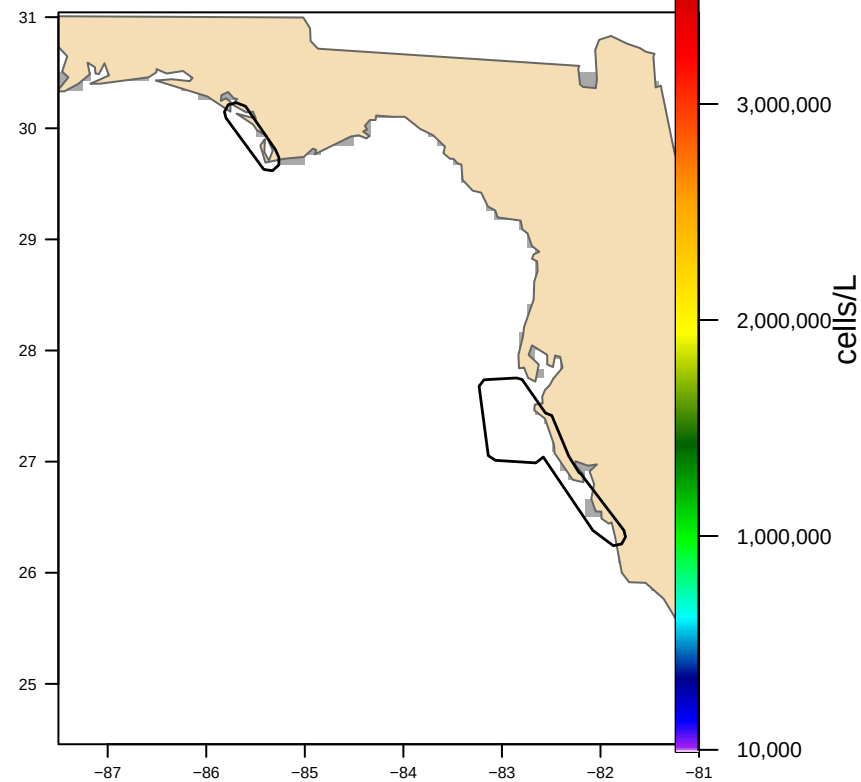
Hull-clipped (2 footprint(s), 9,486 km 2 ) bloom area 0 km 2
