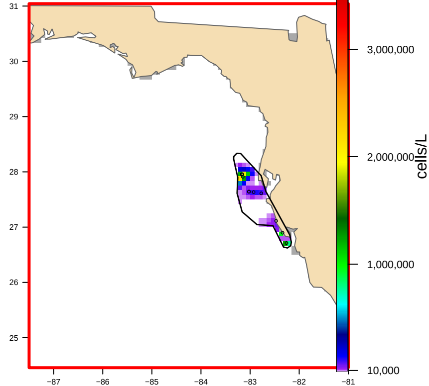
USED: Hull-clipped (1 footprint(s), 8,449 km 2 ) bloom area 4,702 km 2
