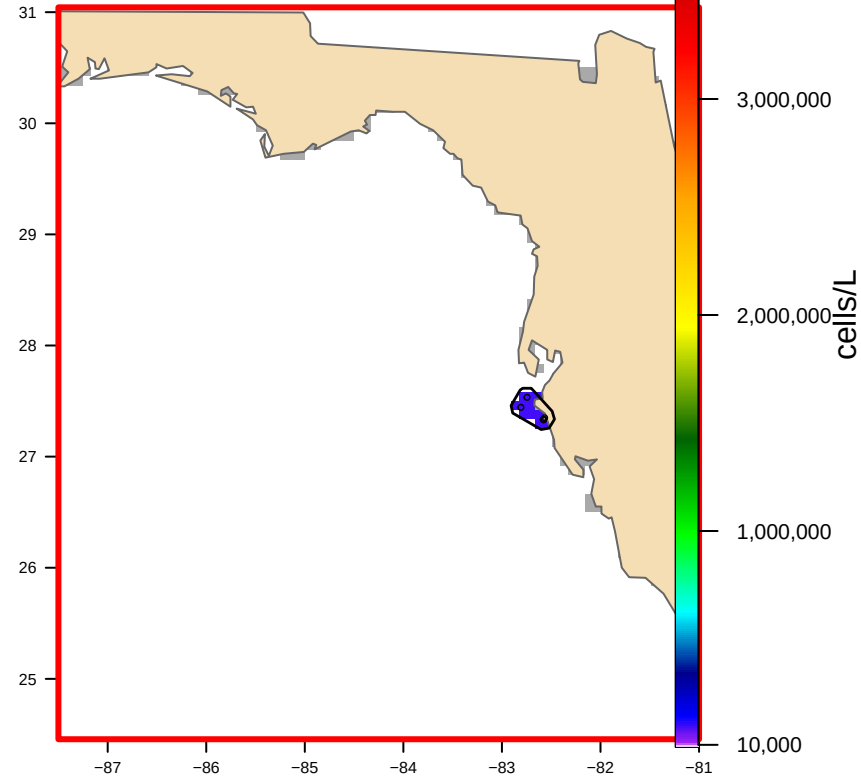
USED: Hull-clipped (1 footprint(s), 1,161 km2) bloom area 835 km2
