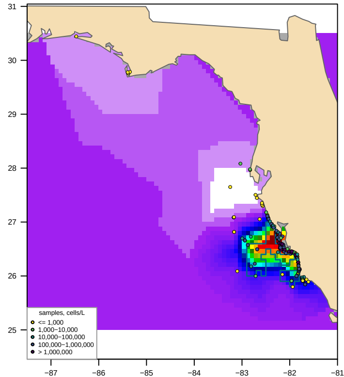
Unclipped sdmTMB (fitted, converged = TRUE) bloom area 284,236 km 2 , max 4,995,715 cells/L
