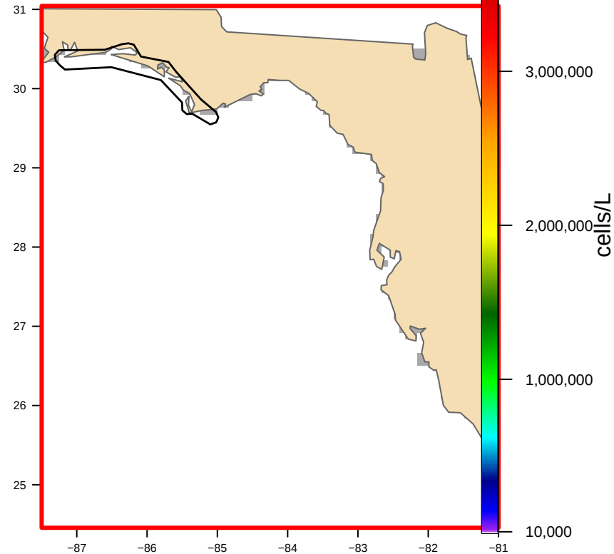
USED: Hull-clipped (1 footprint(s), 6,632 km 2 ) bloom area 0 km 2
