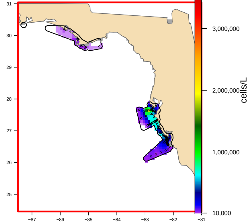
USED: Hull-clipped (3 footprint(s), 18,347 km 2 ) bloom area 13,690 km 2
