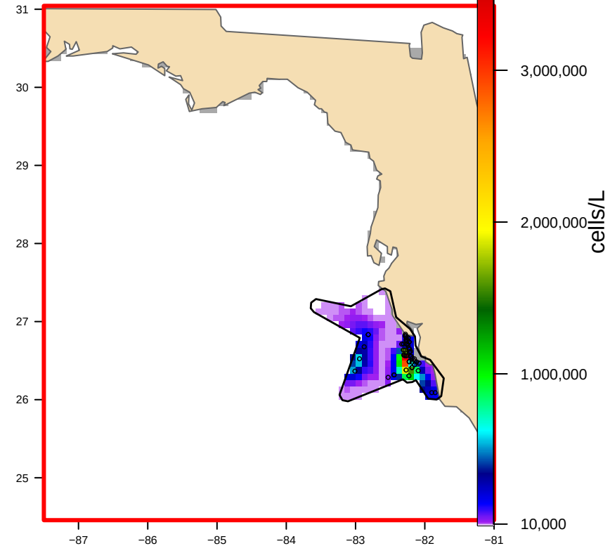
USED: Hull-clipped (1 footprint(s), 14,616 km 2 ) bloom area 12,694 km 2
