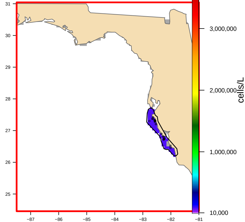
USED: Hull-clipped (1 footprint(s), 5,250 km 2 ) bloom area 3,812 km 2
