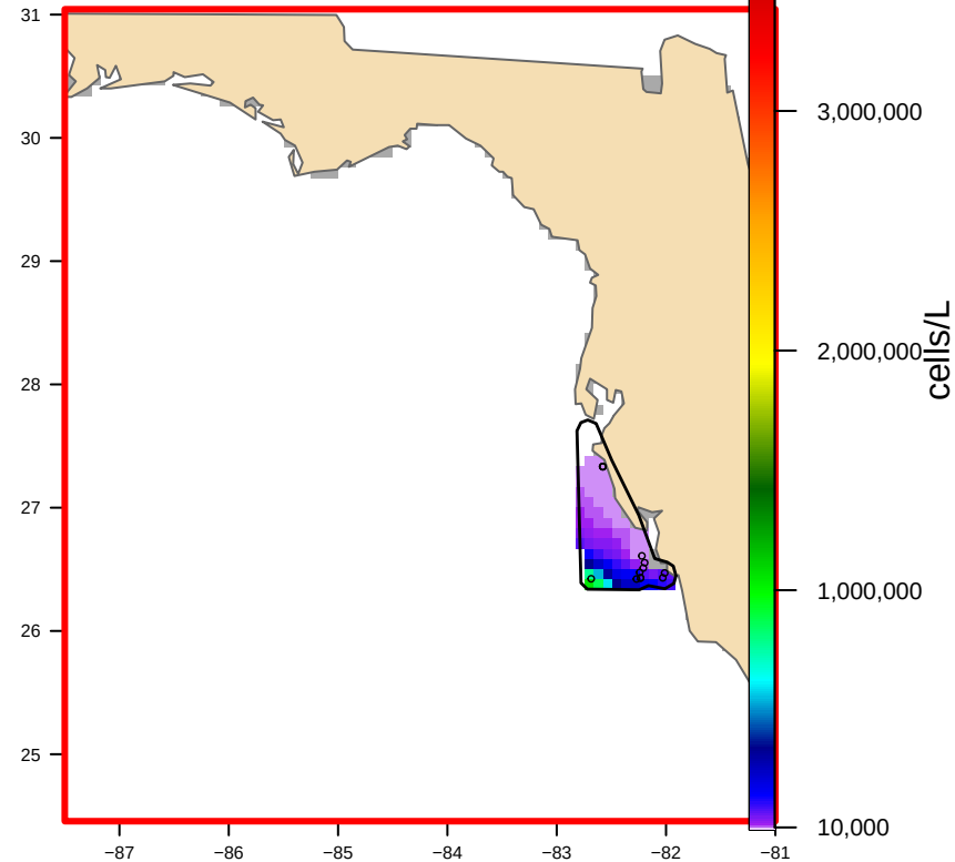
USED: Hull-clipped (1 footprint(s), 7,636 km 2 ) bloom area 6,110 km 2
