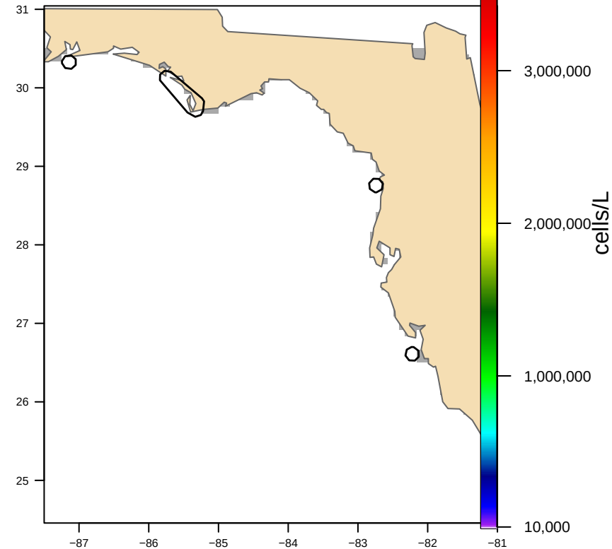
Hull-clipped (4 footprint(s), 2,788 km 2 ) bloom area 0 km 2
