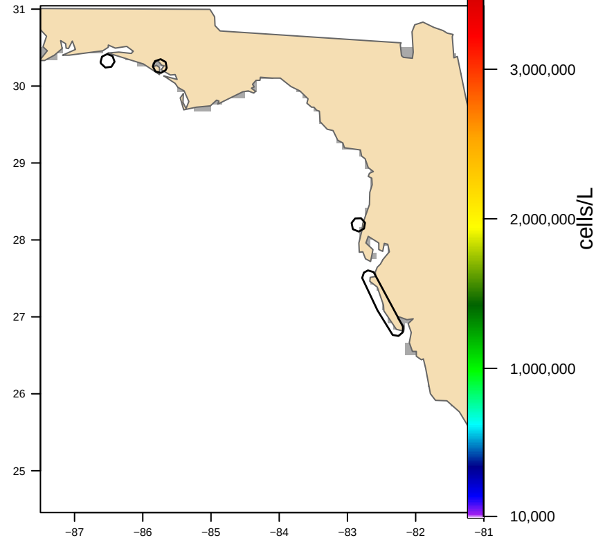
Hull-clipped (4 footprint(s), 3,013 km2) bloom area 0 km2
