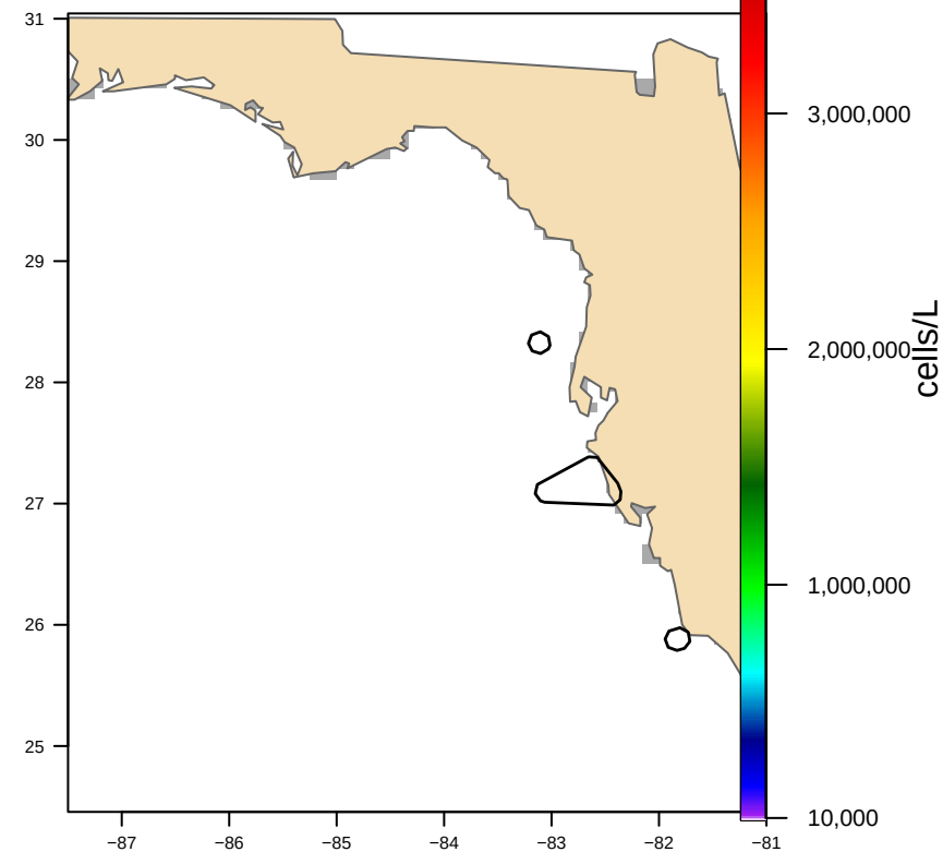
Hull-clipped (3 footprint(s), 3,141 km2) bloom area 0 km2
