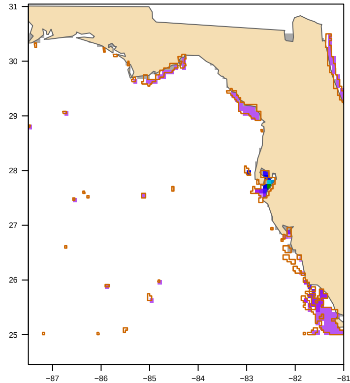
MODIS nFLH-clipped (47 polygon(s)) bloom area 9,106 km 2
