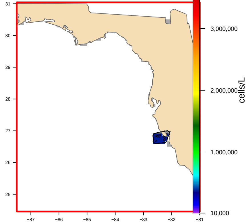
USED: Hull-clipped (1 footprint(s), 2,051 km 2 ) bloom area 1,680 km 2
