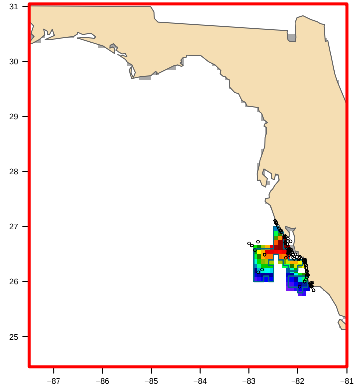
USED: VIIRS-clipped (49 positive VIIRS cells) bloom area 7,744 km 2
