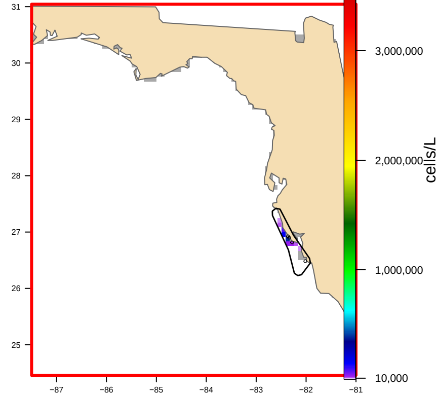
USED: Hull-clipped (1 footprint(s), 3,431 km2) bloom area 686 km2
