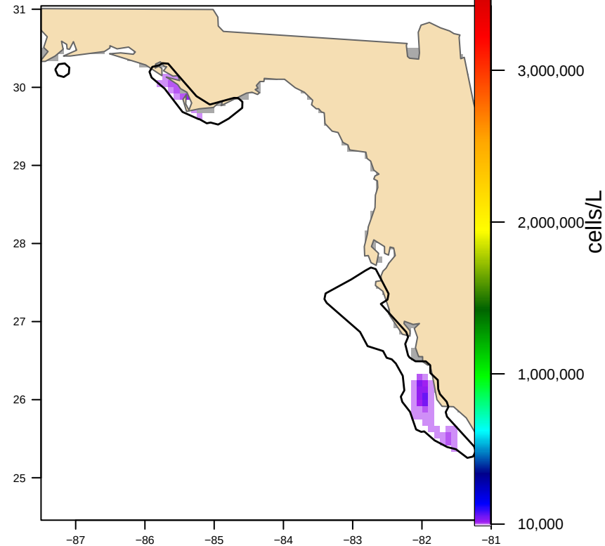
Hull-clipped (3 footprint(s), 19,084 km 2 ) bloom area 4,116 km 2
