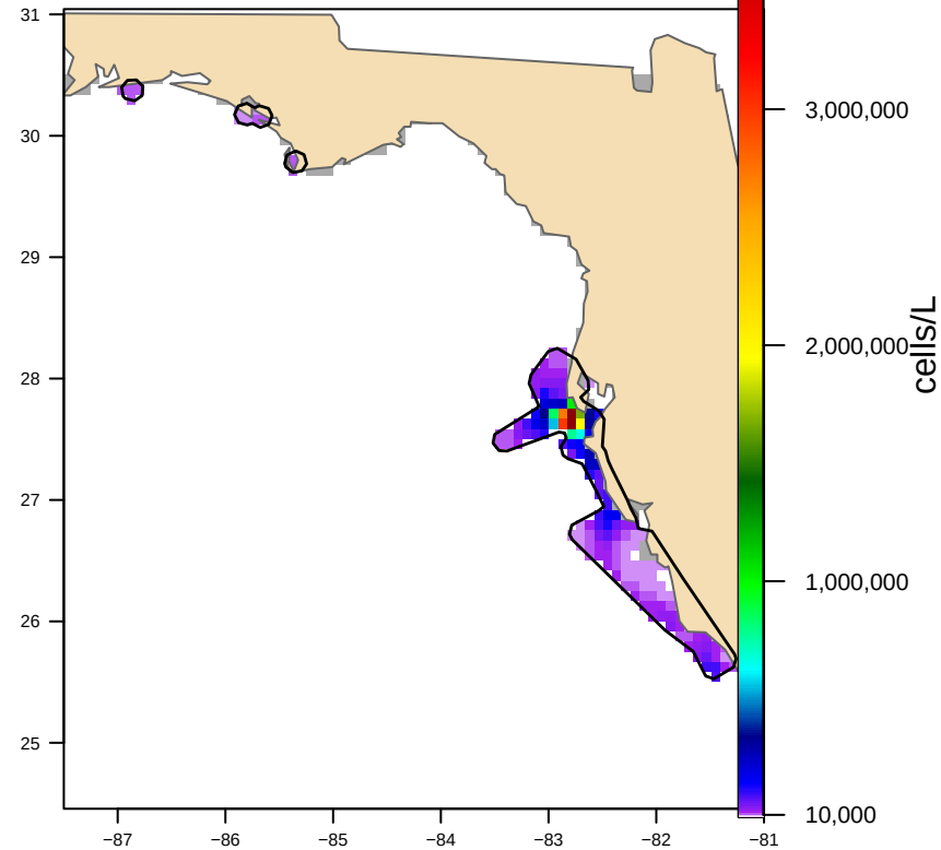
Hull-clipped (4 footprint(s), 16,363 km 2 ) bloom area 12,403 km 2
