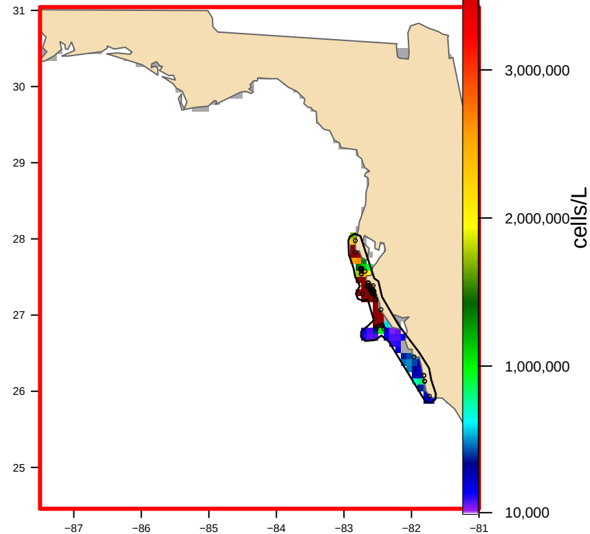
USED: Hull-clipped (2 footprint(s), 8,023 km 2 ) bloom area 5,494 km 2
