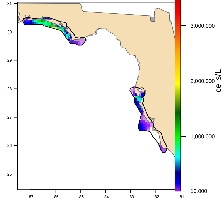
Hull-clipped (2 footprint(s), 17,656 km 2 ) bloom area 11,187 km 2
