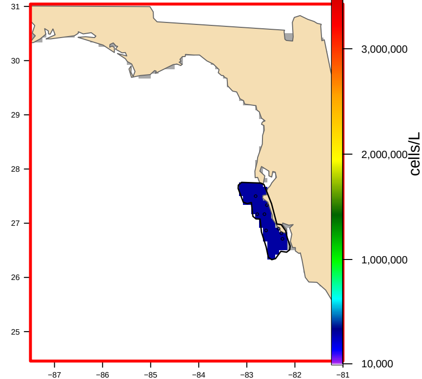
USED: Hull-clipped (1 footprint(s), 7,198 km 2 ) bloom area 6,396 km 2
