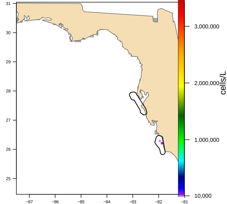
Hull-clipped (2 footprint(s), 4,057 km 2 ) bloom area 153 km 2
