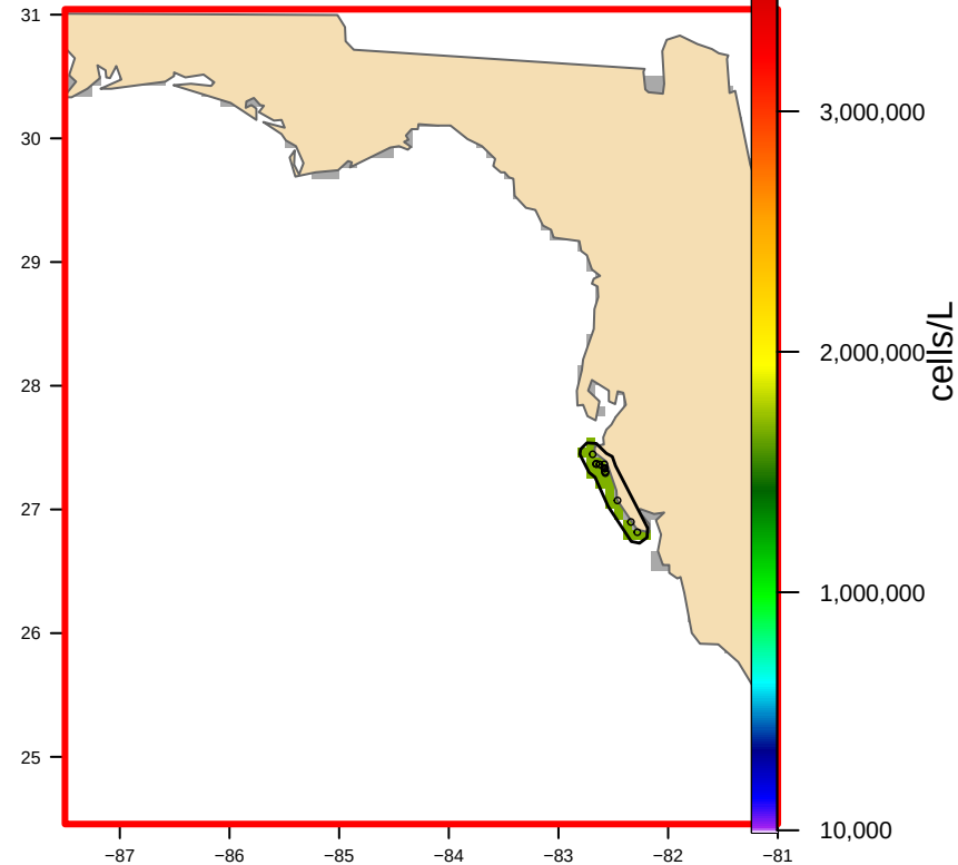
USED: Hull-clipped (1 footprint(s), 2,109 km 2 ) bloom area 1,370 km 2
