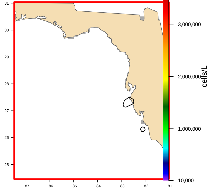
USED: Hull-clipped (2 footprint(s), 1,558 km2) bloom area 0 km2
