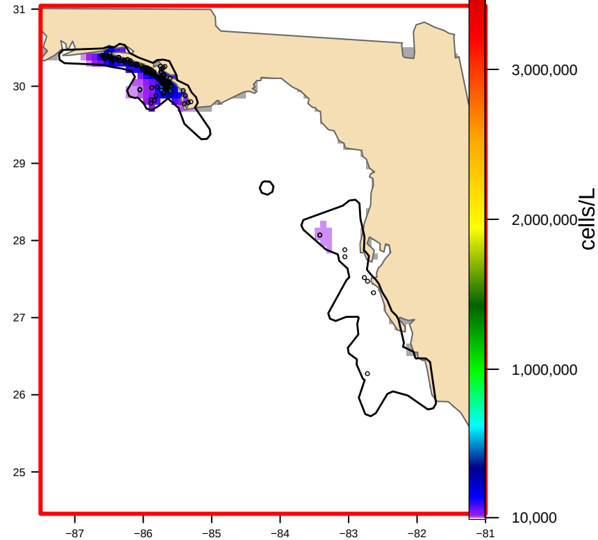
USED: Hull-clipped (3 footprint(s), 30,157 km 2 ) bloom area 6,159 km 2
