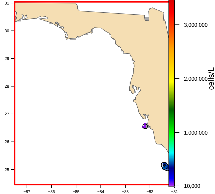
USED: Hull-clipped (2 footprint(s), 1,294 km2) bloom area 1,004 km2
