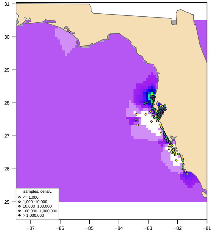
Unclipped sdmTMB (fitted, converged = TRUE) bloom area 285,799 km 2 , max 2,020,226 cells/L
