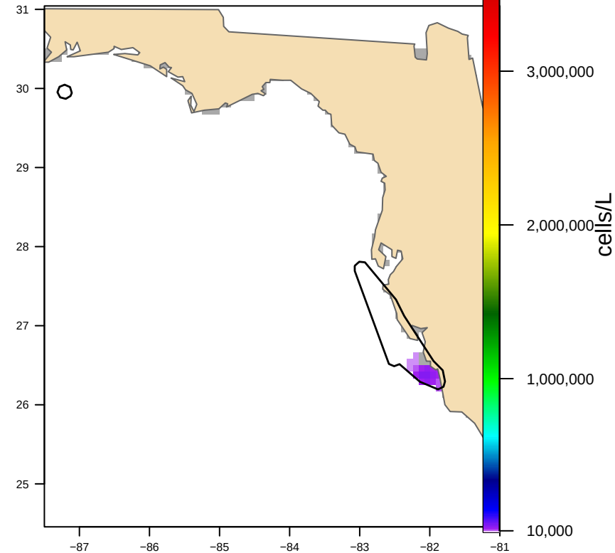
Hull-clipped (2 footprint(s), 8,244 km2) bloom area 1,456 km2
