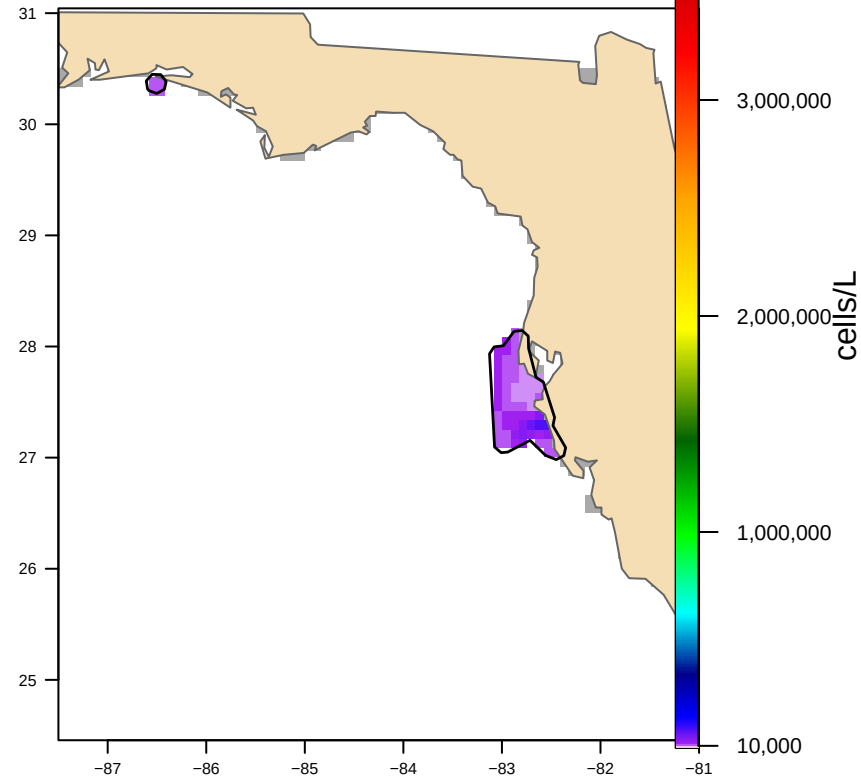
Hull-clipped (2 footprint(s), 6,408 km 2 ) bloom area 5,151 km 2
