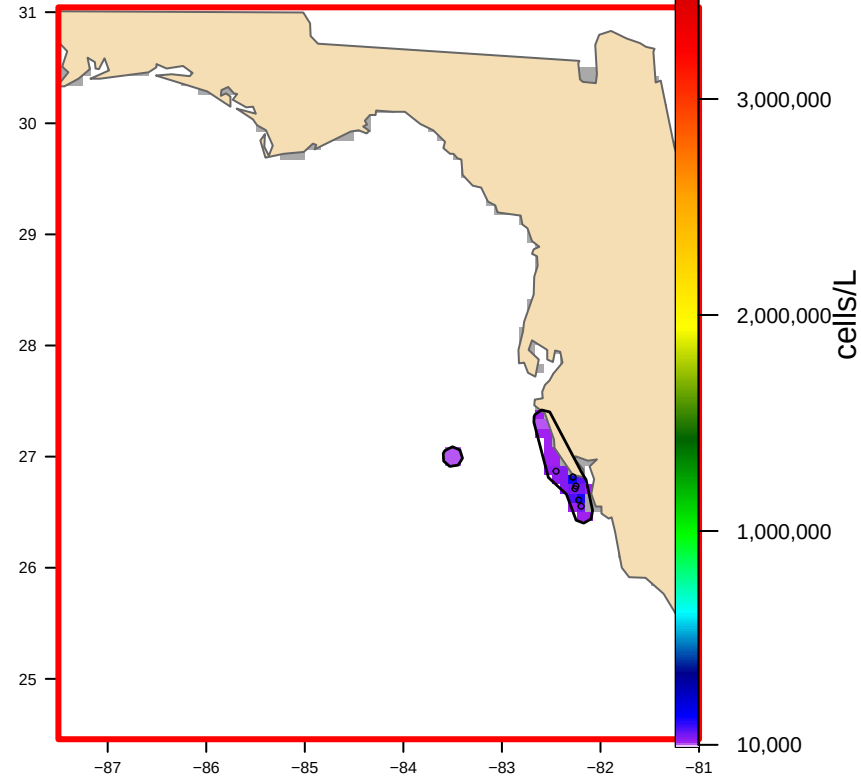
USED: Hull-clipped (2 footprint(s), 3,237 km2) bloom area 2,365 km2
