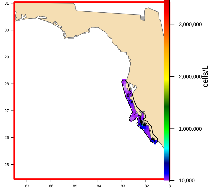
USED: Hull-clipped (1 footprint(s), 9,102 km 2 ) bloom area 6,408 km 2
