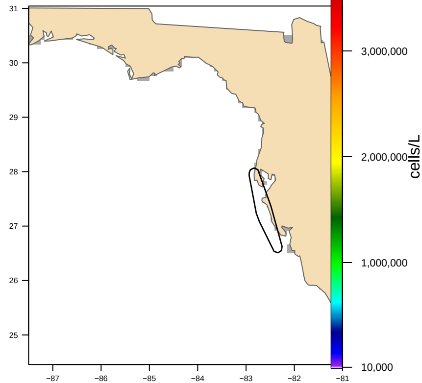
Hull-clipped (1 footprint(s), 4,659 km2) bloom area 0 km2
