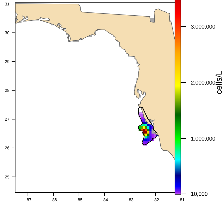
Hull-clipped (1 footprint(s), 5,330 km 2 ) bloom area 4,130 km 2
