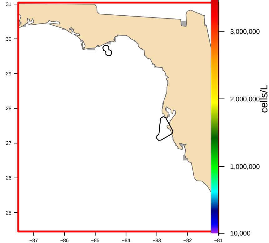
USED: Hull-clipped (2 footprint(s), 2,958 km2) bloom area 0 km2
