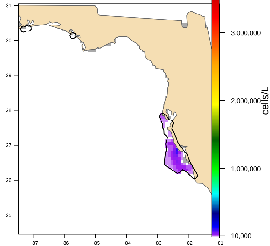
Hull-clipped (3 footprint(s), 10,452 km 2 ) bloom area 6,417 km 2
