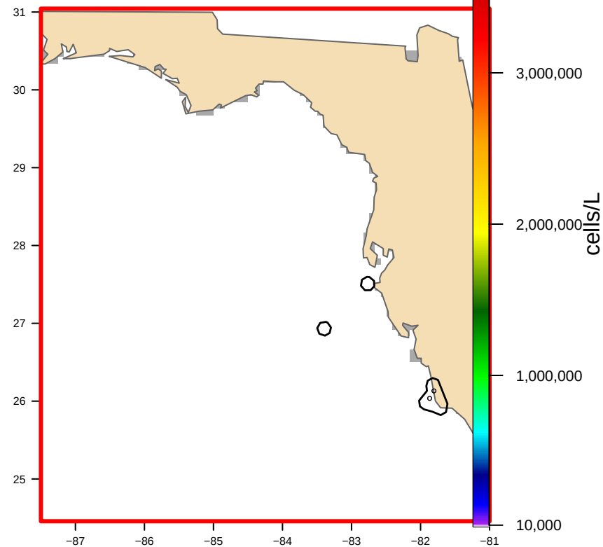
USED: Hull-clipped (3 footprint(s), 2,046 km2) bloom area 0 km2
