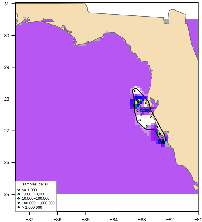
Unclipped sdmTMB (fitted, converged = TRUE) bloom area 288,327 km 2 , max 2,129,701 cells/L
