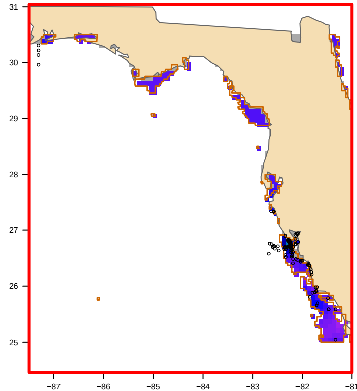
USED: MODIS nFLH-clipped (30 polygon(s)) bloom area 13,049 km 2
