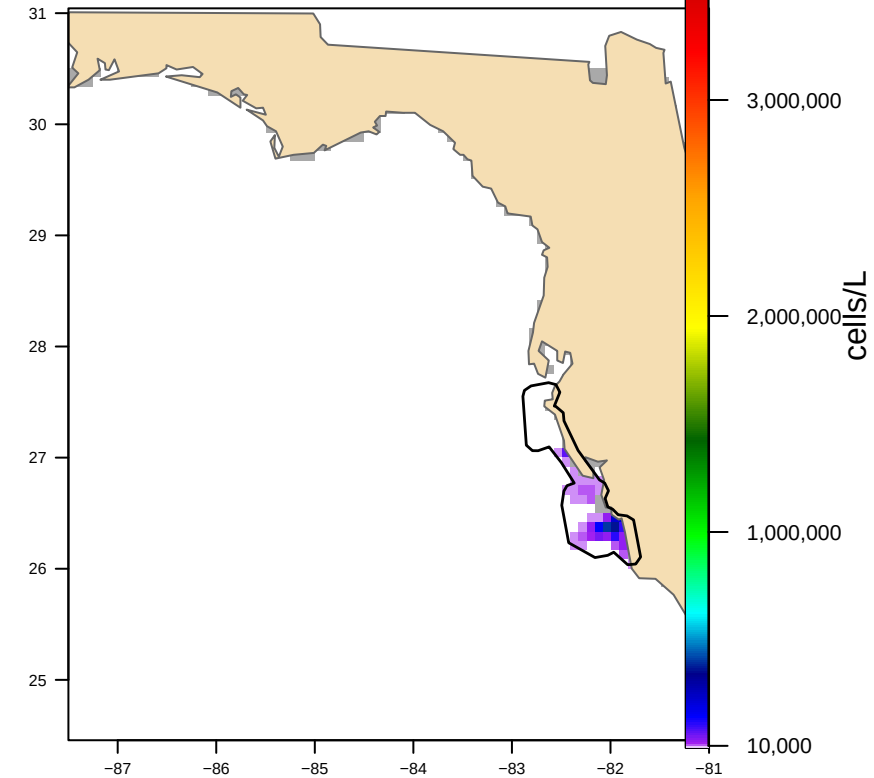
Hull-clipped (1 footprint(s), 7,835 km 2 ) bloom area 3,062 km 2
