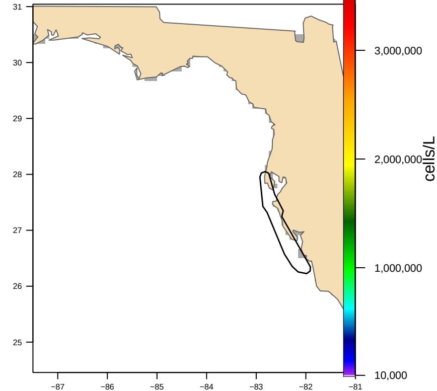
Hull-clipped (1 footprint(s), 6,058 km 2 ) bloom area 0 km 2
