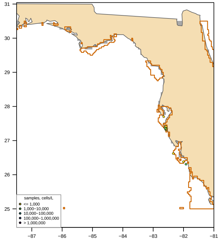
Unclipped sdmTMB (fitted, converged = TRUE) bloom area 0 km 2 , max 2,054 cells/L
