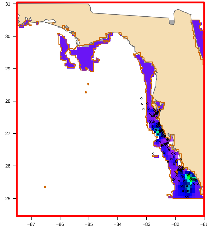
USED: MODIS nFLH-clipped (25 polygon(s)) bloom area 35,649 km 2
