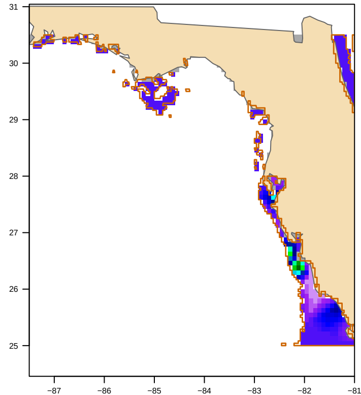
MODIS nFLH-clipped (37 polygon(s)) bloom area 22,096 km 2
