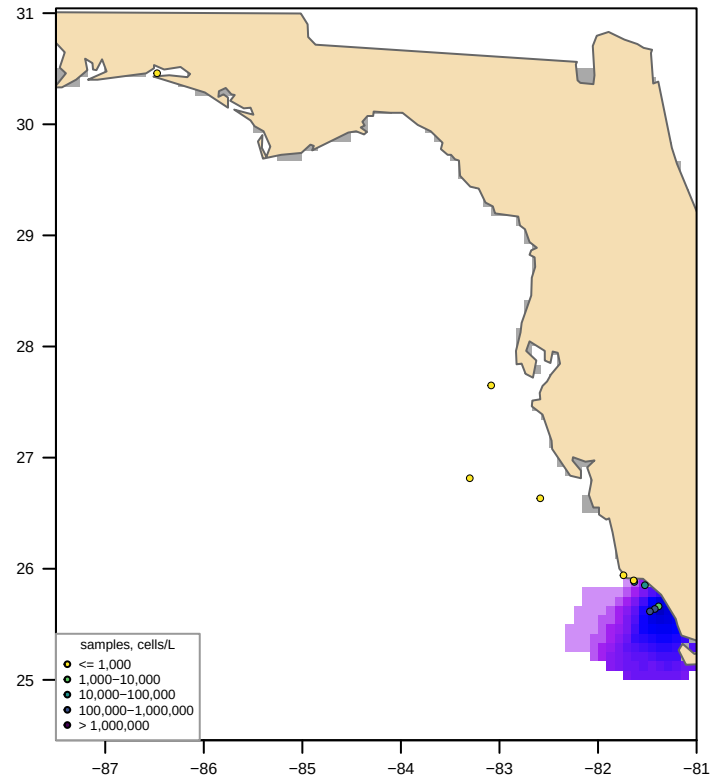
Unclipped sdmTMB (fitted, converged = TRUE) bloom area 9,578 km 2 , max 259,872 cells/L
