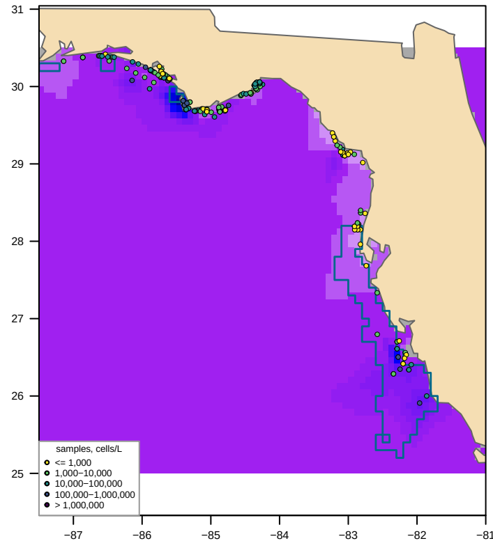
Unclipped sdmTMB (fitted, converged = TRUE) bloom area 291,361 km 2 , max 336,253 cells/L
