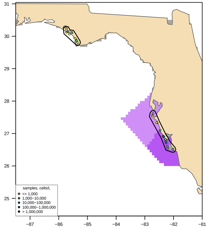
Unclipped sdmTMB (fitted, converged = TRUE) bloom area 20,417 km 2 , max 23,735 cells/L
