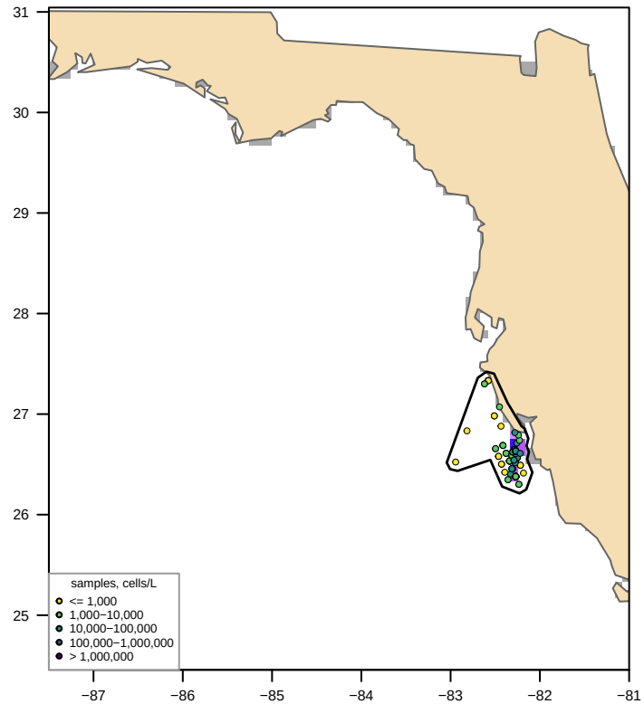
Unclipped sdmTMB (fitted, converged = TRUE) bloom area 612 km 2 , max 106,180 cells/L
