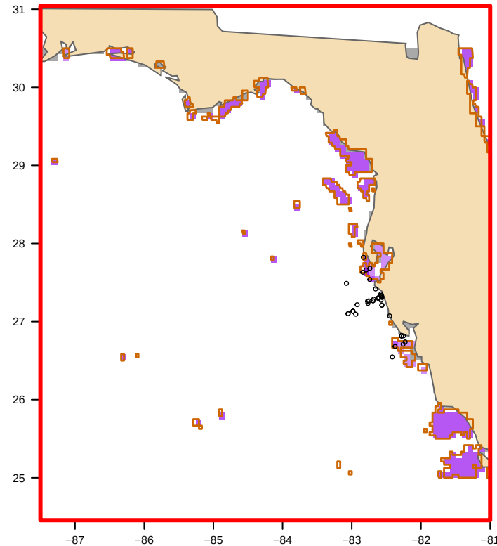
USED: MODIS nFLH-clipped (49 polygon(s)) bloom area 11,509 km 2
