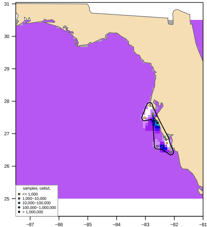
Unclipped sdmTMB (fitted, converged = TRUE) bloom area 290,221 km2, max 820,865 cells/L
