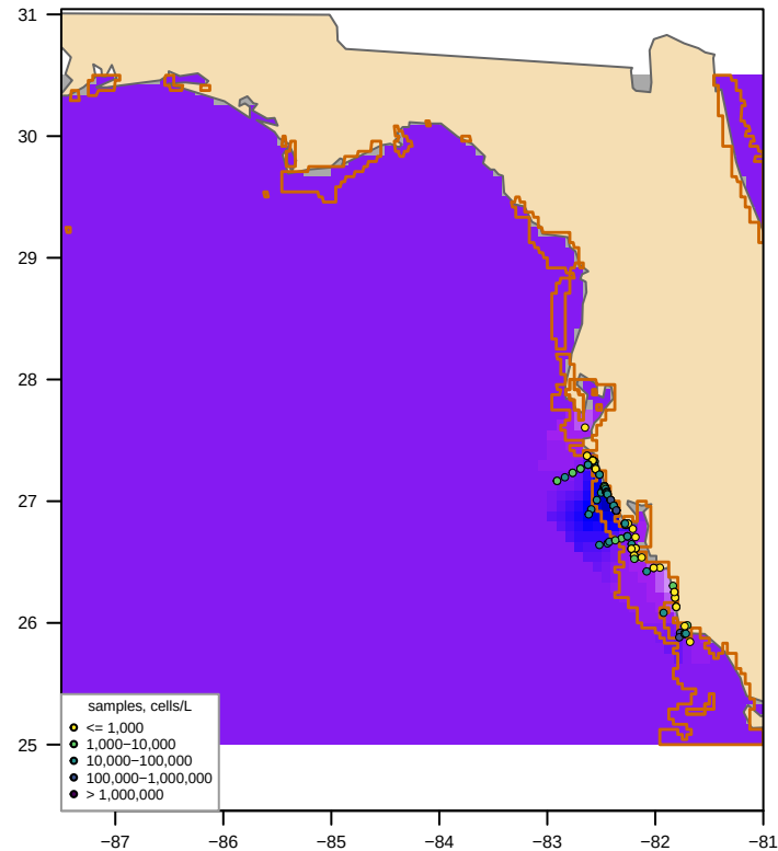
Unclipped sdmTMB (fitted, converged = TRUE) bloom area 291,361 km 2 , max 268,823 cells/L
