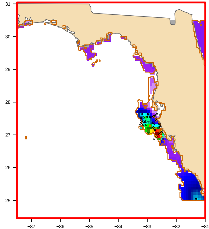
USED: MODIS nFLH-clipped (33 polygon(s)) bloom area 25,542 km 2
