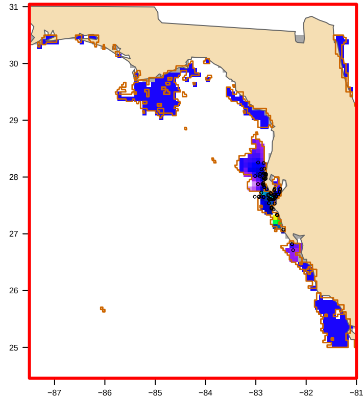
USED: MODIS nFLH-clipped (47 polygon(s)) bloom area 22,694 km 2
