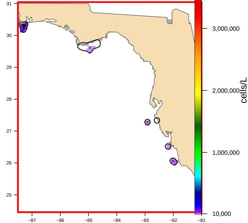
USED: Hull-clipped (6 footprint(s), 4,450 km 2 ) bloom area 2,181 km 2
