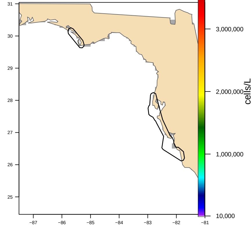
Hull-clipped (2 footprint(s), 9,697 km 2 ) bloom area 0 km 2
