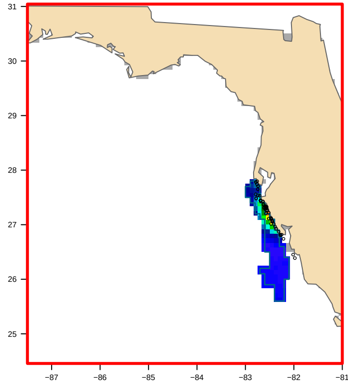
USED: VIIRS-clipped (64 positive VIIRS cells) bloom area 9,253 km 2
