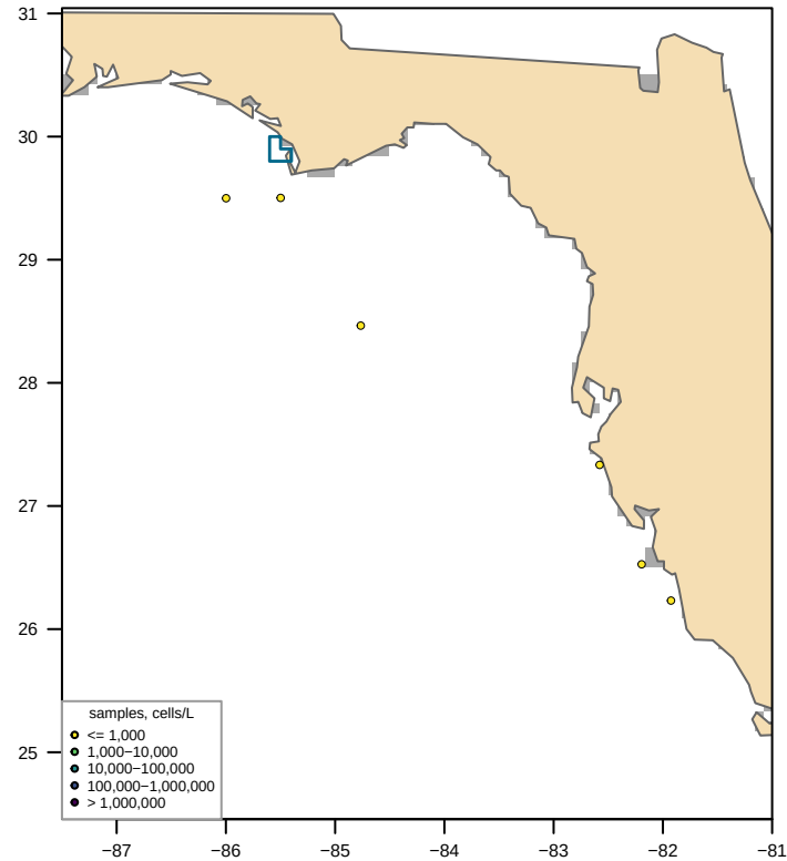
Unclipped sdmTMB (fitted, converged = TRUE) bloom area 0 km2, max 360 cells/L
