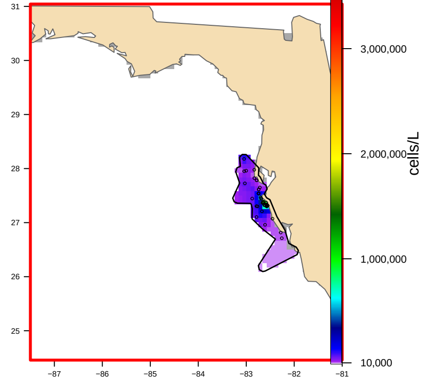
USED: Hull-clipped (1 footprint(s), 11,204 km 2 ) bloom area 9,967 km 2
