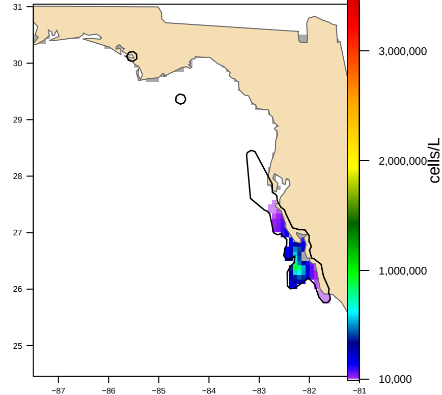
Hull-clipped (3 footprint(s), 13,559 km 2 ) bloom area 6,349 km 2
