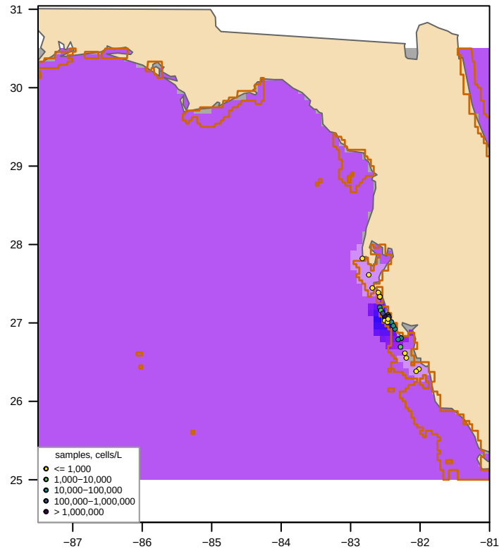
Unclipped sdmTMB (fitted, converged = TRUE) bloom area 291,361 km 2 , max 147,435 cells/L
