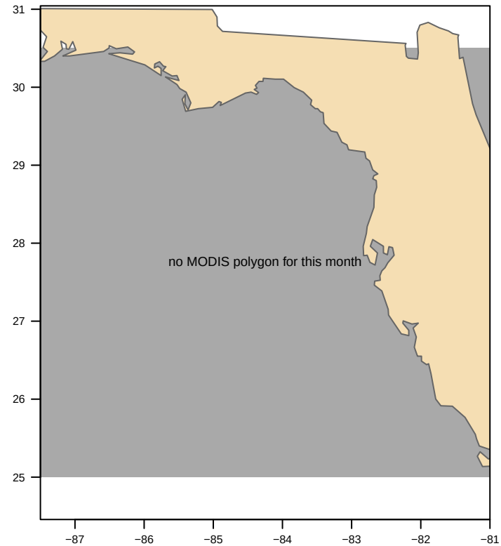
MODIS nFLH-clipped
