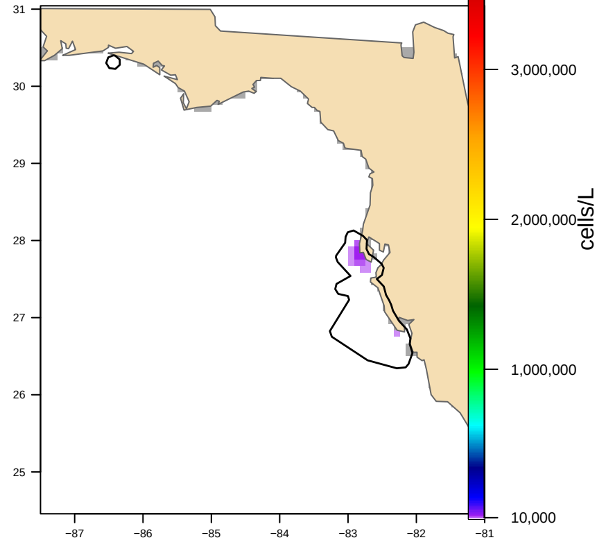
Hull-clipped (2 footprint(s), 13,394 km 2 ) bloom area 985 km 2
