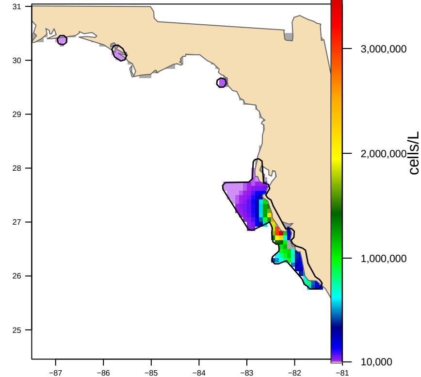
Hull-clipped (4 footprint(s), 15,754 km 2 ) bloom area 12,918 km 2
