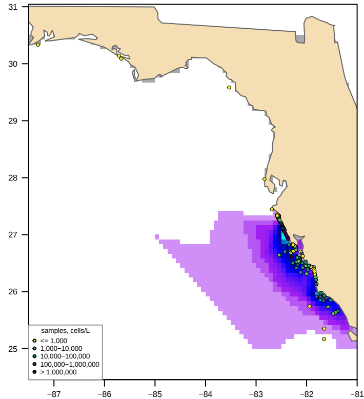
Unclipped sdmTMB (fitted, converged = TRUE) bloom area 55,038 km 2 , max 763,526 cells/L
