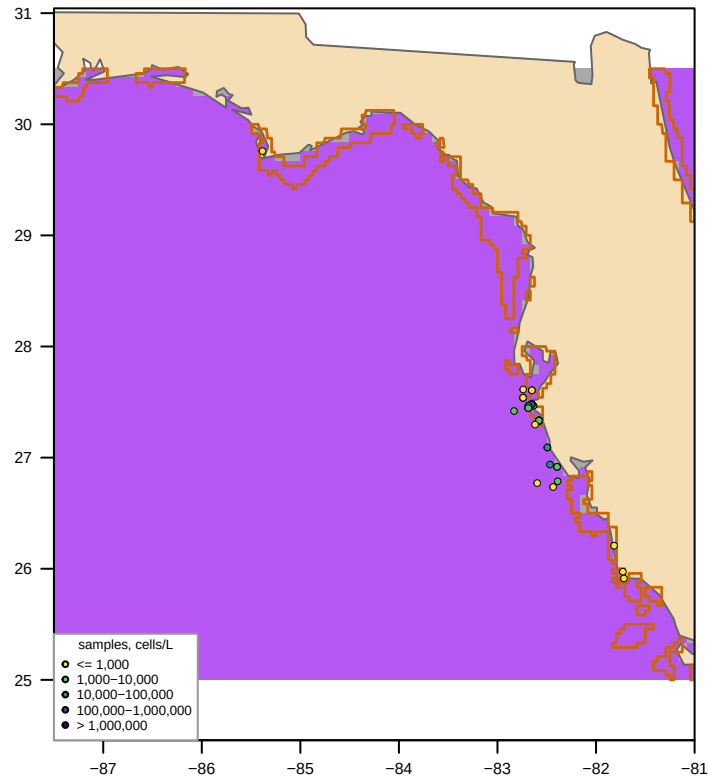
Unclipped sdmTMB (fitted, converged = TRUE) bloom area 291,361 km 2 , max 27,206 cells/L
