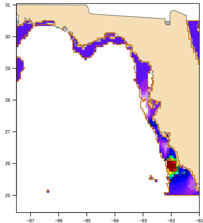
MODIS nFLH-clipped (20 polygon(s)) bloom area 37,458 km 2
