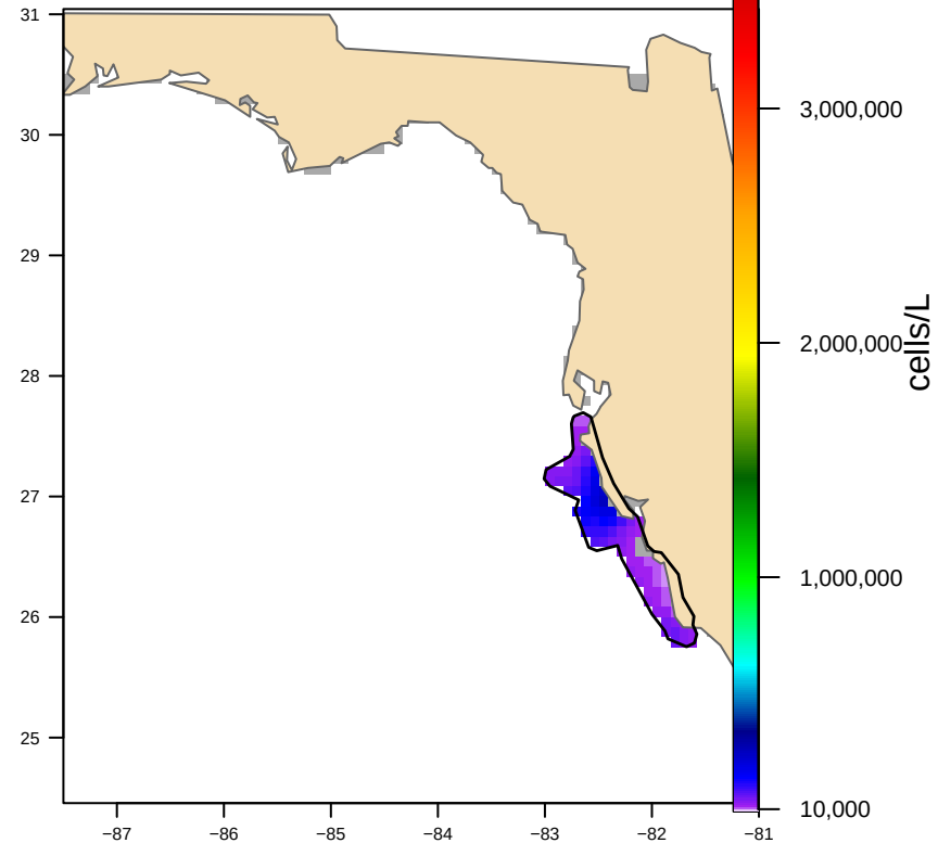
Hull-clipped (1 footprint(s), 8,700 km 2 ) bloom area 6,878 km 2
