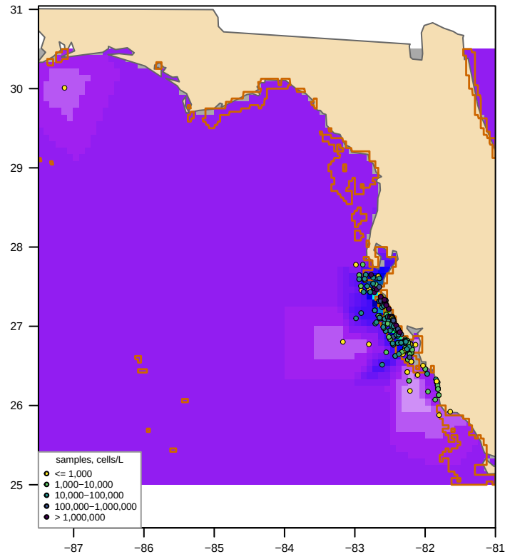
Unclipped sdmTMB (fitted, converged = TRUE) bloom area 291,361 km 2 , max 3,348,804 cells/L
