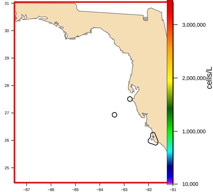
USED: Hull-clipped (3 footprint(s), 2,046 km2) bloom area 0 km2
