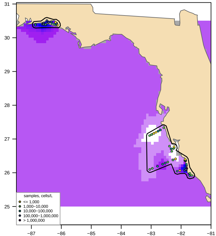
Unclipped sdmTMB (fitted, converged = TRUE) bloom area 287,473 km2, max 401,351 cells/L
