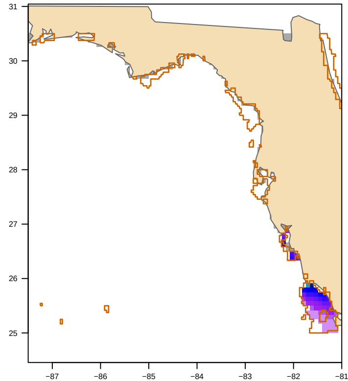
MODIS nFLH-clipped (36 polygon(s)) bloom area 5,322 km 2
