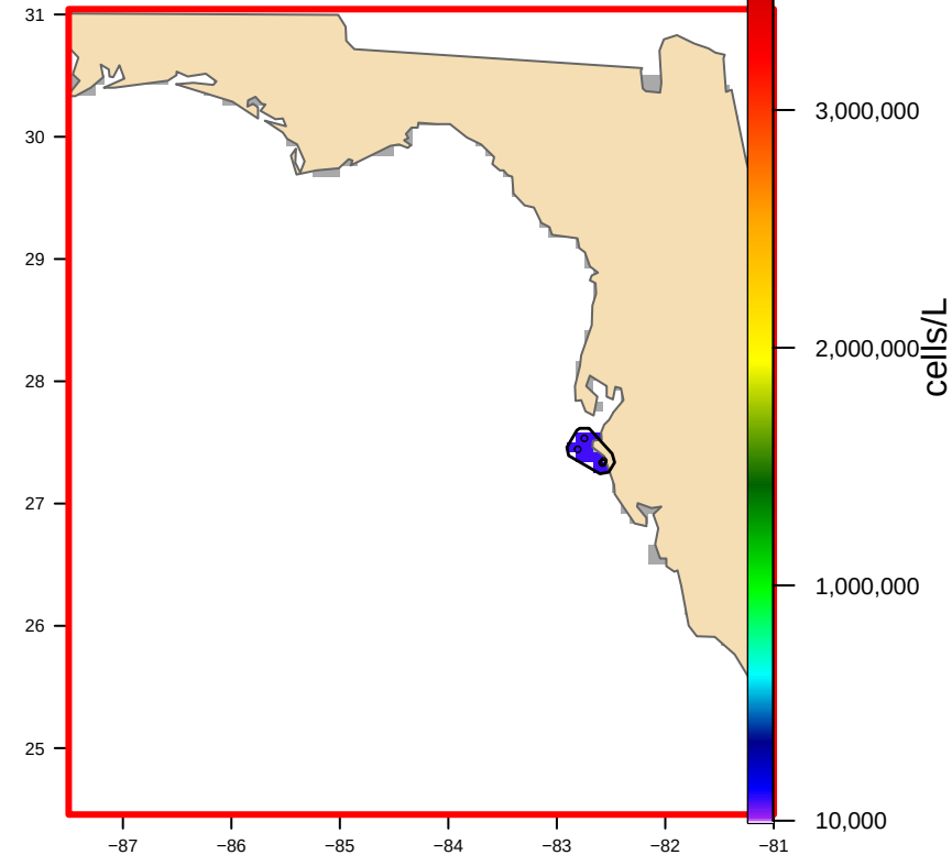
USED: Hull-clipped (1 footprint(s), 1,161 km2) bloom area 835 km2
