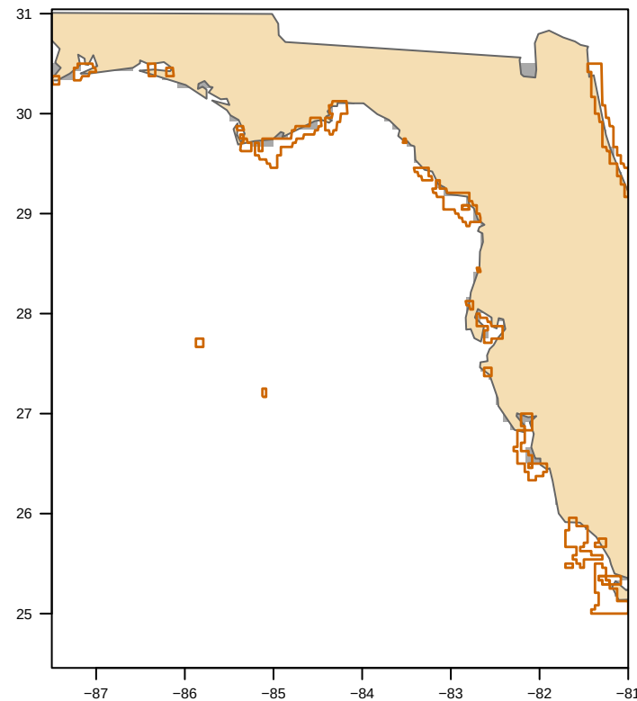
MODIS nFLH-clipped (29 polygon(s)) bloom area 0 km 2
