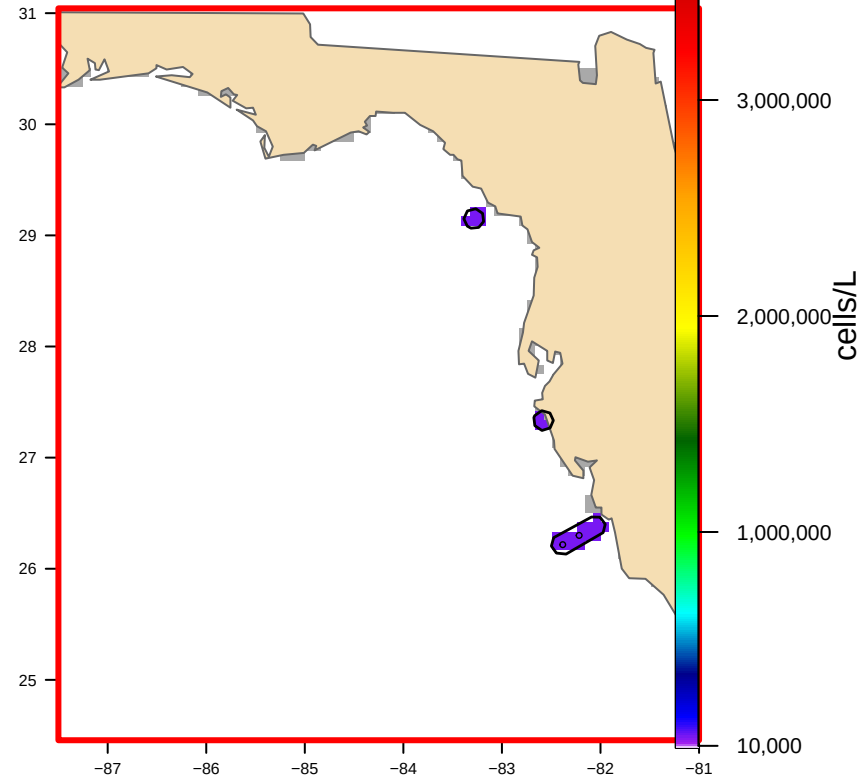
USED: Hull-clipped (3 footprint(s), 1,755 km 2 ) bloom area 1,752 km 2
