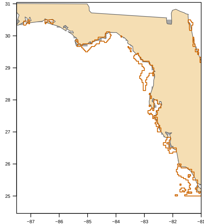
MODIS nFLH-clipped (31 polygon(s)) bloom area 0 km 2
