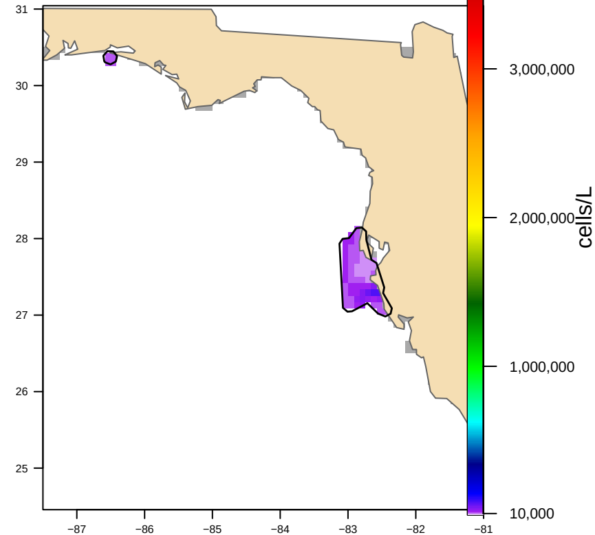
Hull-clipped (2 footprint(s), 6,408 km 2 ) bloom area 5,151 km 2
