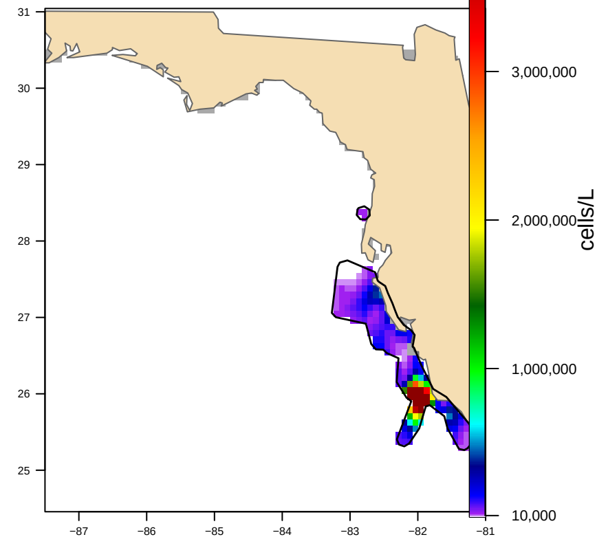
Hull-clipped (2 footprint(s), 16,220 km 2 ) bloom area 14,312 km 2
