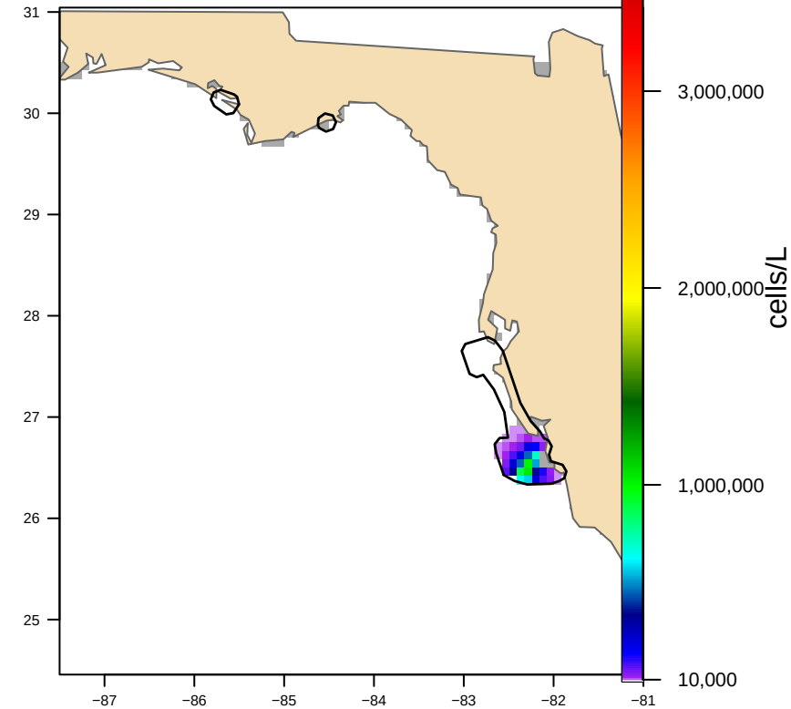
Hull-clipped (3 footprint(s), 7,598 km 2 ) bloom area 3,136 km 2
