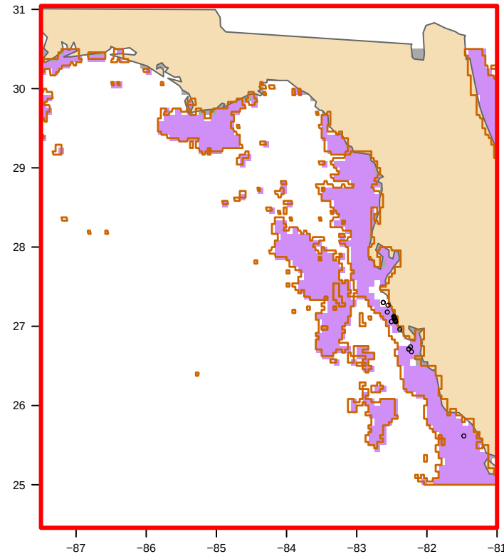
USED: MODIS nFLH-clipped (76 polygon(s)) bloom area 46,598 km 2
