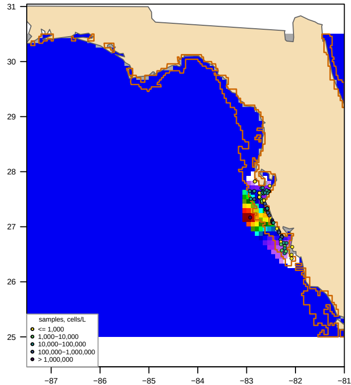
Unclipped sdmTMB (fitted, converged = TRUE) bloom area 290,293 km 2 , max 4,628,416 cells/L
