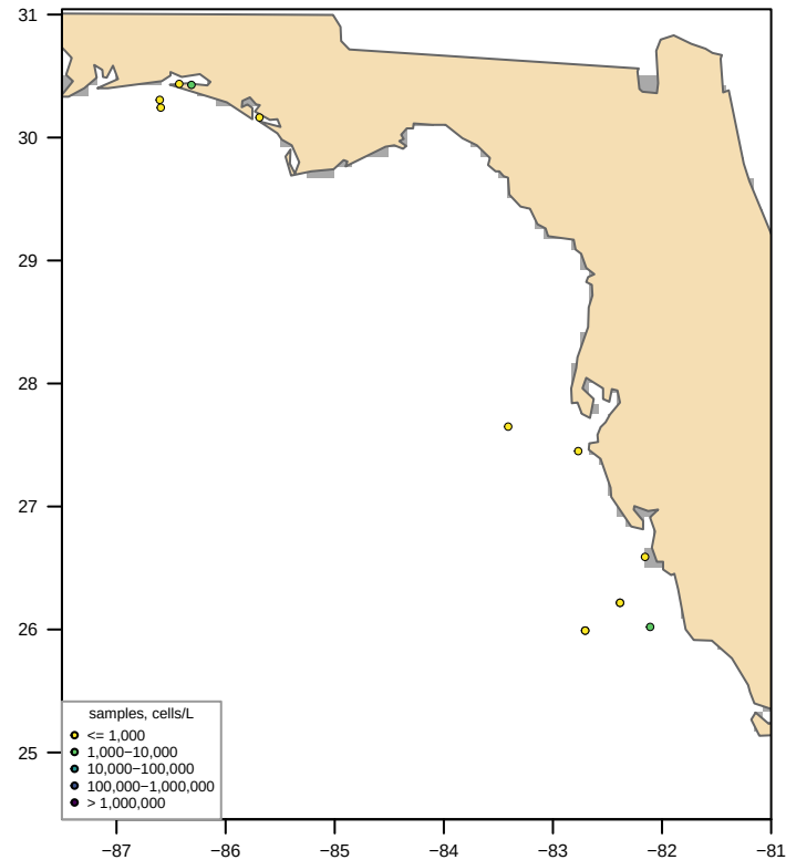
Unclipped sdmTMB (fitted, converged = TRUE) bloom area 0 km 2 , max 4,311 cells/L
