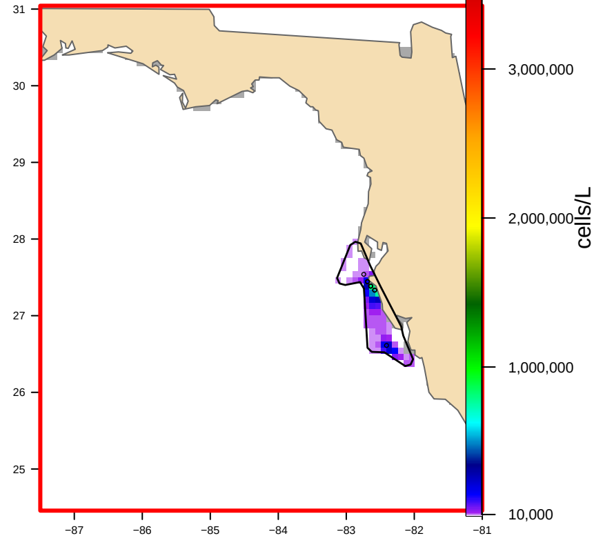
USED: Hull-clipped (1 footprint(s), 7,178 km2) bloom area 5,104 km2
