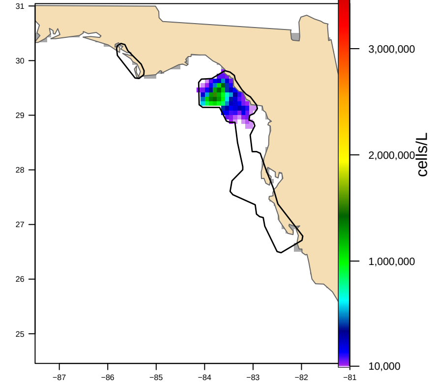
Hull-clipped (2 footprint(s), 23,558 km 2 ) bloom area 7,014 km 2
