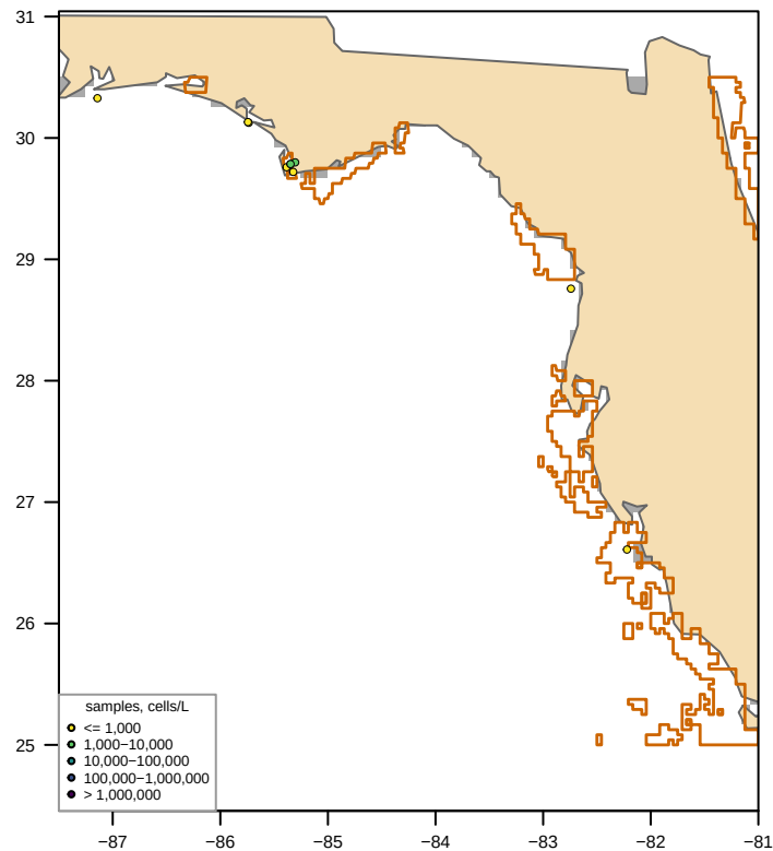
Unclipped sdmTMB (fitted, converged = TRUE) bloom area 0 km 2 , max 793 cells/L
