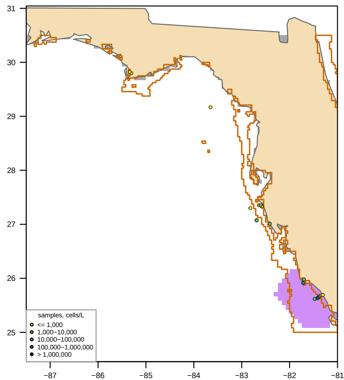
Unclipped sdmTMB (fitted, converged = TRUE) bloom area 9,027 km 2 , max 19,774 cells/L
