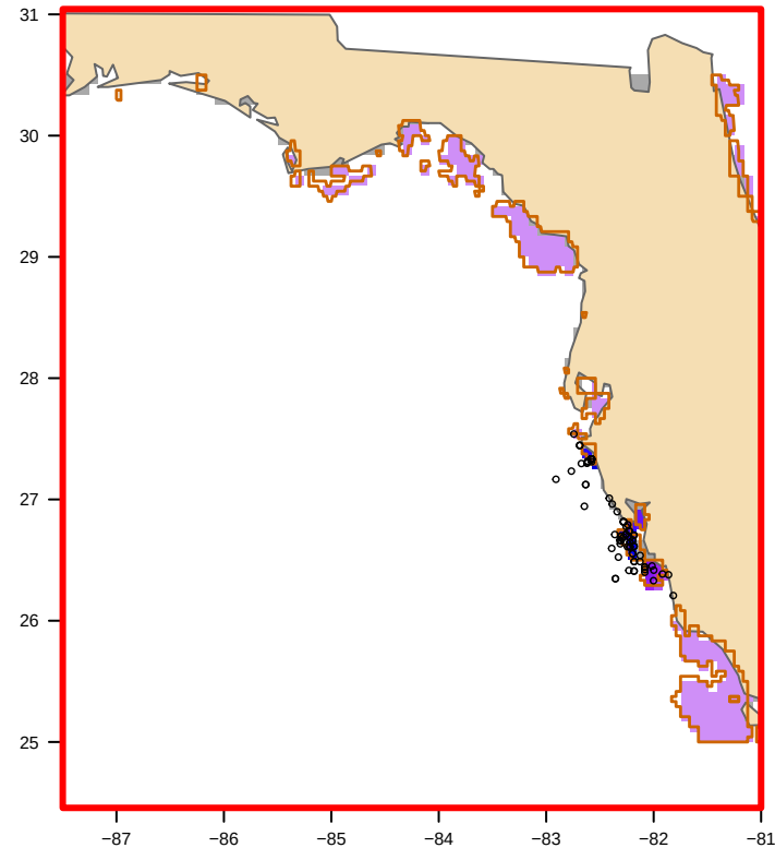
USED: MODIS nFLH-clipped (31 polygon(s)) bloom area 11,896 km 2
