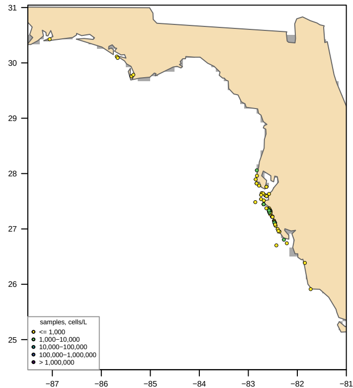
Unclipped sdmTMB (fitted, converged = TRUE) bloom area 0 km 2 , max 2,101 cells/L
