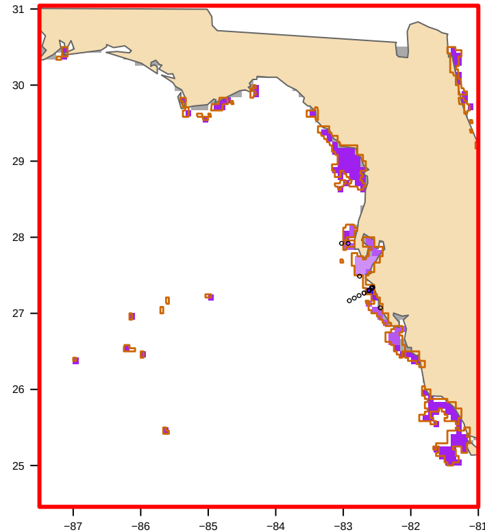
USED: MODIS nFLH-clipped (36 polygon(s)) bloom area 10,685 km 2
