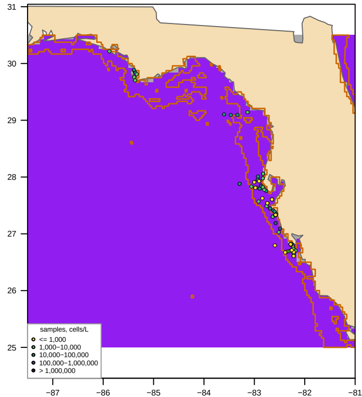
Unclipped sdmTMB (fitted, converged = TRUE) bloom area 291,361 km 2 , max 40,254 cells/L
