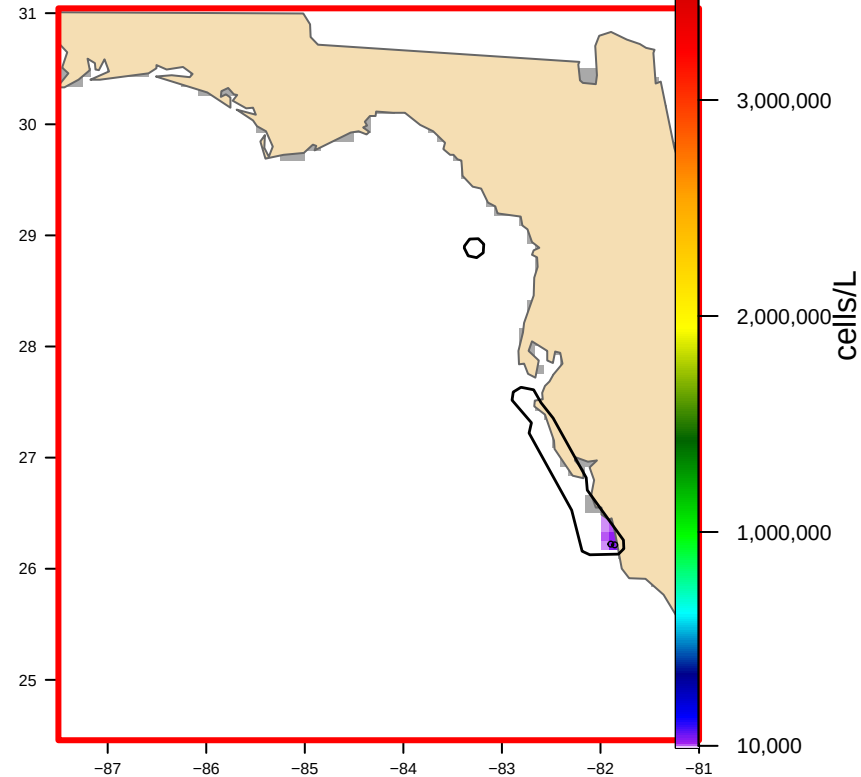
USED: Hull-clipped (2 footprint(s), 5,617 km 2 ) bloom area 537 km 2
