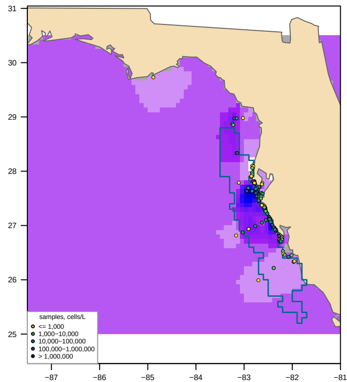
Unclipped sdmTMB (fitted, converged = TRUE) bloom area 290,983 km 2 , max 293,029 cells/L
