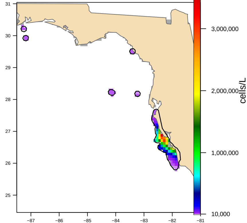
Hull-clipped (6 footprint(s), 9,563 km 2 ) bloom area 7,310 km 2
