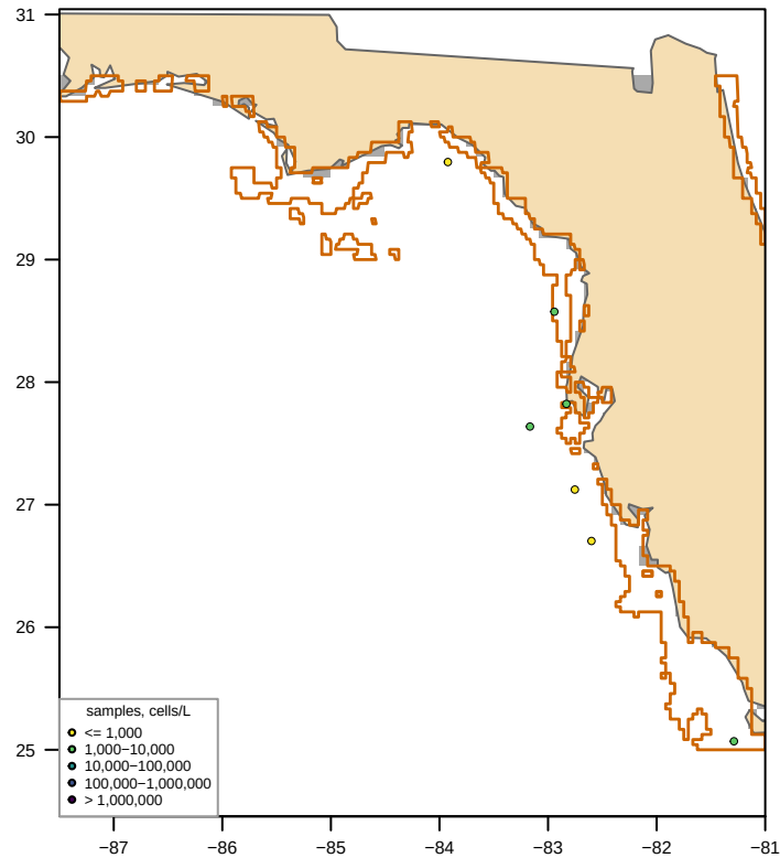
Unclipped sdmTMB (fitted, converged = TRUE) bloom area 0 km 2 , max 4,947 cells/L
