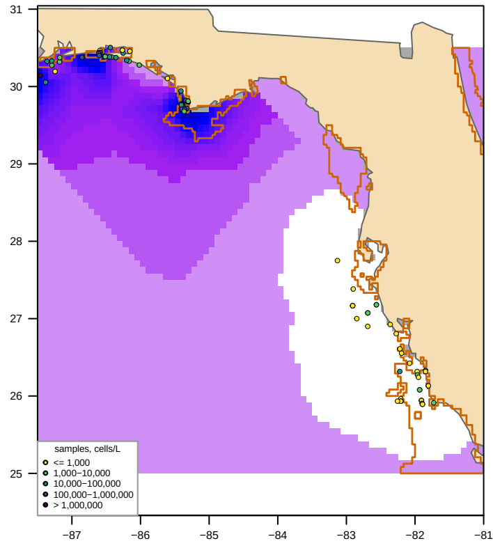
Unclipped sdmTMB (fitted, converged = TRUE) bloom area 235,364 km 2 , max 348,828 cells/L
