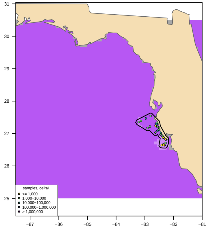
Unclipped sdmTMB (fitted, converged = TRUE) bloom area 291,361 km 2 , max 22,319 cells/L
