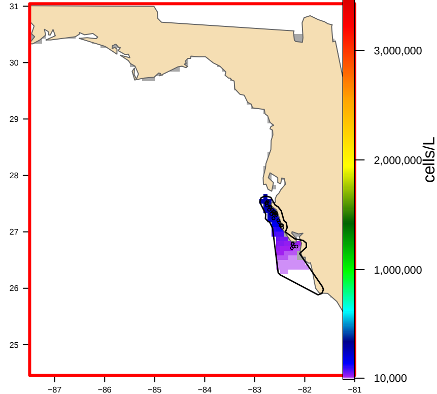
USED: Hull-clipped (1 footprint(s), 8,430 km 2 ) bloom area 4,962 km 2
