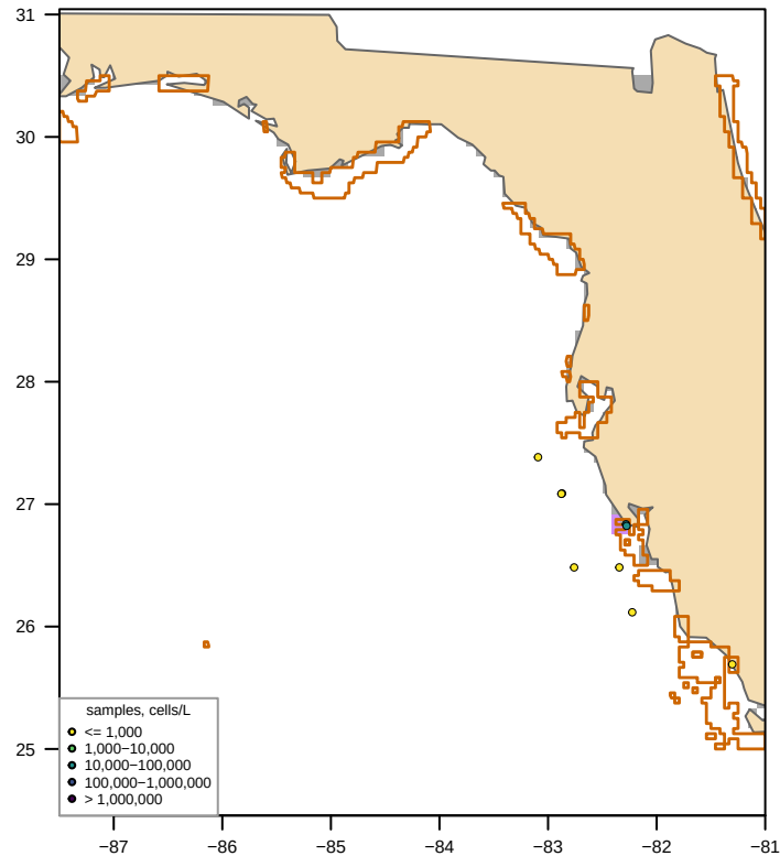
Unclipped sdmTMB (fitted, converged = TRUE) bloom area 229 km2, max 13,216 cells/L
