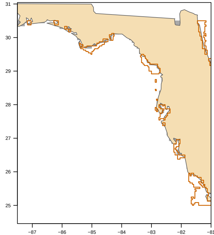
MODIS nFLH-clipped (18 polygon(s)) bloom area 0 km 2
