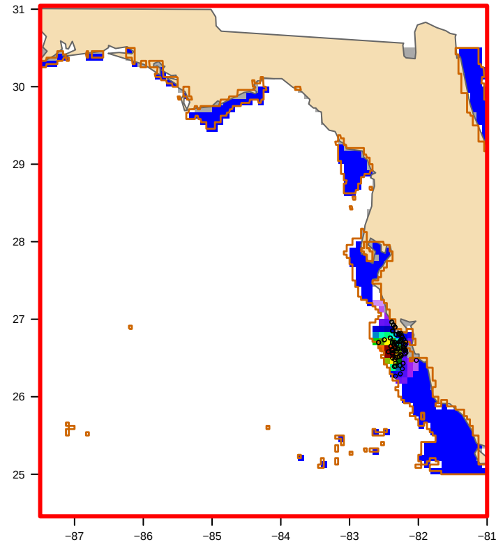
USED: MODIS nFLH-clipped (38 polygon(s)) bloom area 24,969 km 2
