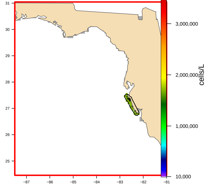
USED: Hull-clipped (1 footprint(s), 2,109 km 2 ) bloom area 1,370 km 2
