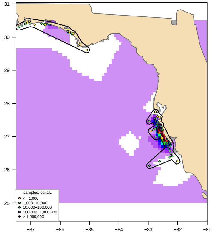
Unclipped sdmTMB (fitted, converged = TRUE) bloom area 248,084 km2, max 6,448,972 cells/L
