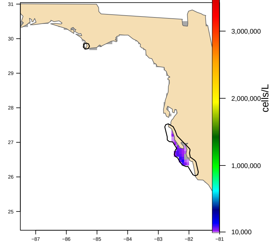
Hull-clipped (2 footprint(s), 6,437 km 2 ) bloom area 2,292 km 2
