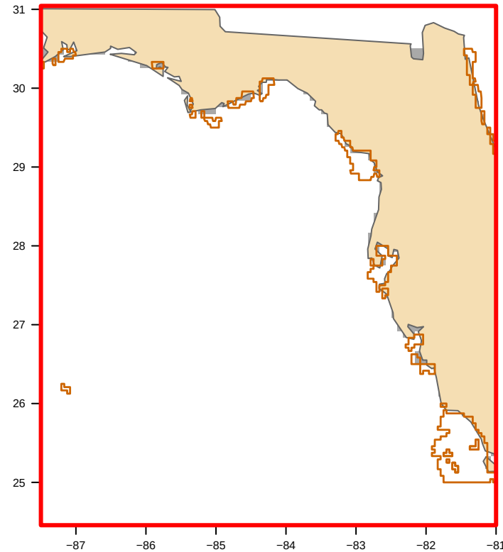
USED: MODIS nFLH-clipped (30 polygon(s)) bloom area 0 km2
