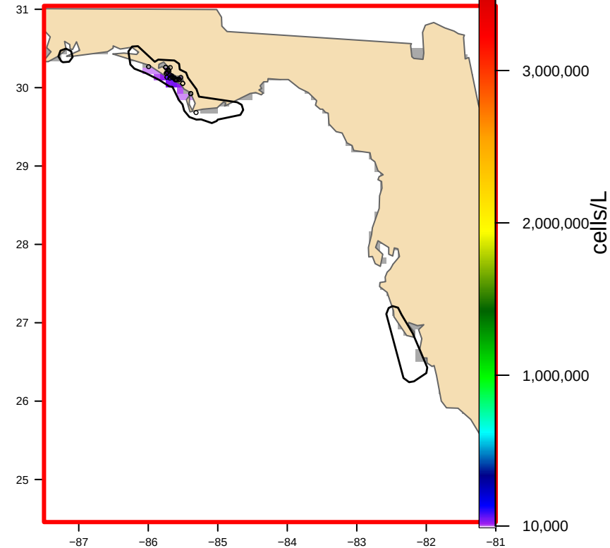
USED: Hull-clipped (3 footprint(s), 8,748 km 2 ) bloom area 1,258 km 2
