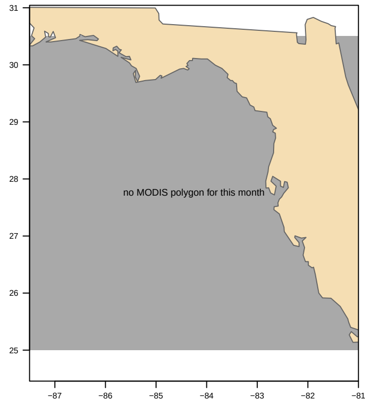
MODIS nFLH-clipped
