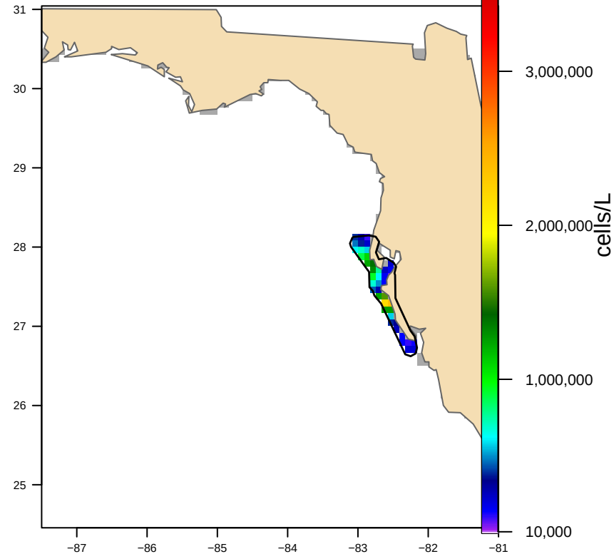
Hull-clipped (1 footprint(s), 5,035 km 2 ) bloom area 3,262 km 2
