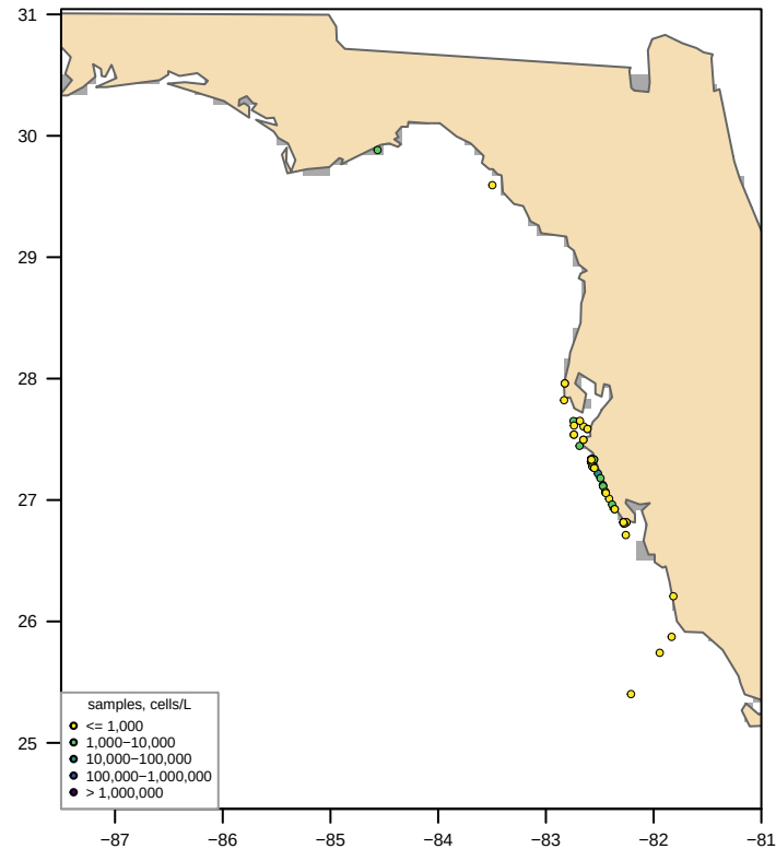
Unclipped sdmTMB (fitted, converged = TRUE) bloom area 0 km2, max 4,172 cells/L
