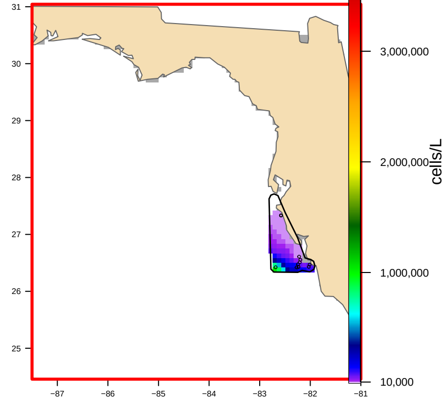
USED: Hull-clipped (1 footprint(s), 7,636 km 2 ) bloom area 6,110 km 2
