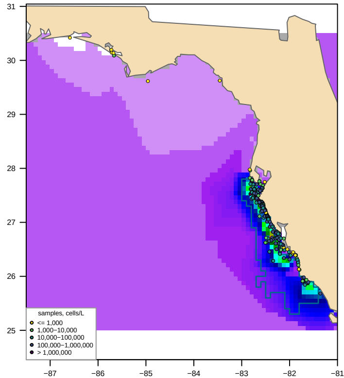
Unclipped sdmTMB (fitted, converged = TRUE) bloom area 288,915 km 2 , max 2,720,364 cells/L
