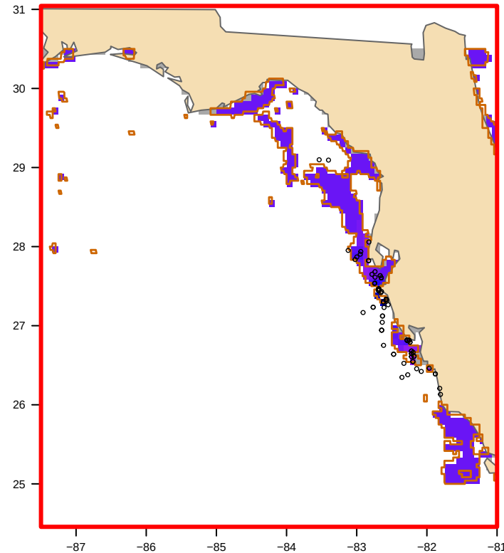
USED: MODIS nFLH-clipped (41 polygon(s)) bloom area 18,709 km2
