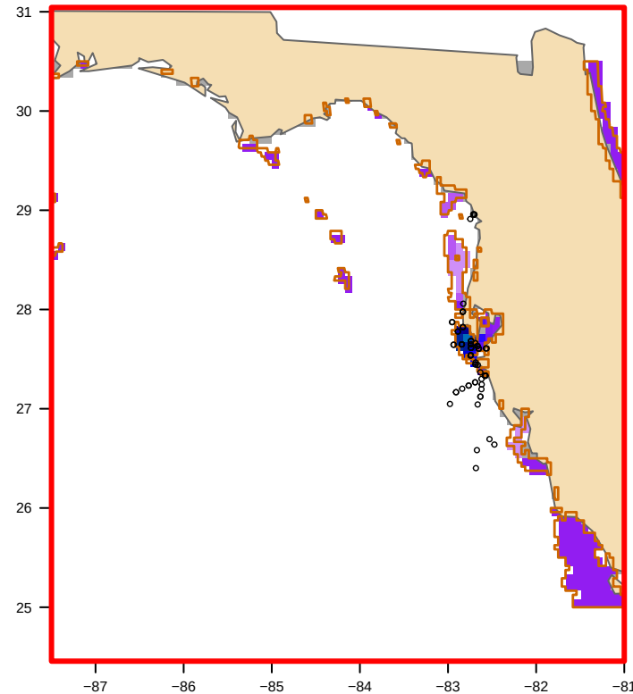
USED: MODIS nFLH-clipped (41 polygon(s)) bloom area 12,224 km 2
