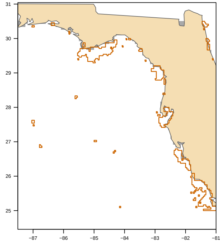
MODIS nFLH-clipped (39 polygon(s)) bloom area 0 km2
