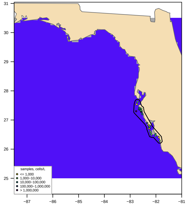
Unclipped sdmTMB (fitted, converged = TRUE) bloom area 291,361 km 2 , max 98,743 cells/L
