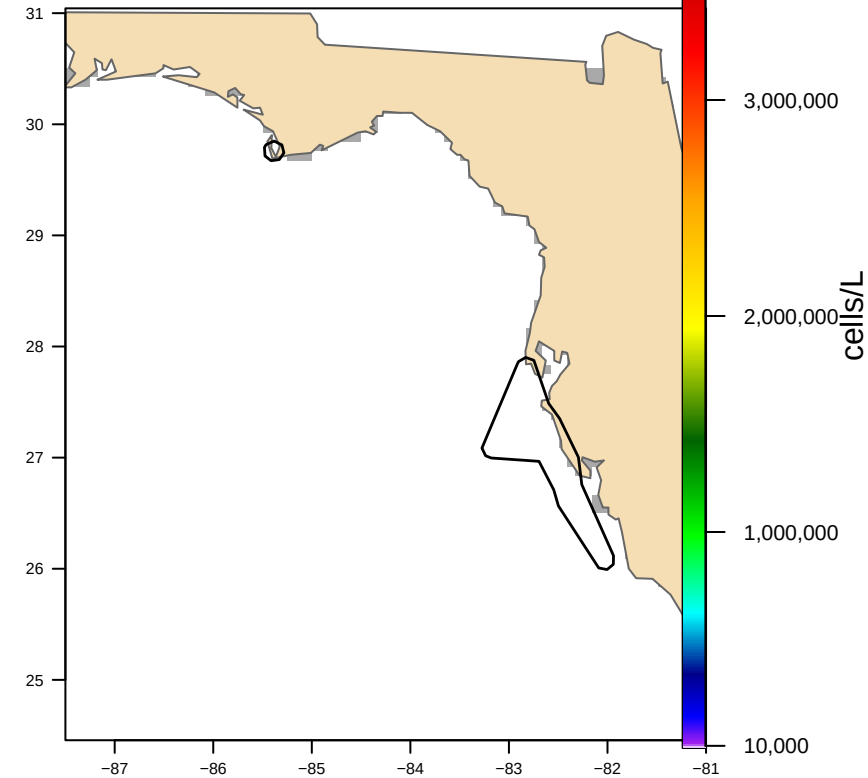
Hull-clipped (2 footprint(s), 9,258 km 2 ) bloom area 0 km 2
