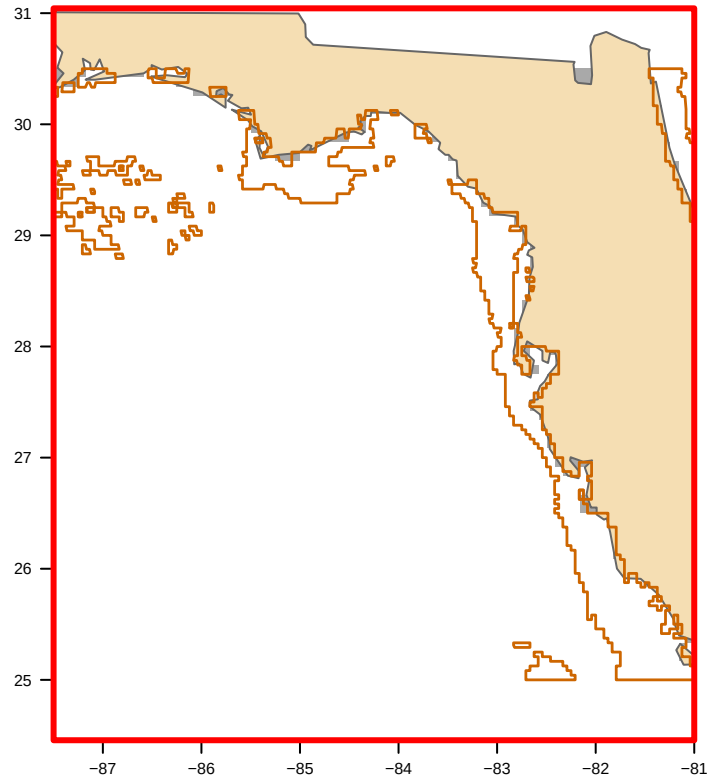
USED: MODIS nFLH-clipped (55 polygon(s)) bloom area 0 km 2
