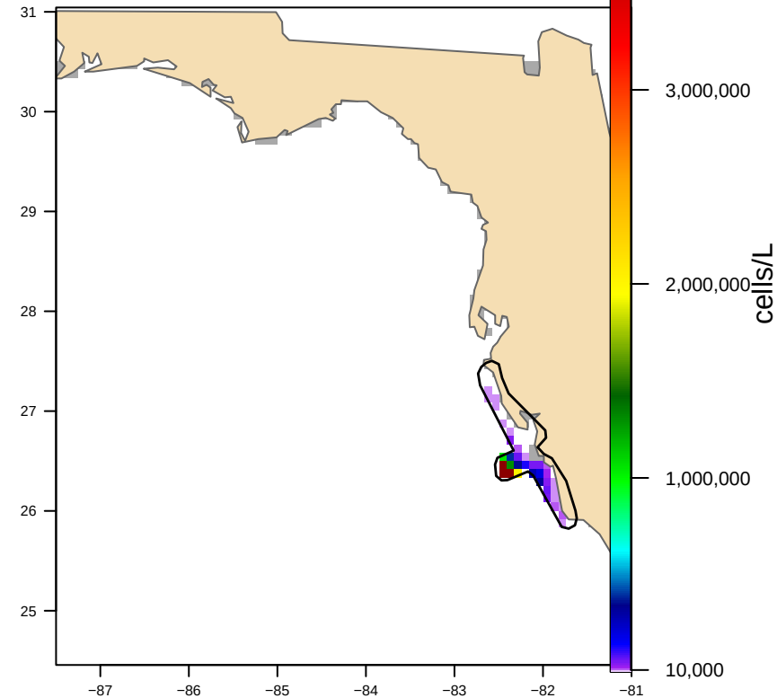
Hull-clipped (1 footprint(s), 6,677 km 2 ) bloom area 2,834 km 2
