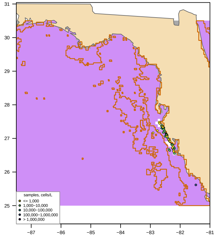
Unclipped sdmTMB (fitted, converged = TRUE) bloom area 290,447 km 2 , max 18,510 cells/L
