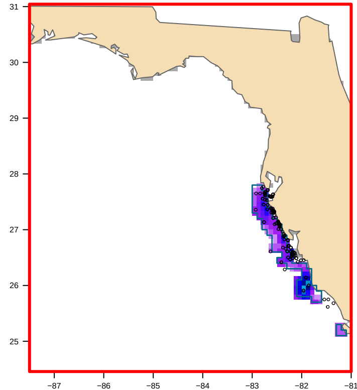
USED: VIIRS-clipped (67 positive VIIRS cells) bloom area 9,482 km 2
