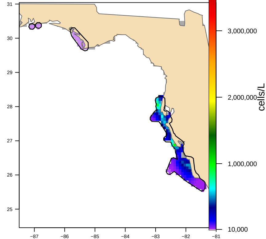
Hull-clipped (4 footprint(s), 17,365 km 2 ) bloom area 13,386 km 2
