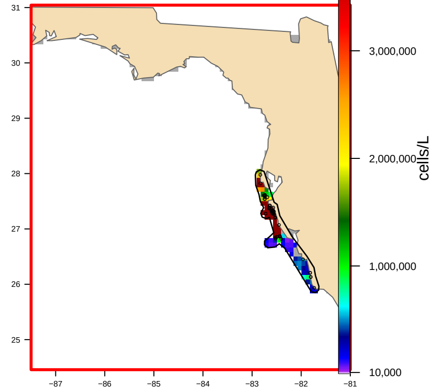
USED: Hull-clipped (2 footprint(s), 8,023 km 2 ) bloom area 5,494 km 2
