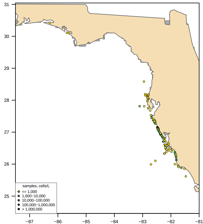
Unclipped sdmTMB (fitted, converged = TRUE) bloom area 0 km 2 , max 5,824 cells/L
