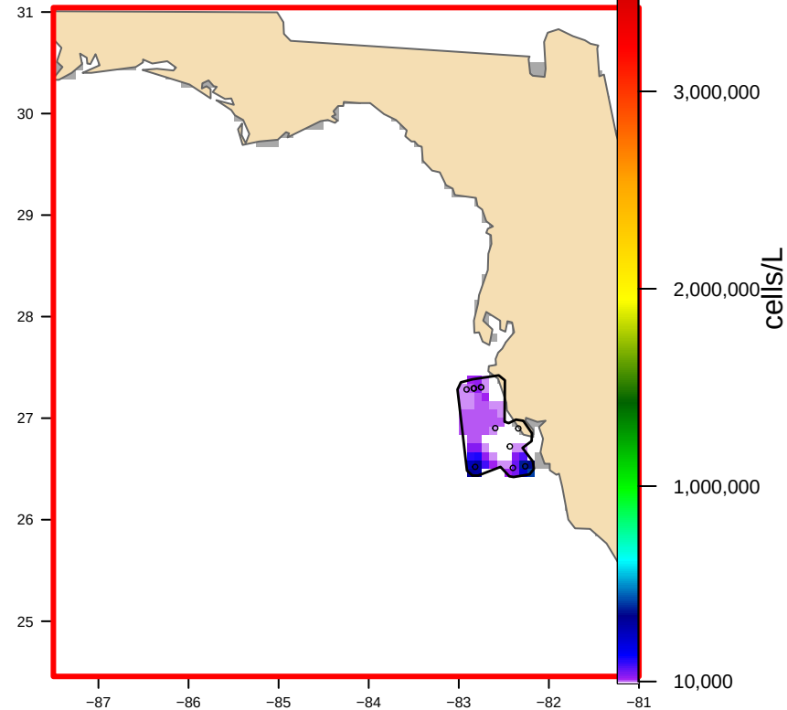
USED: Hull-clipped (1 footprint(s), 6,554 km 2 ) bloom area 4,731 km 2
