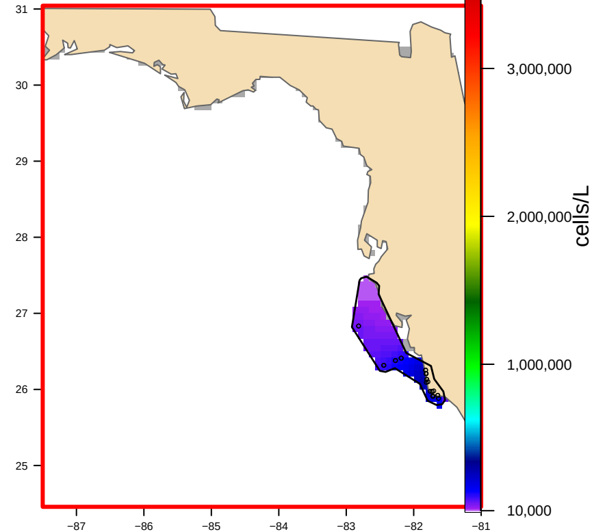
USED: Hull-clipped (1 footprint(s), 8,542 km 2 ) bloom area 7,951 km 2
