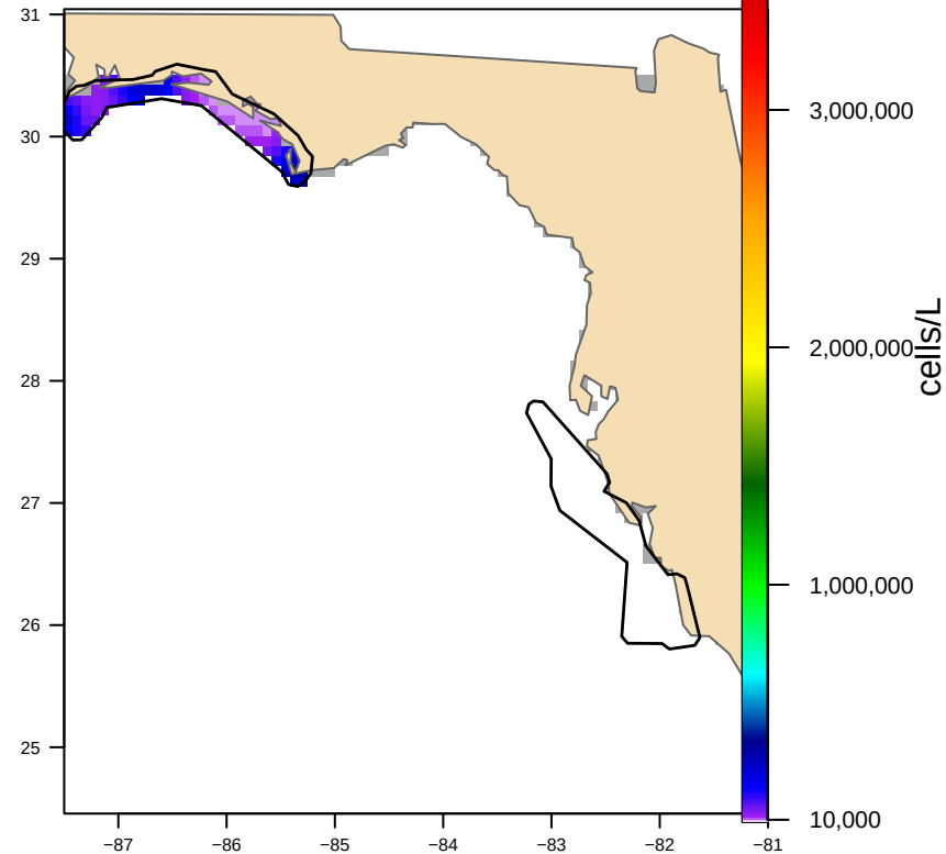
Hull-clipped (2 footprint(s), 18,625 km 2 ) bloom area 5,770 km 2
