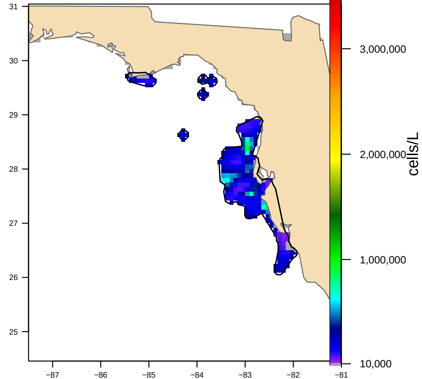
Hull-clipped (5 footprint(s), 20,359 km 2 ) bloom area 17,079 km 2
