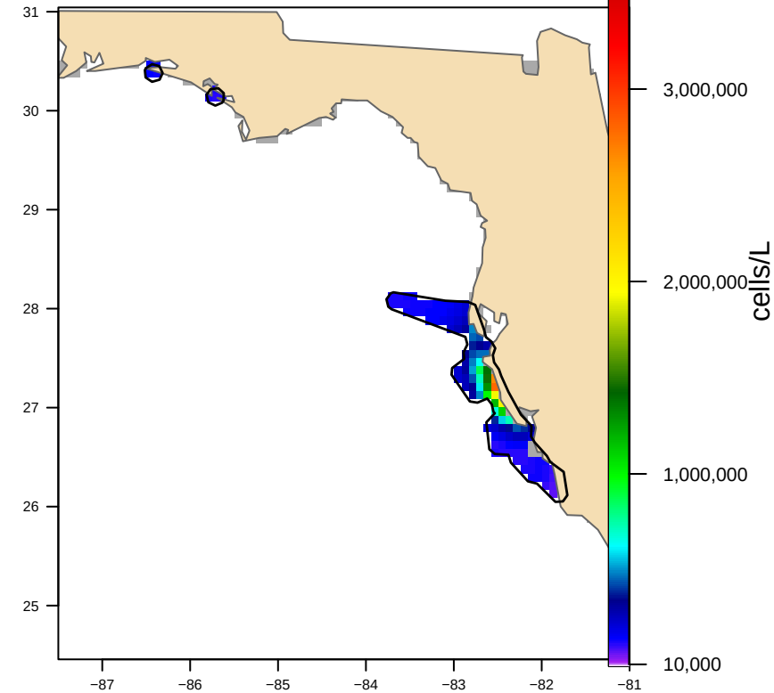
Hull-clipped (3 footprint(s), 11,596 km 2 ) bloom area 9,261 km 2
