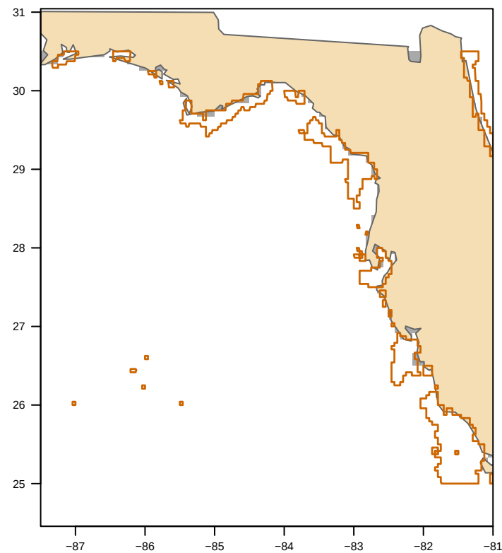
MODIS nFLH-clipped (35 polygon(s)) bloom area 0 km 2
