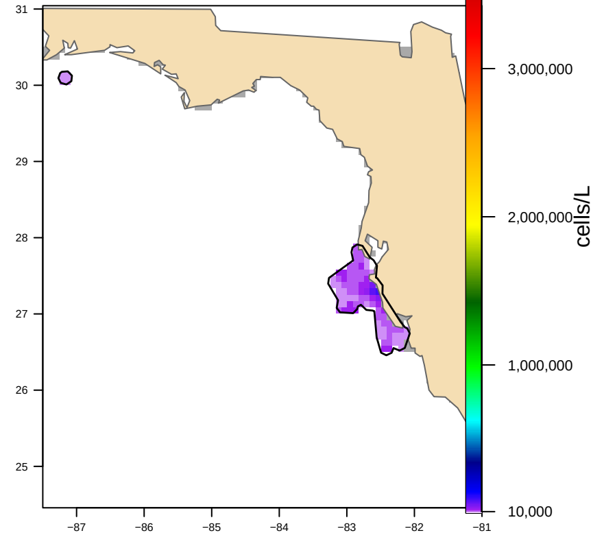
Hull-clipped (2 footprint(s), 8,145 km 2 ) bloom area 6,840 km 2
