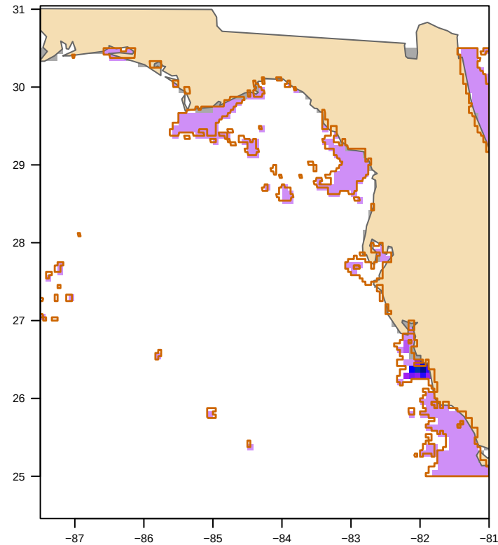
MODIS nFLH-clipped (62 polygon(s)) bloom area 21,236 km 2
