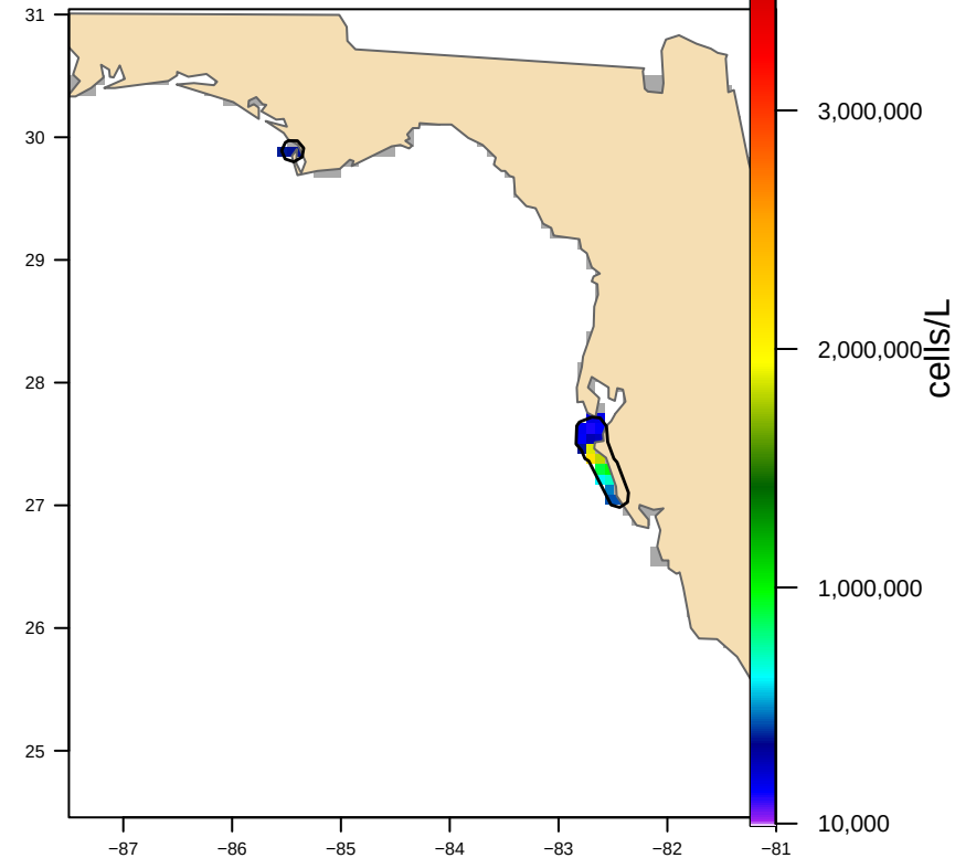
Hull-clipped (2 footprint(s), 2,278 km 2 ) bloom area 1,665 km 2
