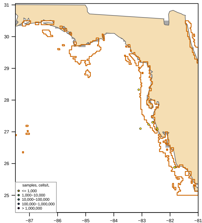
Unclipped sdmTMB (fitted, converged = FALSE) bloom area 0 km2, max 1,000 cells/L
