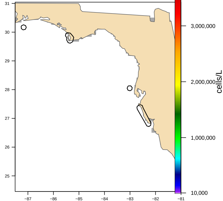
Hull-clipped (4 footprint(s), 3,426 km 2 ) bloom area 0 km 2
