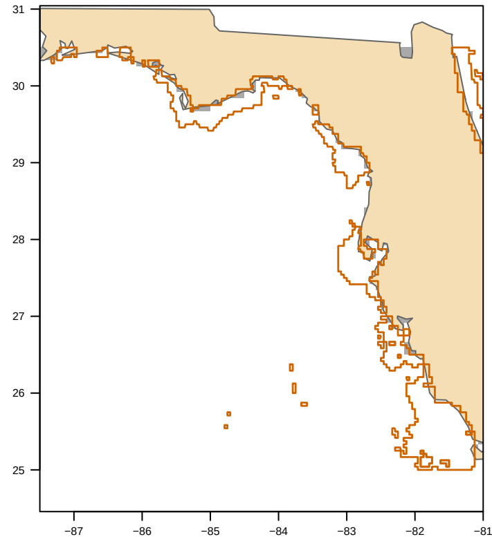
MODIS nFLH-clipped (41 polygon(s)) bloom area 0 km 2
