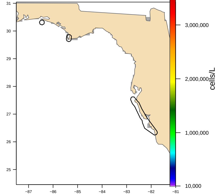
Hull-clipped (3 footprint(s), 5,093 km 2 ) bloom area 0 km 2
