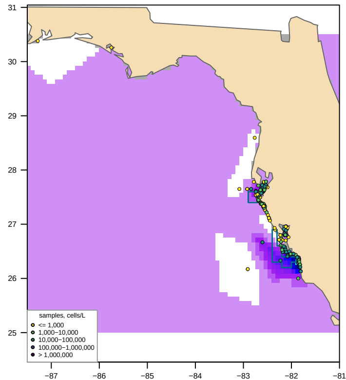
Unclipped sdmTMB (fitted, converged = TRUE) bloom area 267,749 km 2 , max 638,460 cells/L
