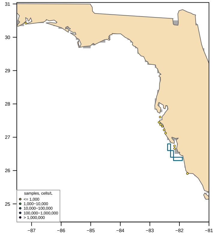
Unclipped sdmTMB (fitted, converged = TRUE) bloom area 0 km2, max 895 cells/L
