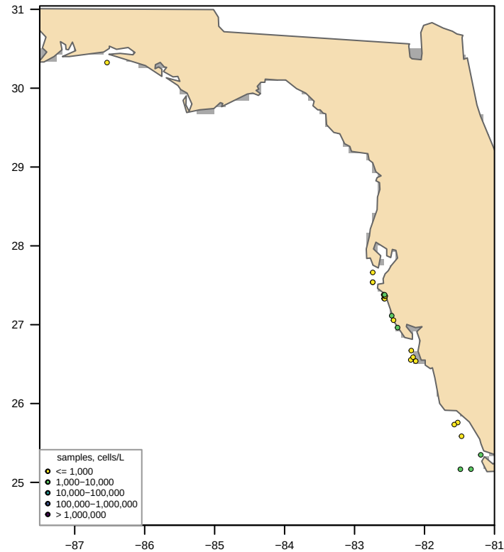
Unclipped sdmTMB (fitted, converged = TRUE) bloom area 0 km 2 , max 3,880 cells/L
