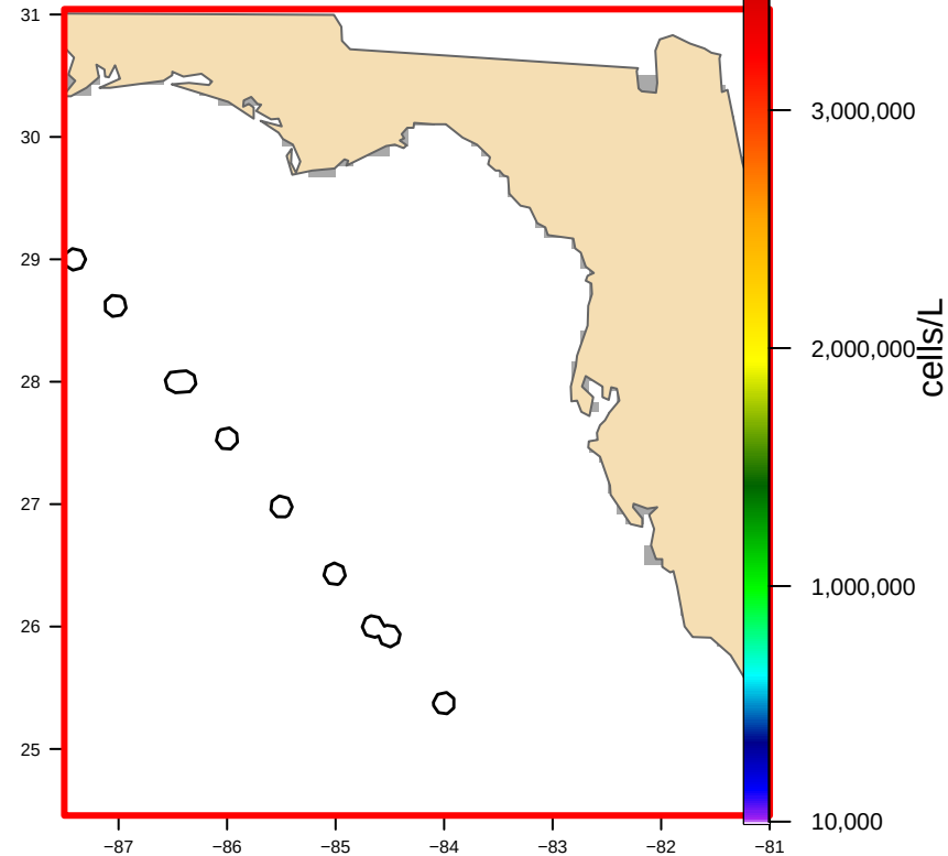
USED: Hull-clipped (8 footprint(s), 2,970 km2) bloom area 0 km2
