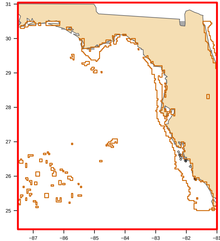
USED: MODIS nFLH-clipped (71 polygon(s)) bloom area 0 km2
