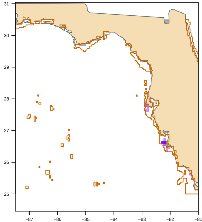
MODIS nFLH-clipped (41 polygon(s)) bloom area 1,144 km 2
