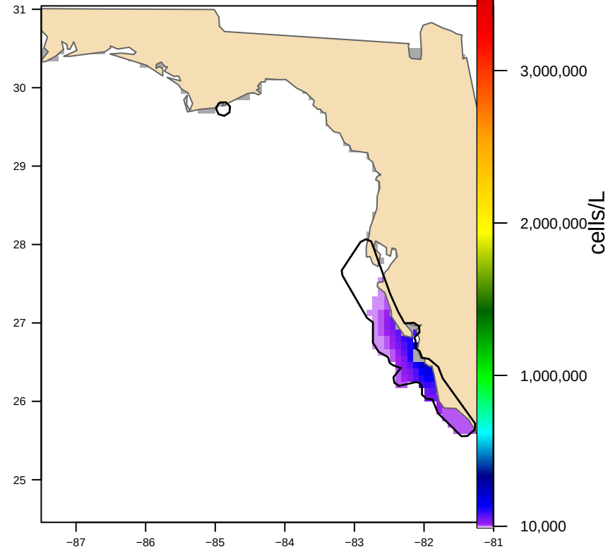
Hull-clipped (2 footprint(s), 14,016 km 2 ) bloom area 7,808 km 2
