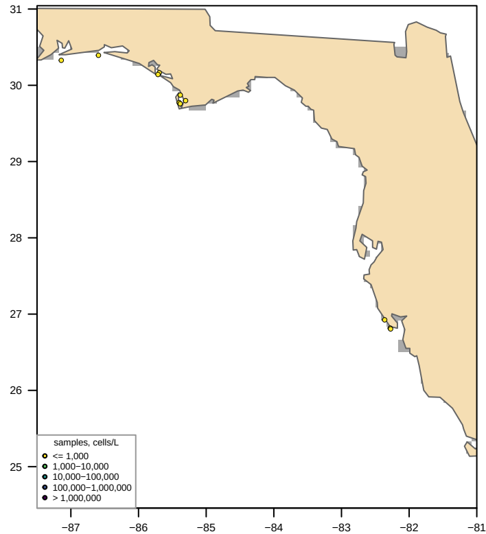
Unclipped sdmTMB (fitted, converged = TRUE) bloom area 0 km 2 , max 560 cells/L
