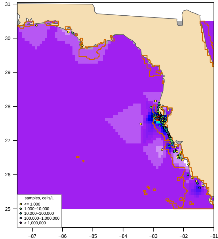
Unclipped sdmTMB (fitted, converged = TRUE) bloom area 291,054 km 2 , max 4,789,492 cells/L
