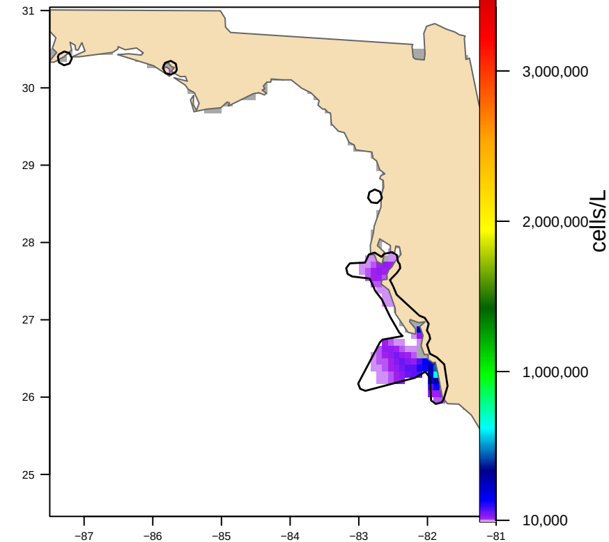
Hull-clipped (4 footprint(s), 13,272 km 2 ) bloom area 7,786 km 2
