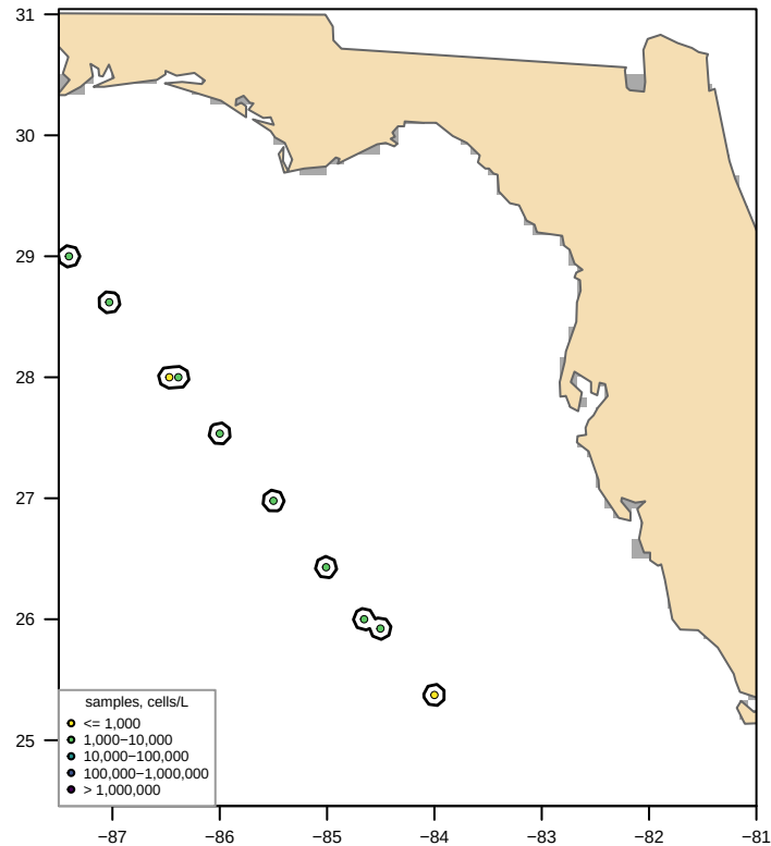
Unclipped sdmTMB (fitted, converged = TRUE) bloom area 0 km2, max 2,840 cells/L
