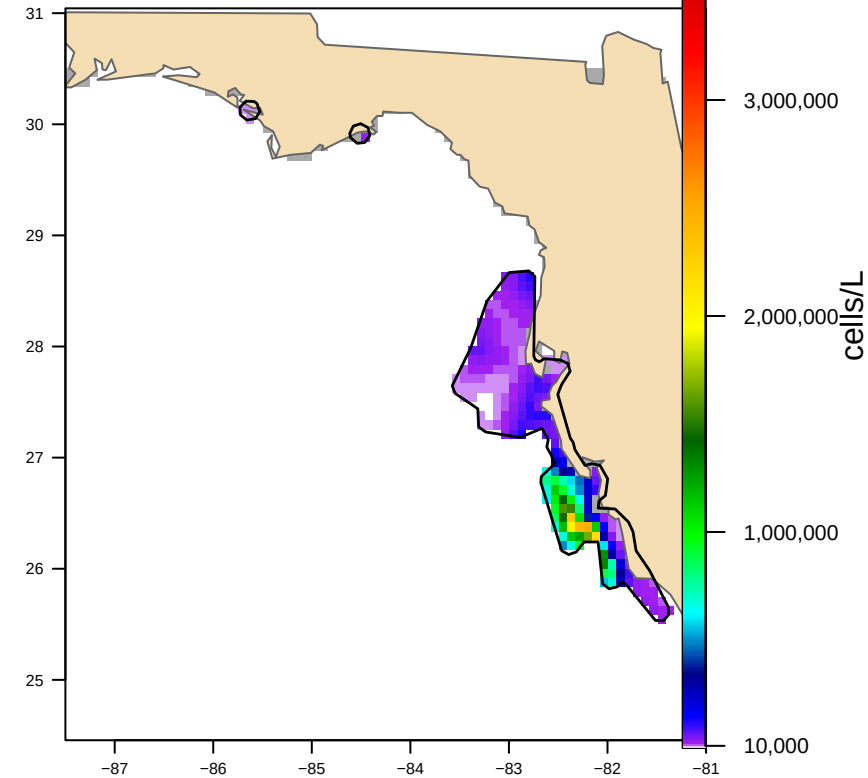
Hull-clipped (3 footprint(s), 21,481 km 2 ) bloom area 18,016 km 2
