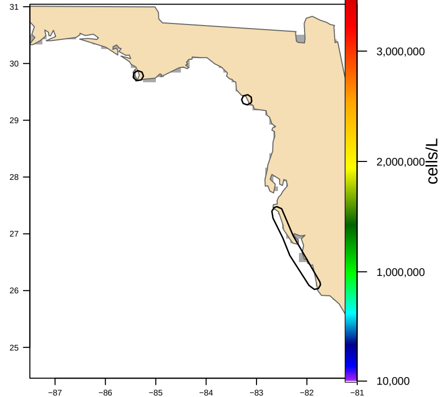
Hull-clipped (3 footprint(s), 4,620 km 2 ) bloom area 0 km 2
