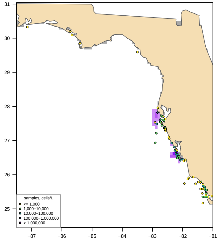
Unclipped sdmTMB (fitted, converged = TRUE) bloom area 2,208 km 2 , max 78,879 cells/L
