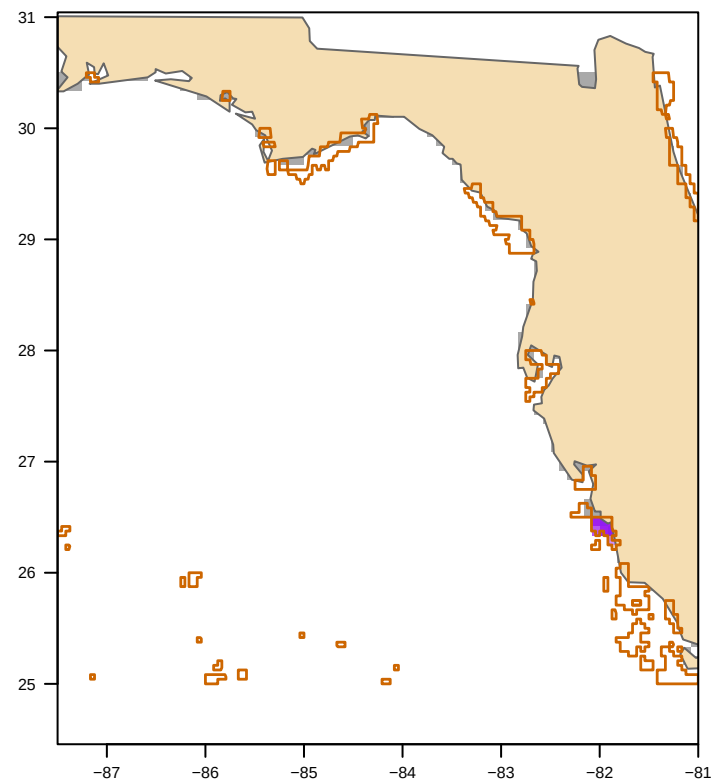
MODIS nFLH-clipped (41 polygon(s)) bloom area 536 km 2
