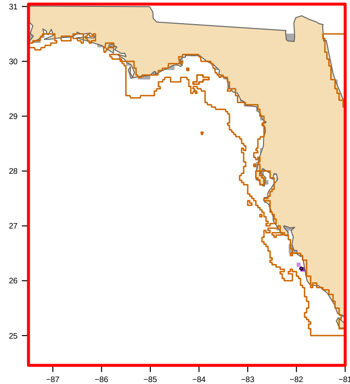
USED: MODIS nFLH-clipped (19 polygon(s)) bloom area 153 km 2
