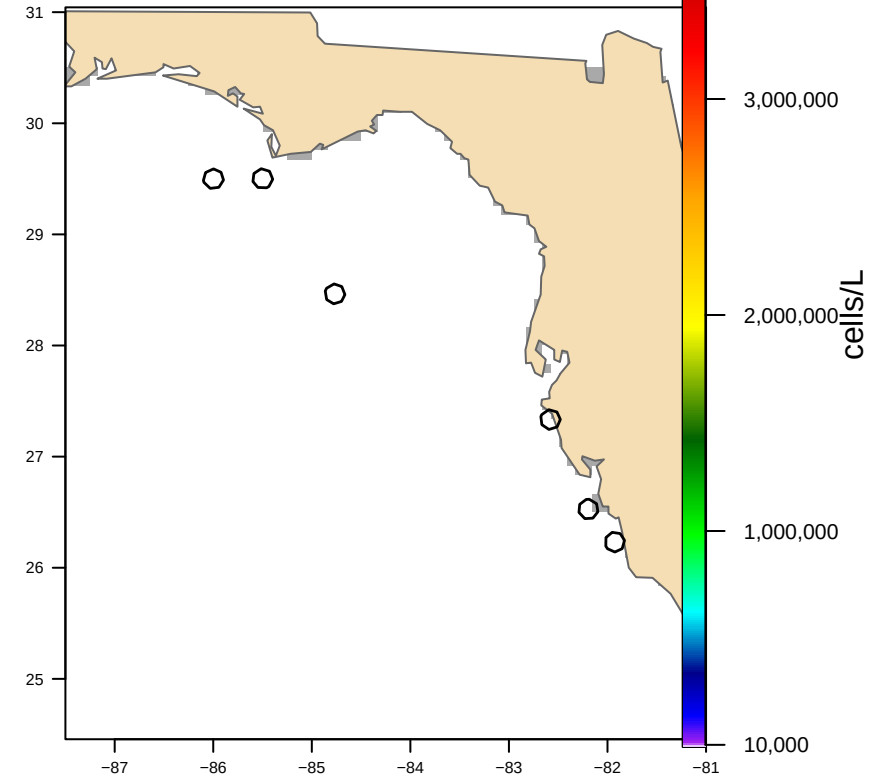
Hull-clipped (6 footprint(s), 1,884 km2) bloom area 0 km2
