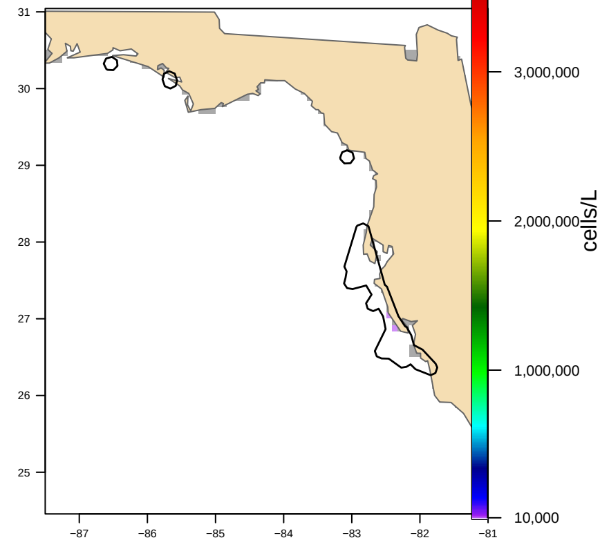
Hull-clipped (4 footprint(s), 9,988 km 2 ) bloom area 152 km 2
