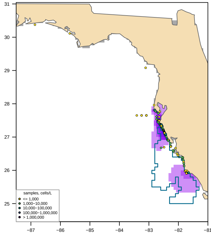
Unclipped sdmTMB (fitted, converged = TRUE) bloom area 12,797 km 2 , max 95,374 cells/L
