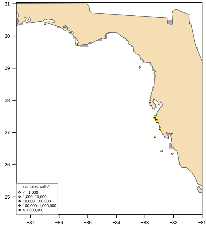
Unclipped sdmTMB (fitted, converged = TRUE) bloom area 0 km 2 , max 3,050 cells/L
