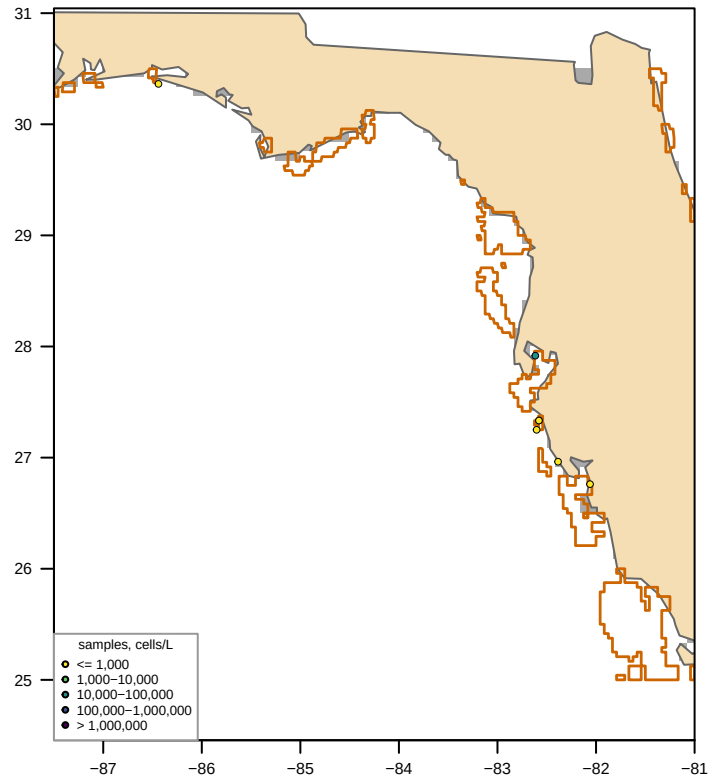
Unclipped sdmTMB (fitted, converged = TRUE) bloom area 0 km 2 , max 2,625 cells/L
