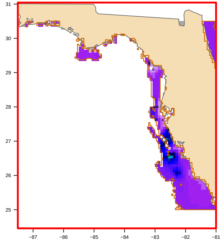
USED: MODIS nFLH-clipped (28 polygon(s)) bloom area 38,022 km 2
