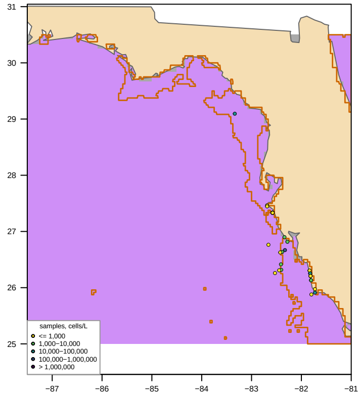
Unclipped sdmTMB (fitted, converged = TRUE) bloom area 291,361 km 2 , max 18,476 cells/L
