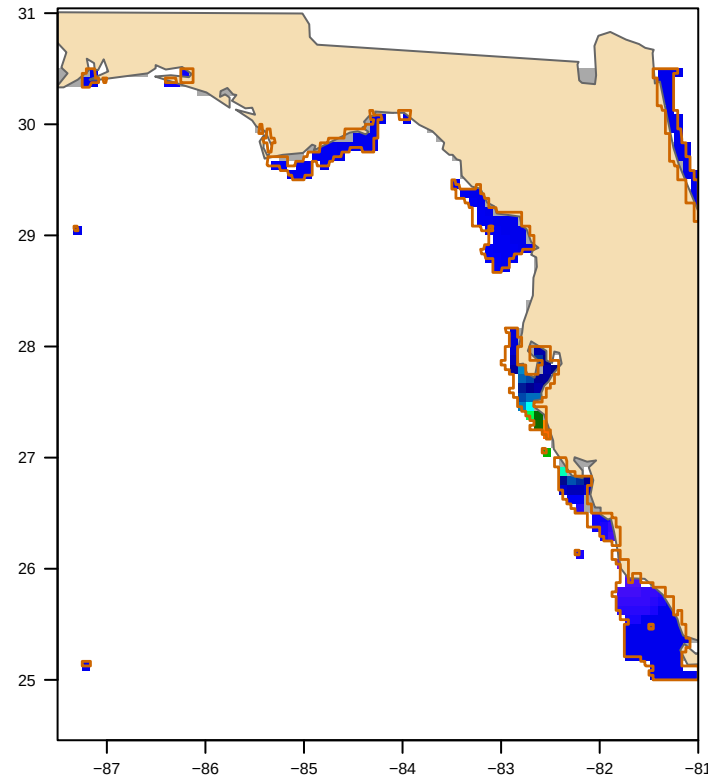
MODIS nFLH-clipped (19 polygon(s)) bloom area 16,283 km 2
