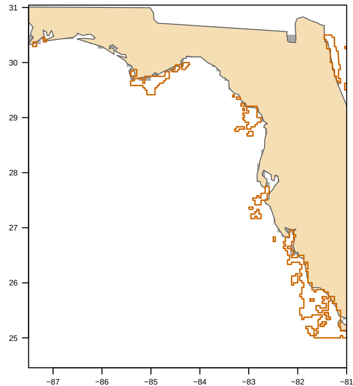
MODIS nFLH-clipped (26 polygon(s)) bloom area 0 km 2
