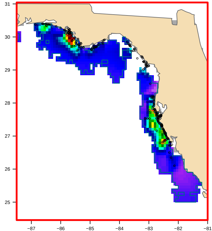
USED: VIIRS-clipped (482 positive VIIRS cells) bloom area 63,315 km 2
