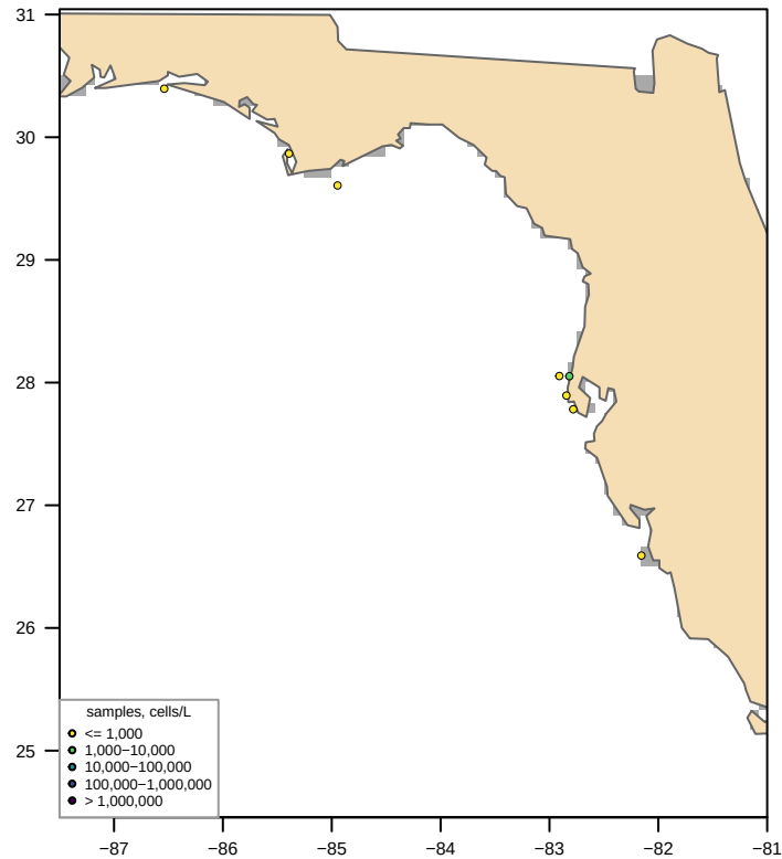
Unclipped sdmTMB (fitted, converged = TRUE) bloom area 0 km 2 , max 632 cells/L
