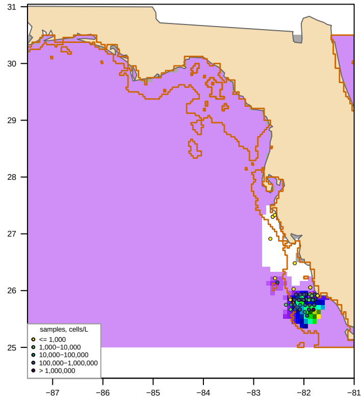
Unclipped sdmTMB (fitted, converged = TRUE) bloom area 283,719 km 2 , max 2,097,662 cells/L
