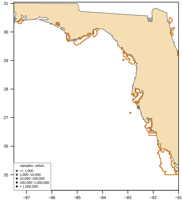
Unclipped sdmTMB (fitted, converged = TRUE) bloom area 0 km2, max 701 cells/L
