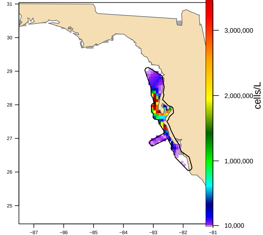
Hull-clipped (1 footprint(s), 14,206 km 2 ) bloom area 9,984 km 2
