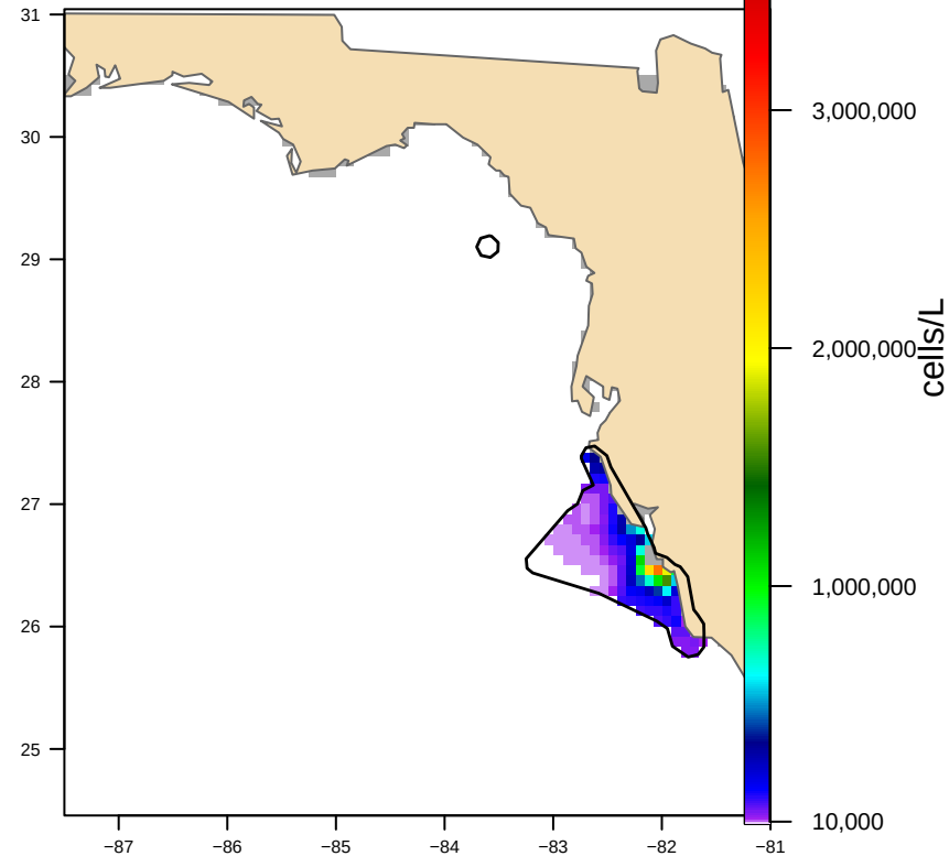
Hull-clipped (2 footprint(s), 12,570 km 2 ) bloom area 9,258 km 2
