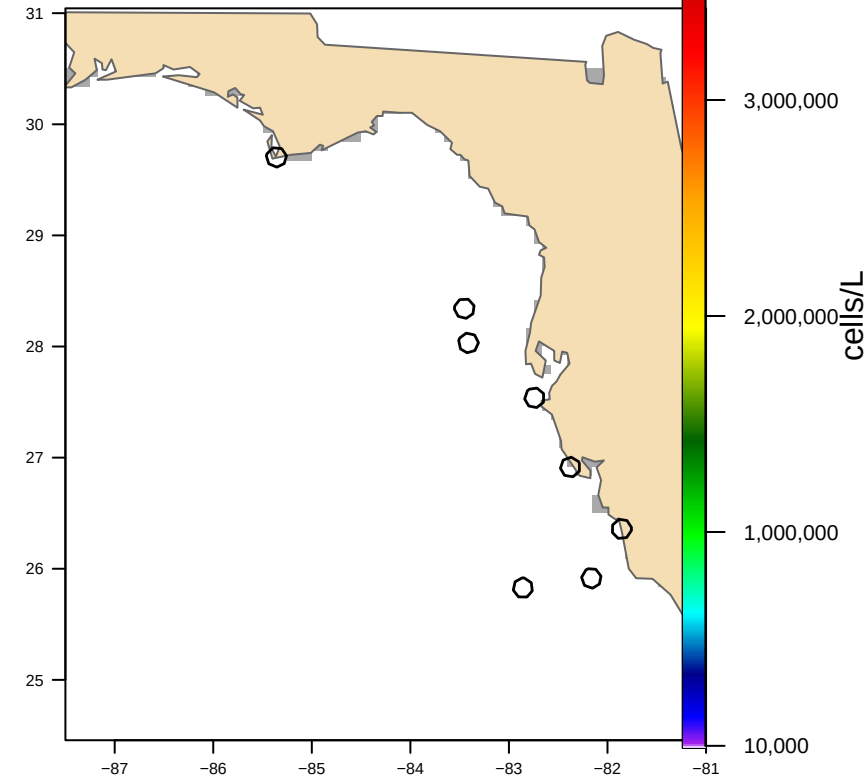
Hull-clipped (8 footprint(s), 2,512 km 2 ) bloom area 0 km 2
