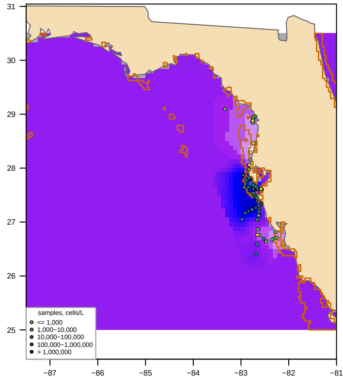
Unclipped sdmTMB (fitted, converged = TRUE) bloom area 291,210 km 2 , max 477,141 cells/L
