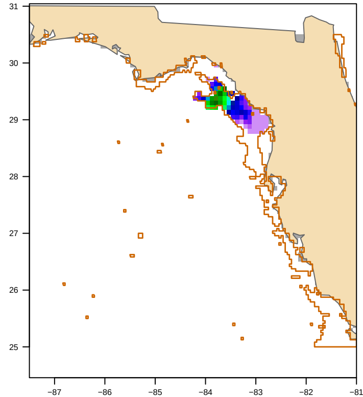
MODIS nFLH-clipped (48 polygon(s)) bloom area 6,271 km 2
