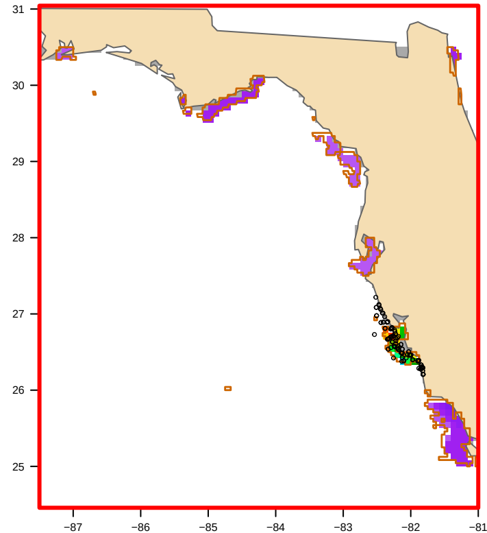
USED: MODIS nFLH-clipped (19 polygon(s)) bloom area 9,702 km 2
