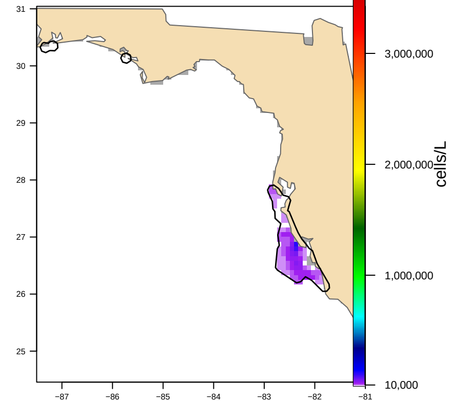
Hull-clipped (3 footprint(s), 10,452 km 2 ) bloom area 6,417 km 2
