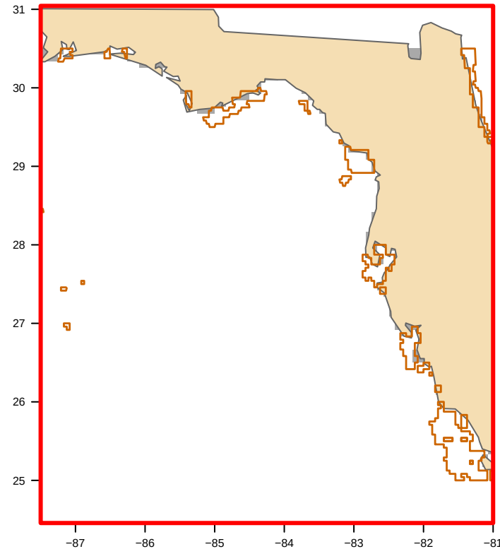
USED: MODIS nFLH-clipped (28 polygon(s)) bloom area 0 km 2
