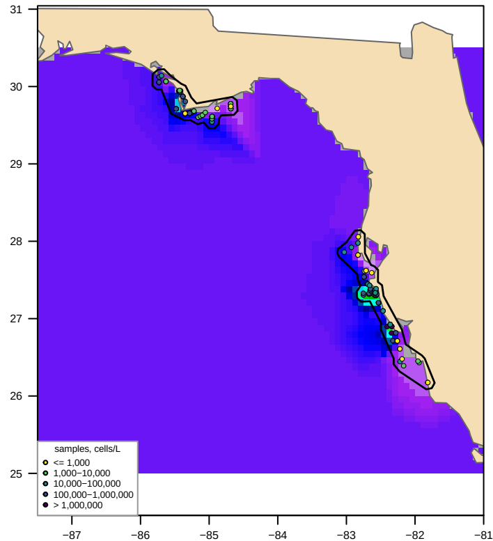
Unclipped sdmTMB (fitted, converged = TRUE) bloom area 291,361 km 2 , max 1,205,908 cells/L
