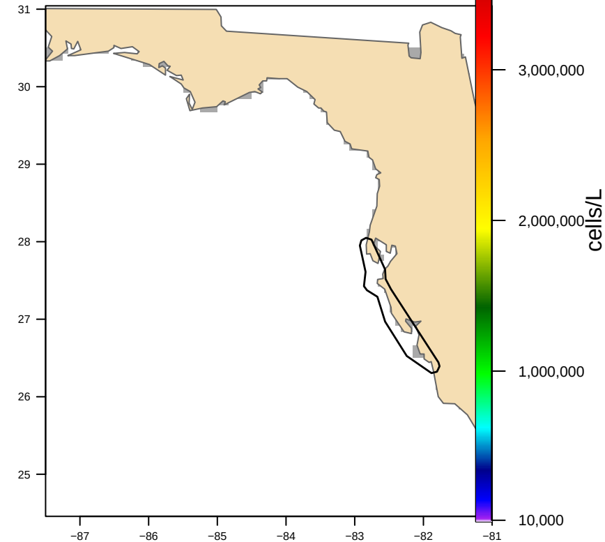
Hull-clipped (1 footprint(s), 6,092 km 2 ) bloom area 0 km 2
