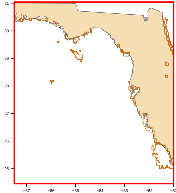
USED: MODIS nFLH-clipped (37 polygon(s)) bloom area 0 km2
