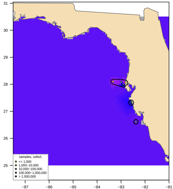
Unclipped sdmTMB (fitted, converged = TRUE) bloom area 291,361 km2, max 299,247 cells/L
