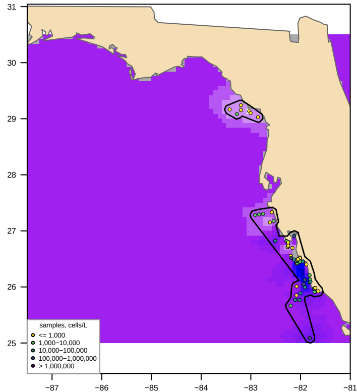
Unclipped sdmTMB (fitted, converged = TRUE) bloom area 291,286 km 2 , max 260,350 cells/L
