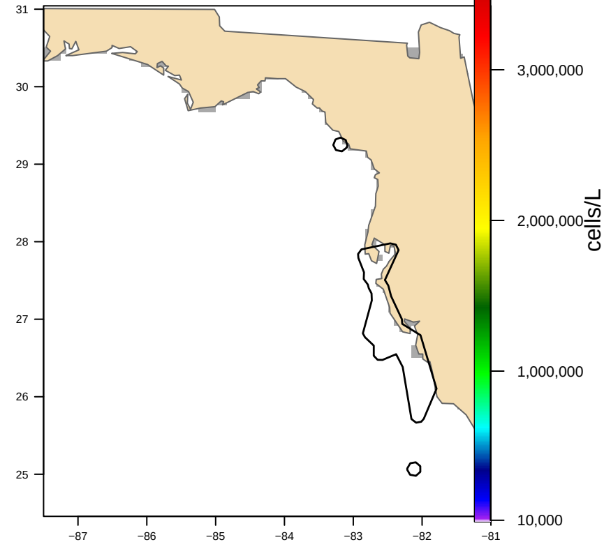
Hull-clipped (3 footprint(s), 12,050 km 2 ) bloom area 0 km 2
