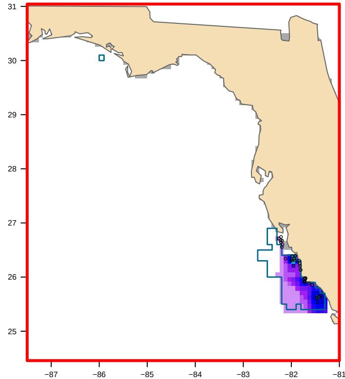
USED: VIIRS-clipped (88 positive VIIRS cells) bloom area 8,932 km 2
