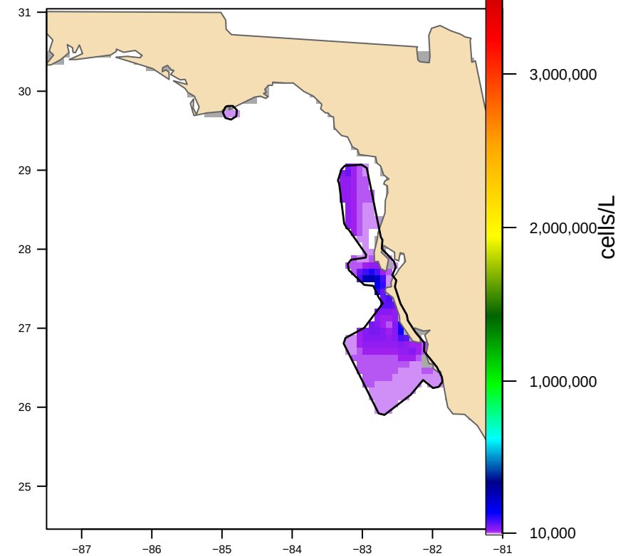
Hull-clipped (2 footprint(s), 20,823 km 2 ) bloom area 18,778 km 2
