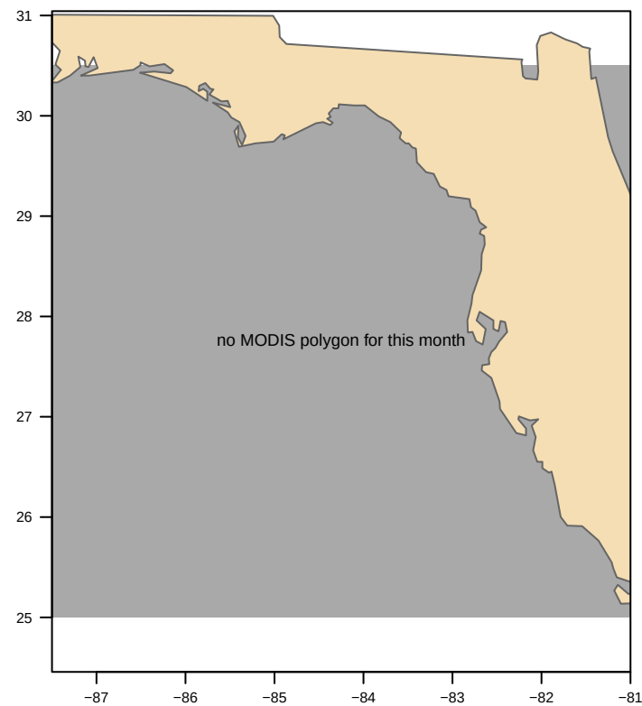
MODIS nFLH-clipped
