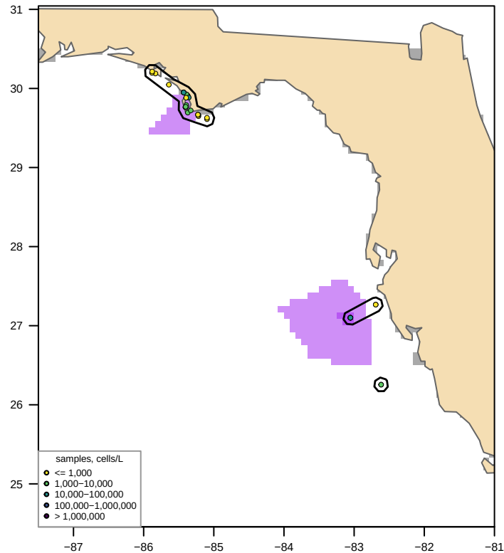
Unclipped sdmTMB (fitted, converged = TRUE) bloom area 13,052 km 2 , max 21,358 cells/L
