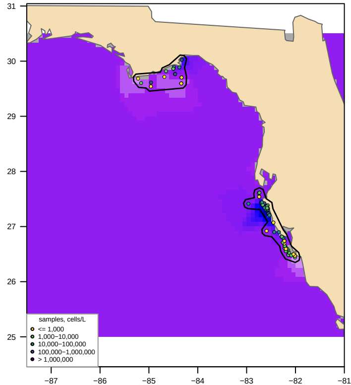
Unclipped sdmTMB (fitted, converged = TRUE) bloom area 291,361 km2, max 477,131 cells/L
