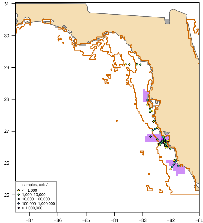
Unclipped sdmTMB (fitted, converged = TRUE) bloom area 4,970 km 2 , max 31,135 cells/L
