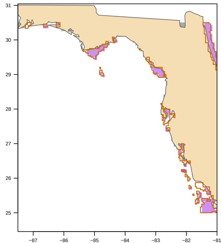
MODIS nFLH-clipped (29 polygon(s)) bloom area 8,376 km 2
