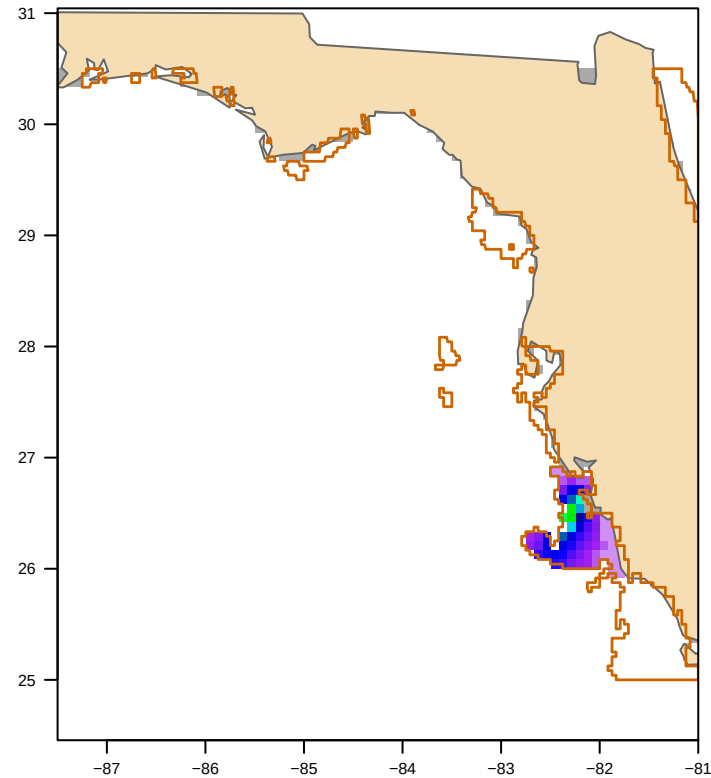
MODIS nFLH-clipped (26 polygon(s)) bloom area 5,213 km 2
