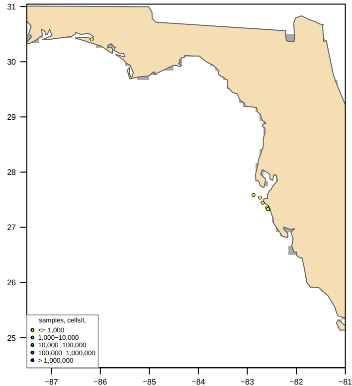
Unclipped sdmTMB (fitted, converged = TRUE) bloom area 0 km 2 , max 989 cells/L
