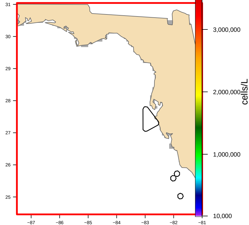
USED: Hull-clipped (4 footprint(s), 4,084 km 2 ) bloom area 0 km 2
