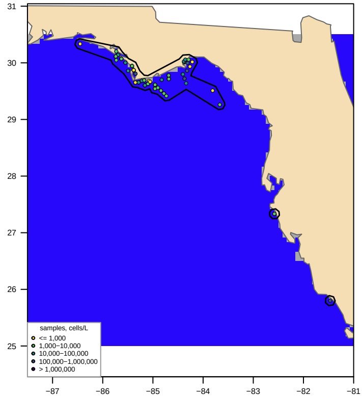
Unclipped sdmTMB (fitted, converged = TRUE) bloom area 291,361 km 2 , max 127,472 cells/L
