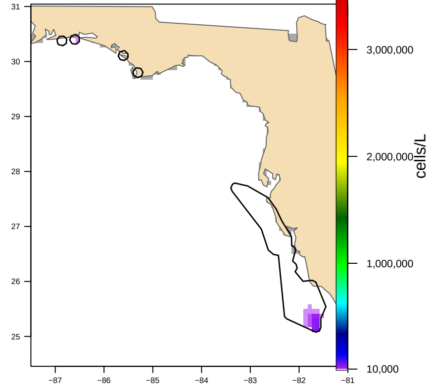
Hull-clipped (5 footprint(s), 18,086 km 2 ) bloom area 1,694 km 2
