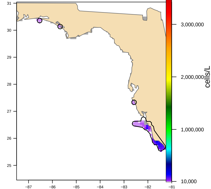
Hull-clipped (4 footprint(s), 6,549 km 2 ) bloom area 4,354 km 2
