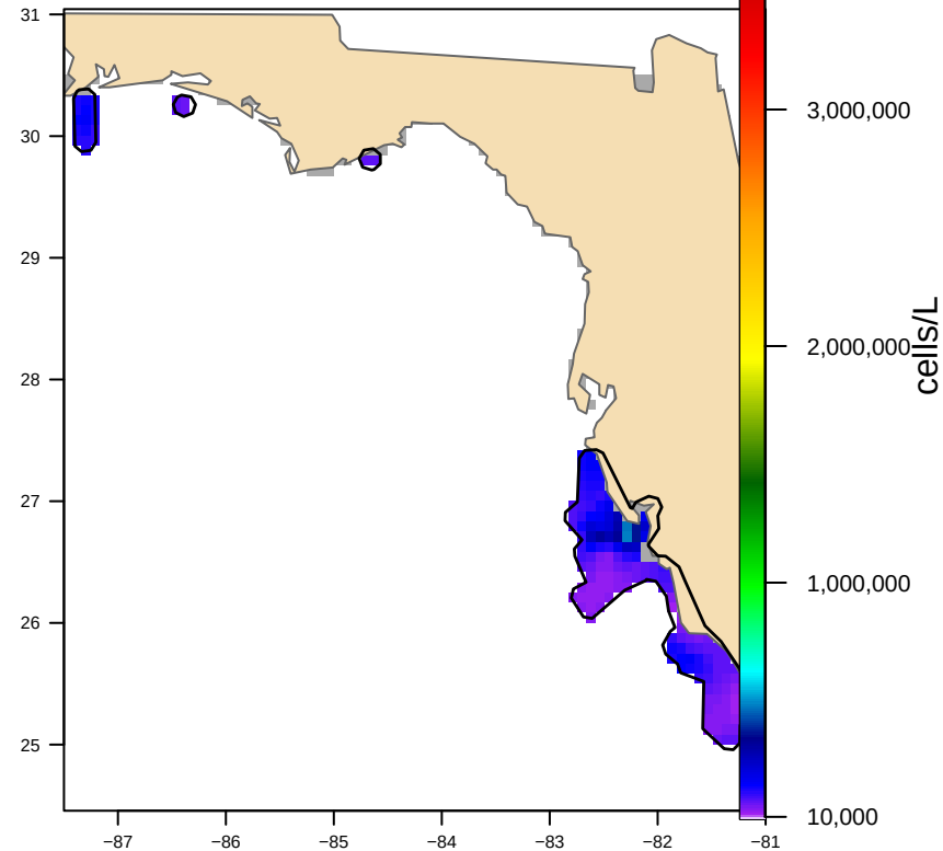
Hull-clipped (4 footprint(s), 16,300 km 2 ) bloom area 13,829 km 2
