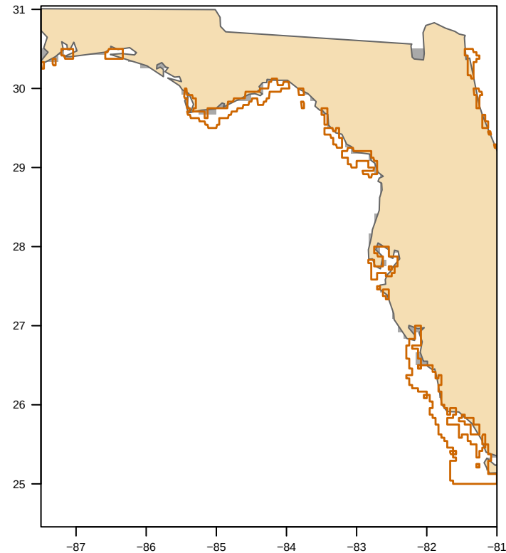
MODIS nFLH-clipped (27 polygon(s)) bloom area 0 km 2
