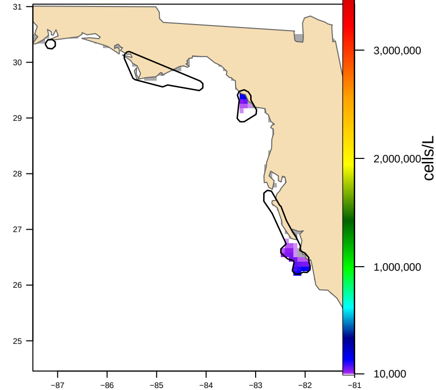
Hull-clipped (4 footprint(s), 12,438 km 2 ) bloom area 2,739 km 2
