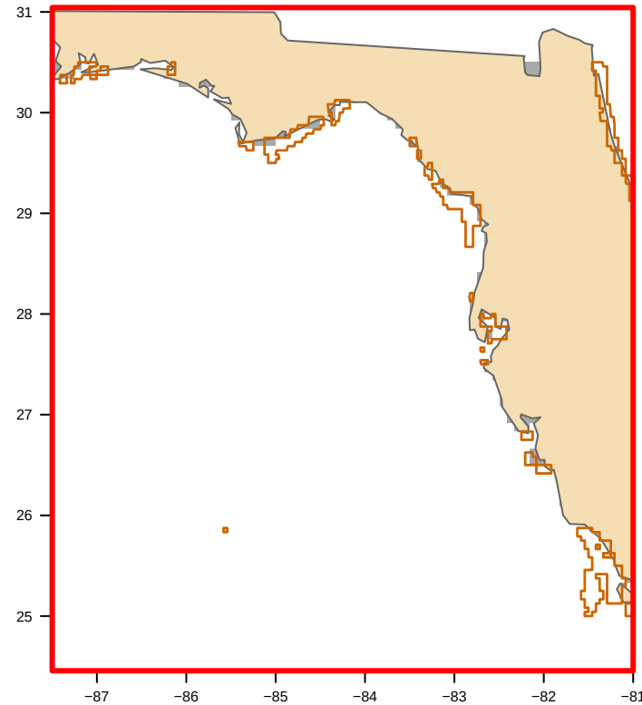
USED: MODIS nFLH-clipped (26 polygon(s)) bloom area 0 km2
