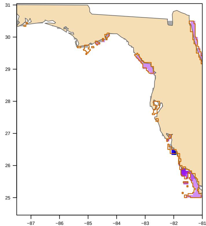
MODIS nFLH-clipped (22 polygon(s)) bloom area 6,373 km 2
