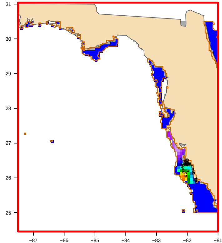
USED: MODIS nFLH-clipped (29 polygon(s)) bloom area 22,888 km 2
