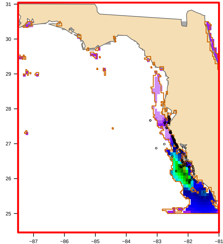
USED: MODIS nFLH-clipped (38 polygon(s)) bloom area 23,519 km 2
