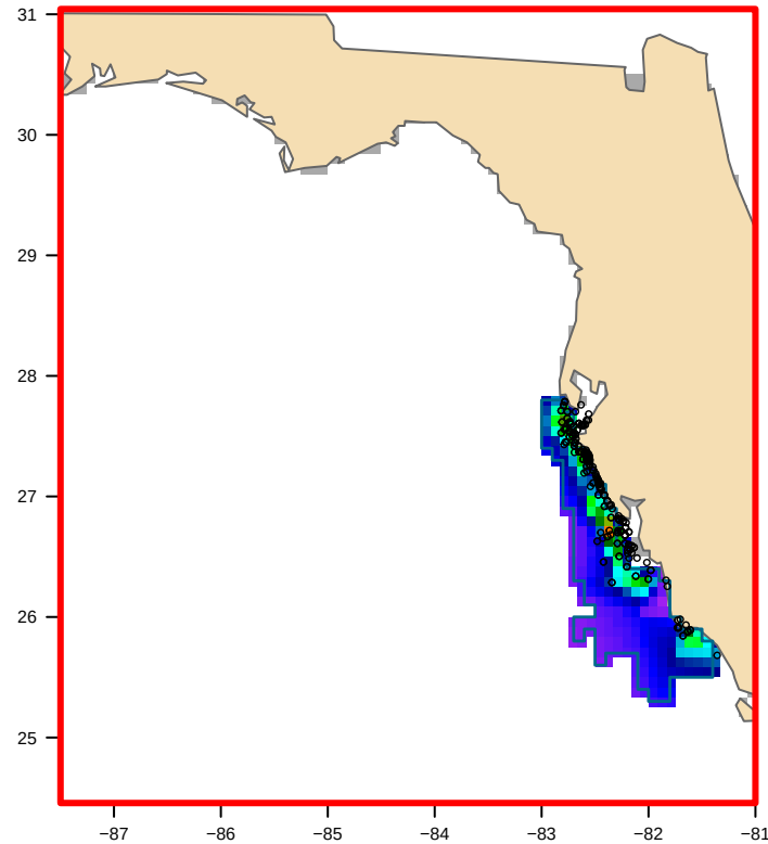
USED: VIIRS-clipped (132 positive VIIRS cells) bloom area 17,557 km 2
