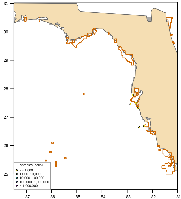
Unclipped sdmTMB (fitted, converged = TRUE) bloom area 0 km2, max 913 cells/L
