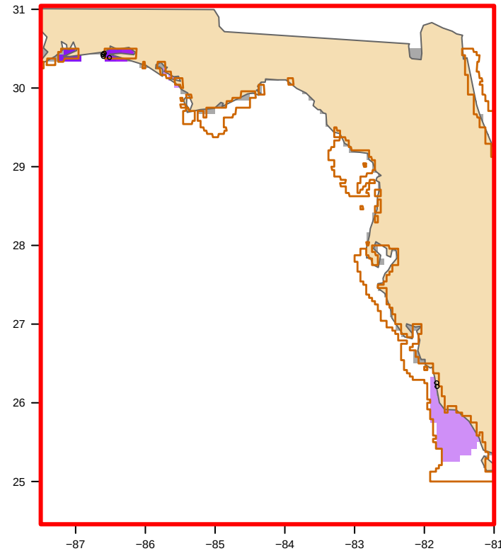
USED: MODIS nFLH-clipped (26 polygon(s)) bloom area 5,723 km 2
