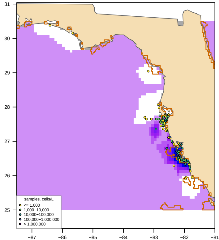
Unclipped sdmTMB (fitted, converged = TRUE) bloom area 268,807 km 2 , max 752,799 cells/L
