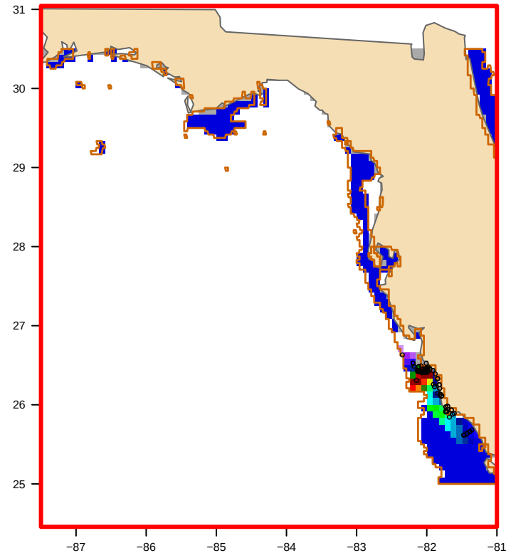
USED: MODIS nFLH-clipped (30 polygon(s)) bloom area 23,115 km 2
