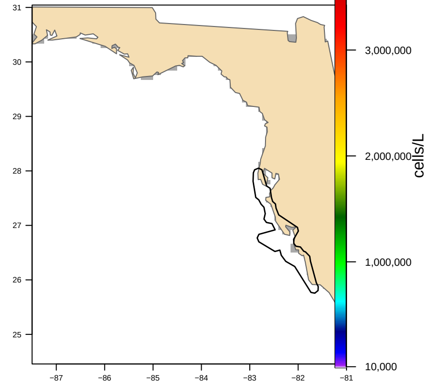
Hull-clipped (1 footprint(s), 9,856 km 2 ) bloom area 0 km 2
