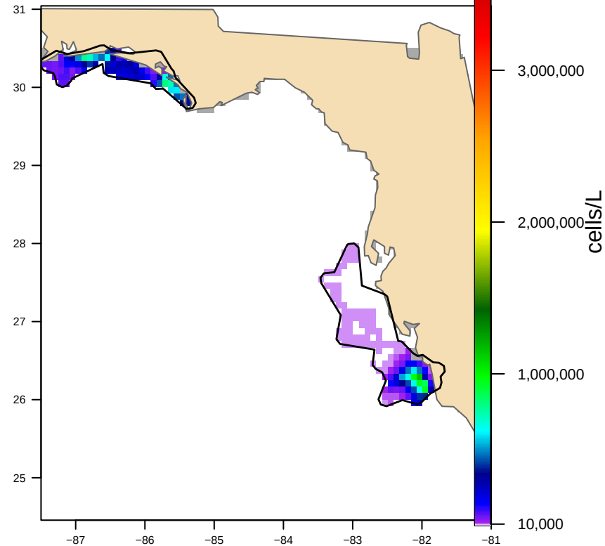
Hull-clipped (2 footprint(s), 23,262 km 2 ) bloom area 15,627 km 2
