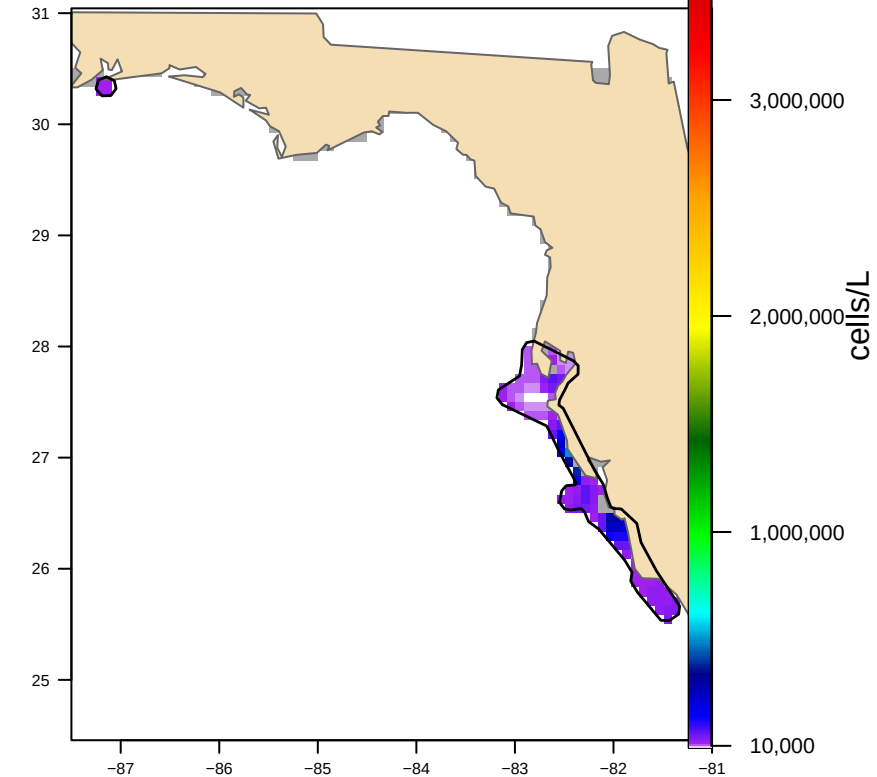
Hull-clipped (2 footprint(s), 10,744 km 2 ) bloom area 7,697 km 2
