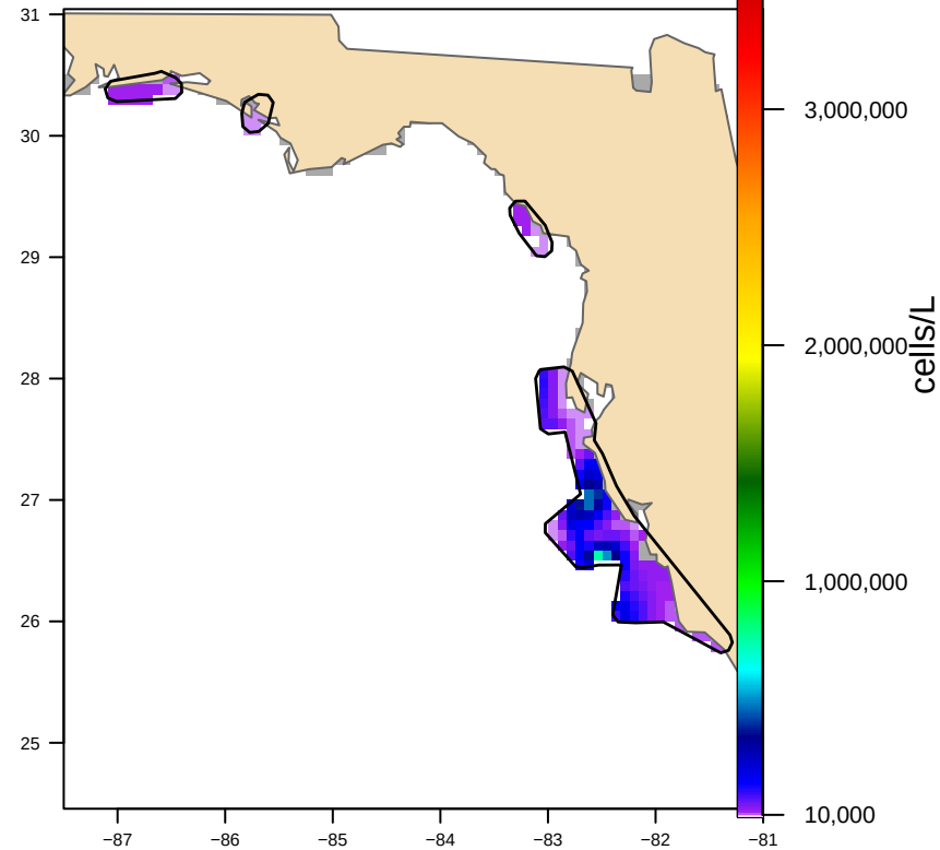
Hull-clipped (4 footprint(s), 17,889 km 2 ) bloom area 13,060 km 2
