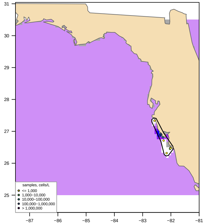
Unclipped sdmTMB (fitted, converged = TRUE) bloom area 289,525 km2, max 396,991 cells/L
