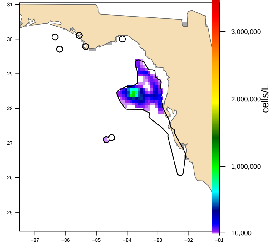
Hull-clipped (7 footprint(s), 24,250 km 2 ) bloom area 13,310 km 2
