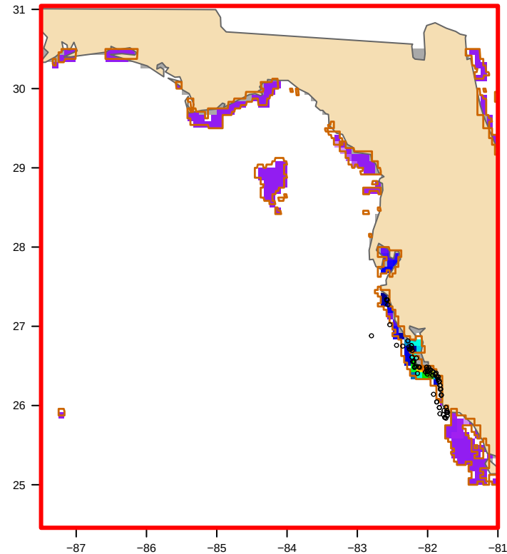
USED: MODIS nFLH-clipped (37 polygon(s)) bloom area 14,042 km 2
