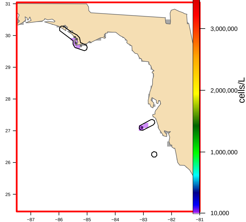
USED: Hull-clipped (3 footprint(s), 4,206 km 2 ) bloom area 1,352 km 2
