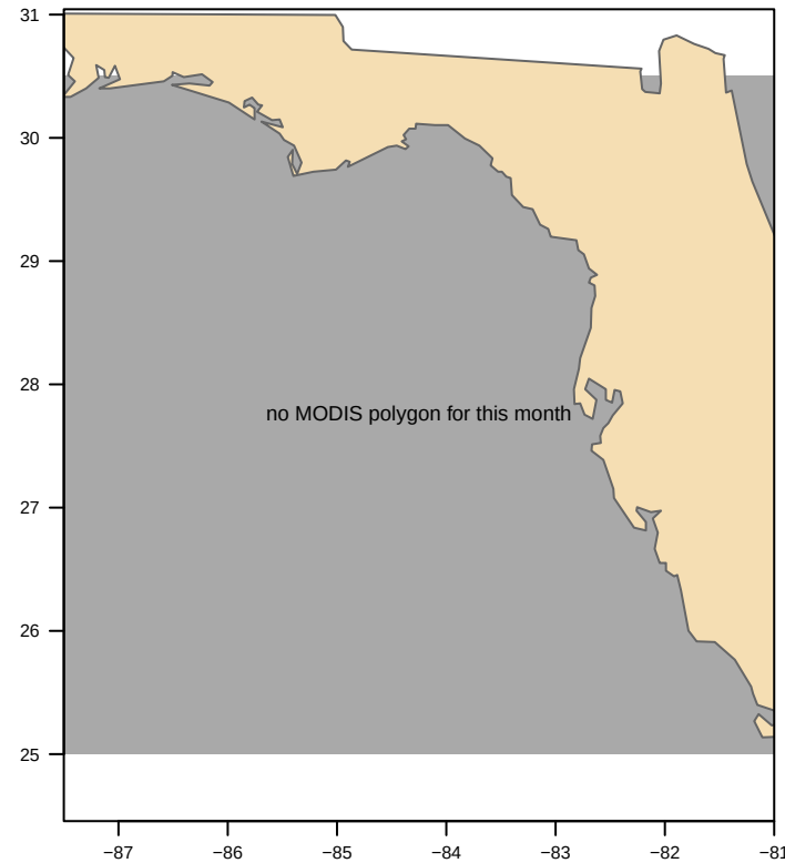
MODIS nFLH-clipped
