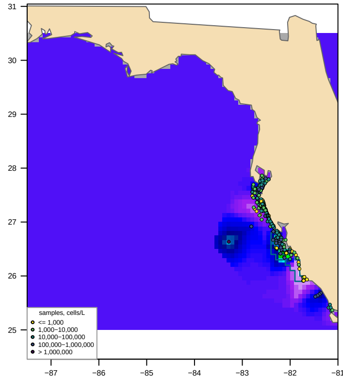
Unclipped sdmTMB (fitted, converged = TRUE) bloom area 291,207 km 2 , max 1,423,496 cells/L
