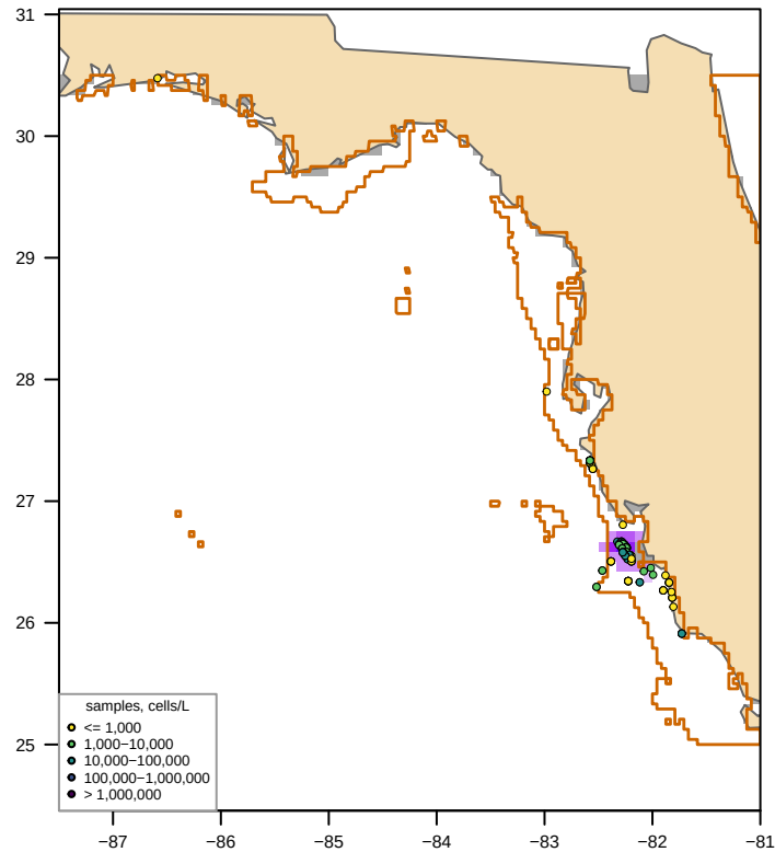
Unclipped sdmTMB (fitted, converged = TRUE) bloom area 1,147 km 2 , max 71,739 cells/L
