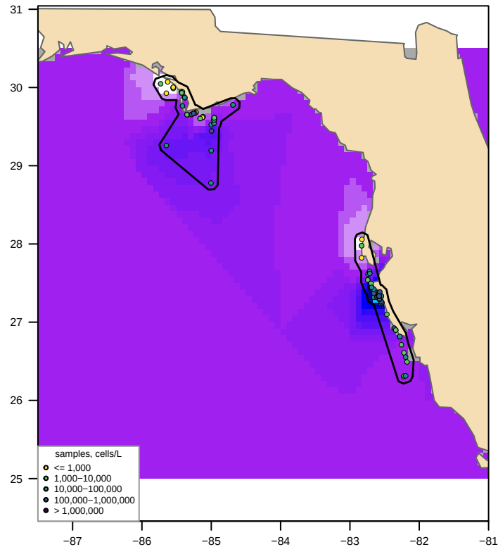
Unclipped sdmTMB (fitted, converged = TRUE) bloom area 290,395 km 2 , max 630,438 cells/L
