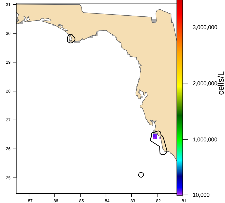
Hull-clipped (3 footprint(s), 4,242 km 2 ) bloom area 383 km 2
