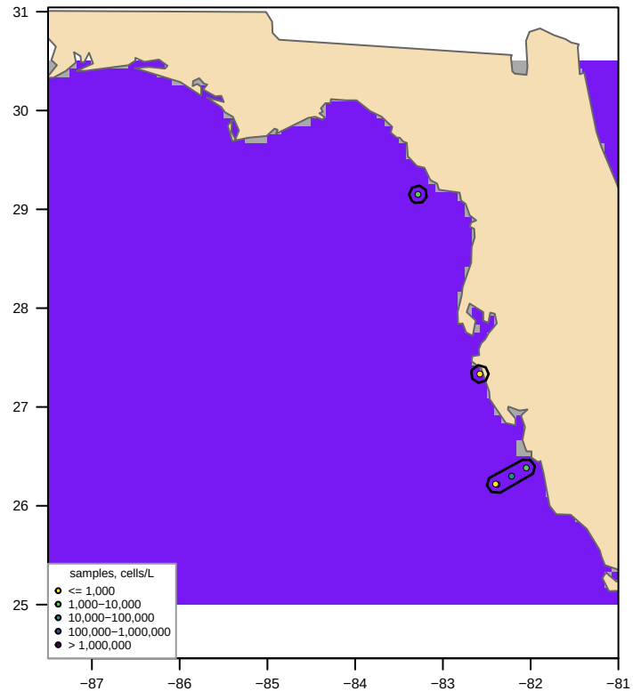
Unclipped sdmTMB (fitted, converged = TRUE) bloom area 291,361 km 2 , max 64,582 cells/L
