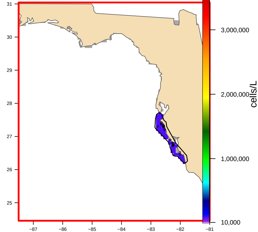
USED: Hull-clipped (1 footprint(s), 5,250 km 2 ) bloom area 3,812 km 2
