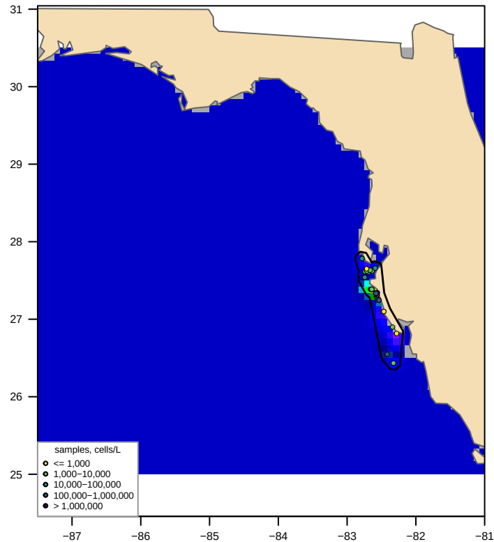
Unclipped sdmTMB (fitted, converged = TRUE) bloom area 291,361 km 2 , max 2,128,102 cells/L
