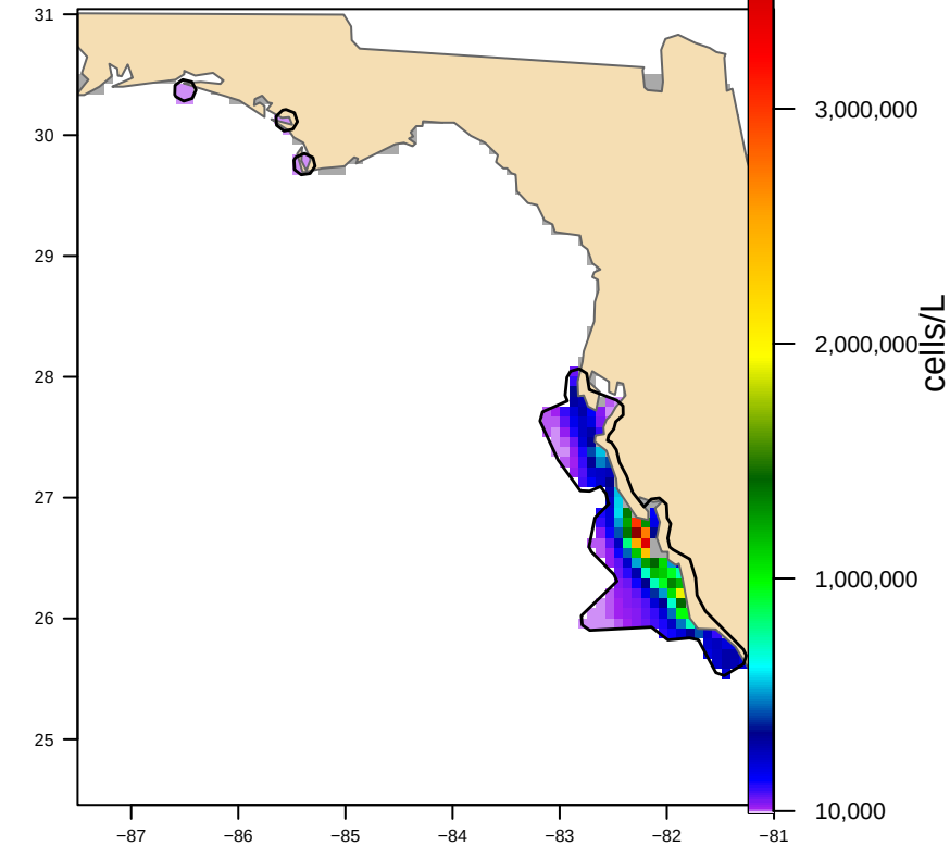
Hull-clipped (4 footprint(s), 18,284 km 2 ) bloom area 14,804 km 2
