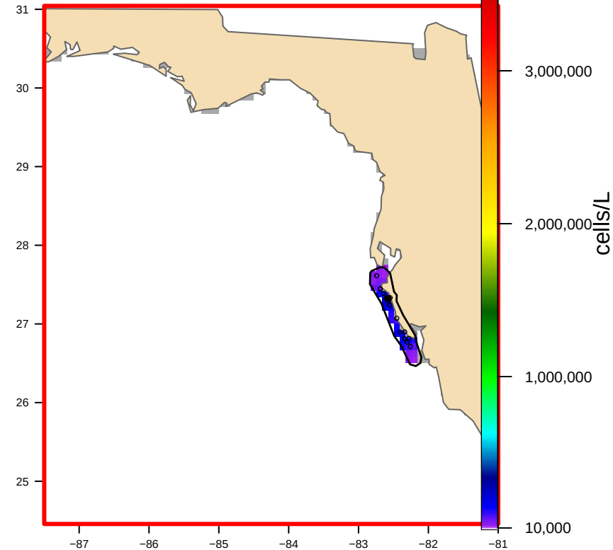
USED: Hull-clipped (1 footprint(s), 3,552 km 2 ) bloom area 2,512 km 2
