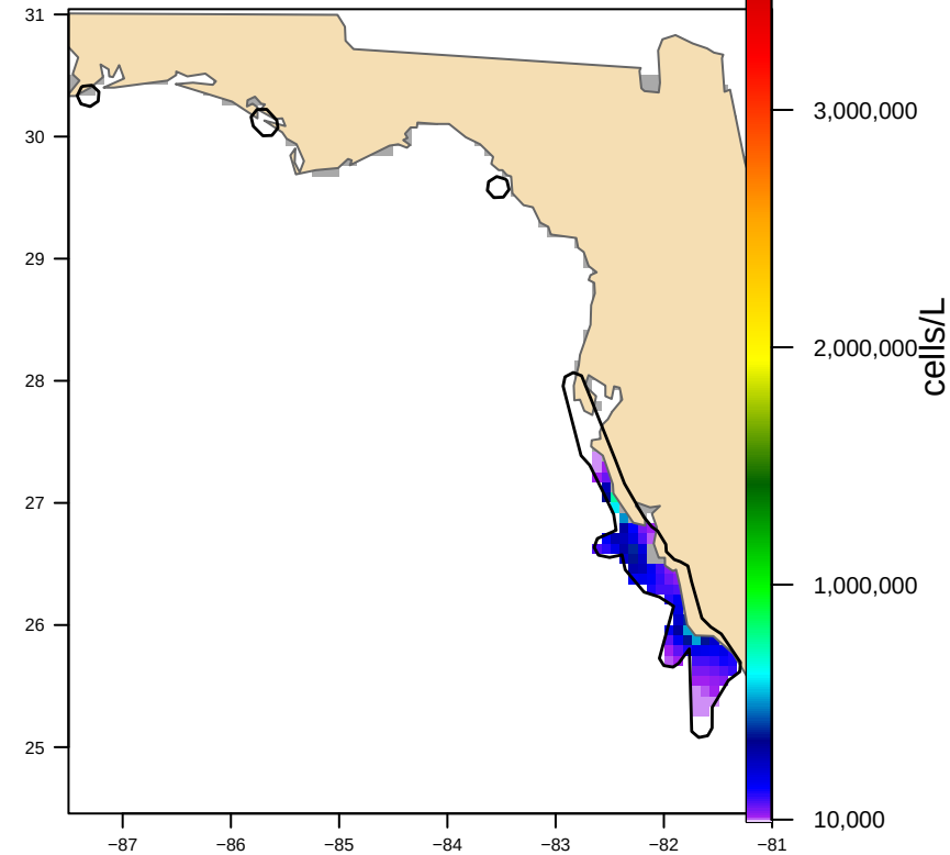
Hull-clipped (4 footprint(s), 12,713 km 2 ) bloom area 7,061 km 2
