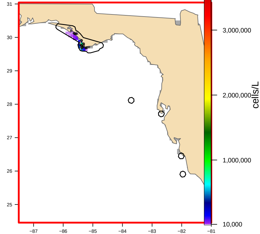
USED: Hull-clipped (5 footprint(s), 6,767 km 2 ) bloom area 1,705 km 2
