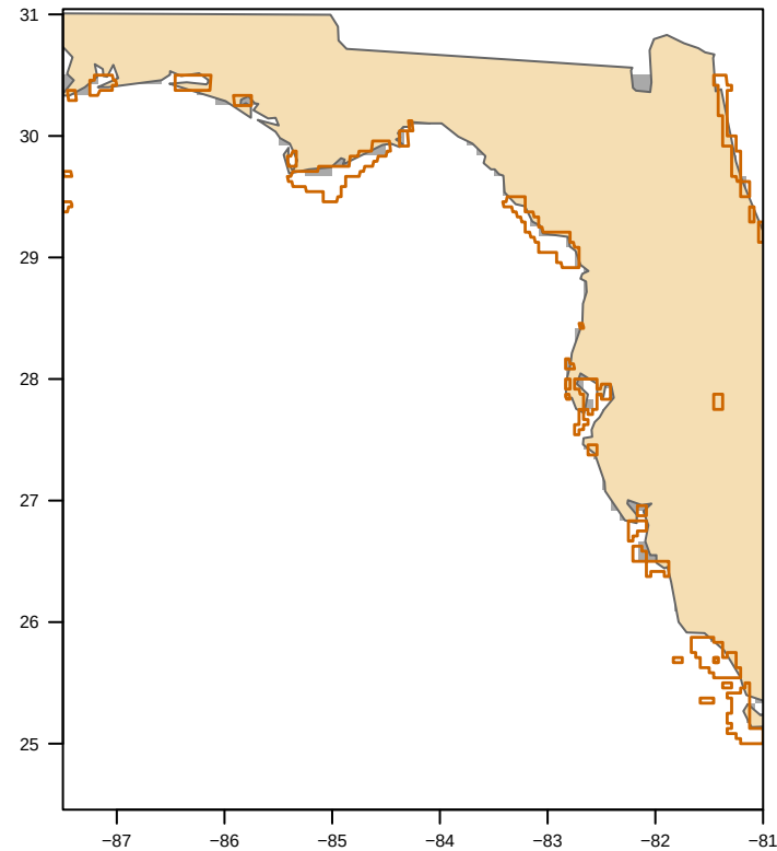
MODIS nFLH-clipped (33 polygon(s)) bloom area 0 km 2
