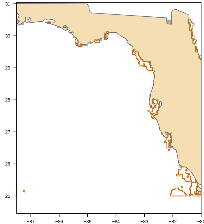
MODIS nFLH-clipped (28 polygon(s)) bloom area 0 km 2
