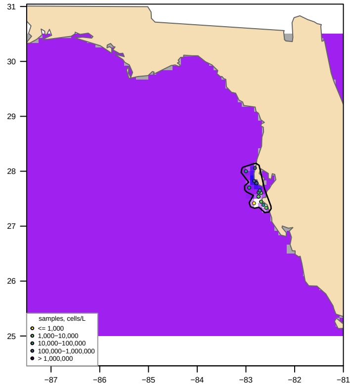
Unclipped sdmTMB (fitted, converged = TRUE) bloom area 291,057 km2, max 378,921 cells/L
