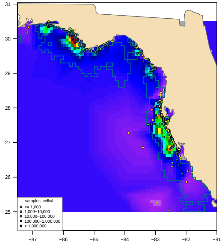
Unclipped sdmTMB (fitted, converged = TRUE) bloom area 291,361 km 2 , max 7,636,488 cells/L
