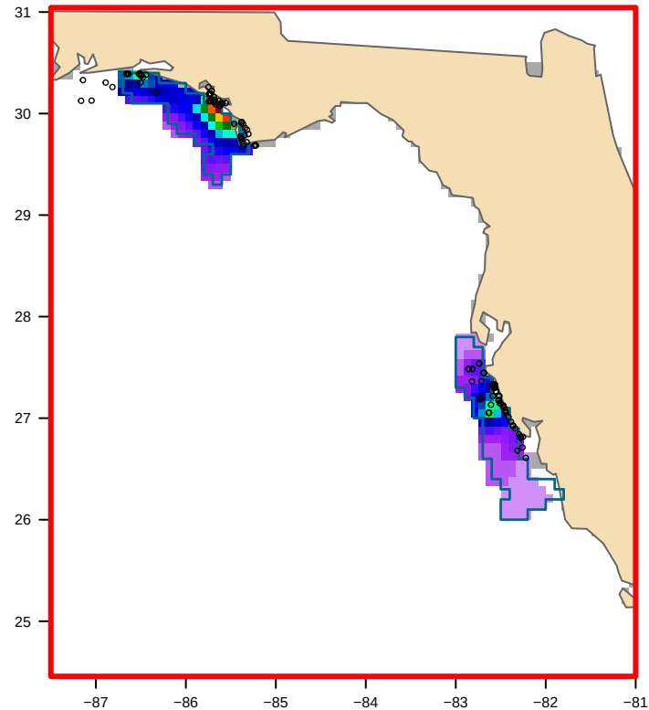
USED: VIIRS-clipped (123 positive VIIRS cells) bloom area 16,484 km 2
