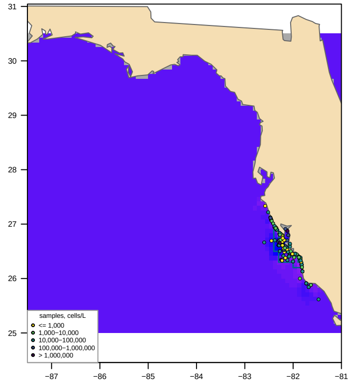
Unclipped sdmTMB (fitted, converged = TRUE) bloom area 291,361 km 2 , max 328,675 cells/L
