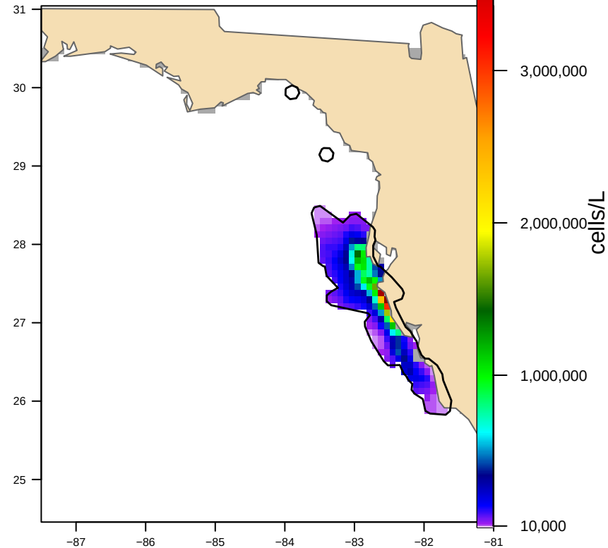
Hull-clipped (3 footprint(s), 20,103 km 2 ) bloom area 16,569 km 2
