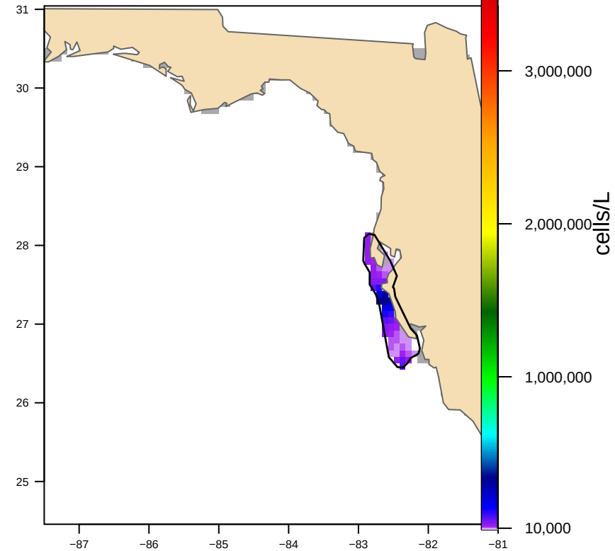
Hull-clipped (1 footprint(s), 6,309 km 2 ) bloom area 4,337 km 2
