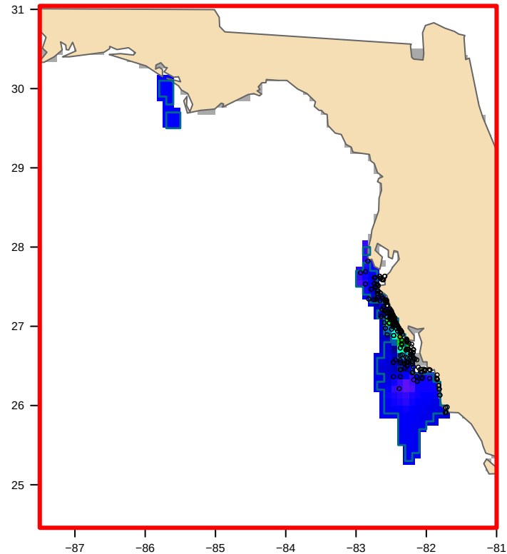
USED: VIIRS-clipped (104 positive VIIRS cells) bloom area 15,494 km 2
