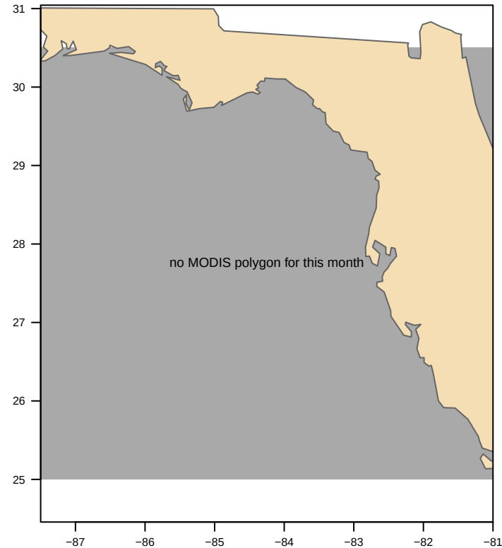
MODIS nFLH-clipped
