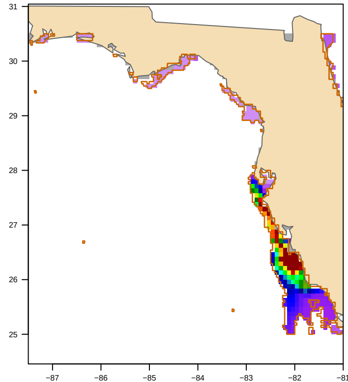
MODIS nFLH-clipped (26 polygon(s)) bloom area 19,808 km 2
