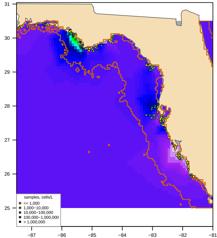
Unclipped sdmTMB (fitted, converged = TRUE) bloom area 291,208 km 2 , max 1,741,901 cells/L
