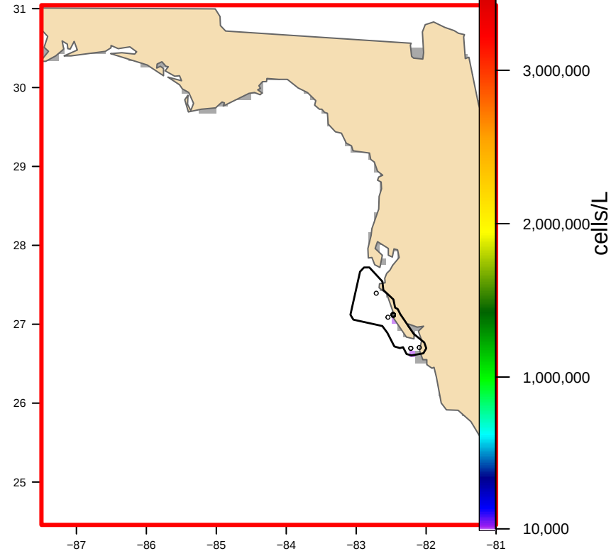
USED: Hull-clipped (1 footprint(s), 5,439 km 2 ) bloom area 153 km 2
