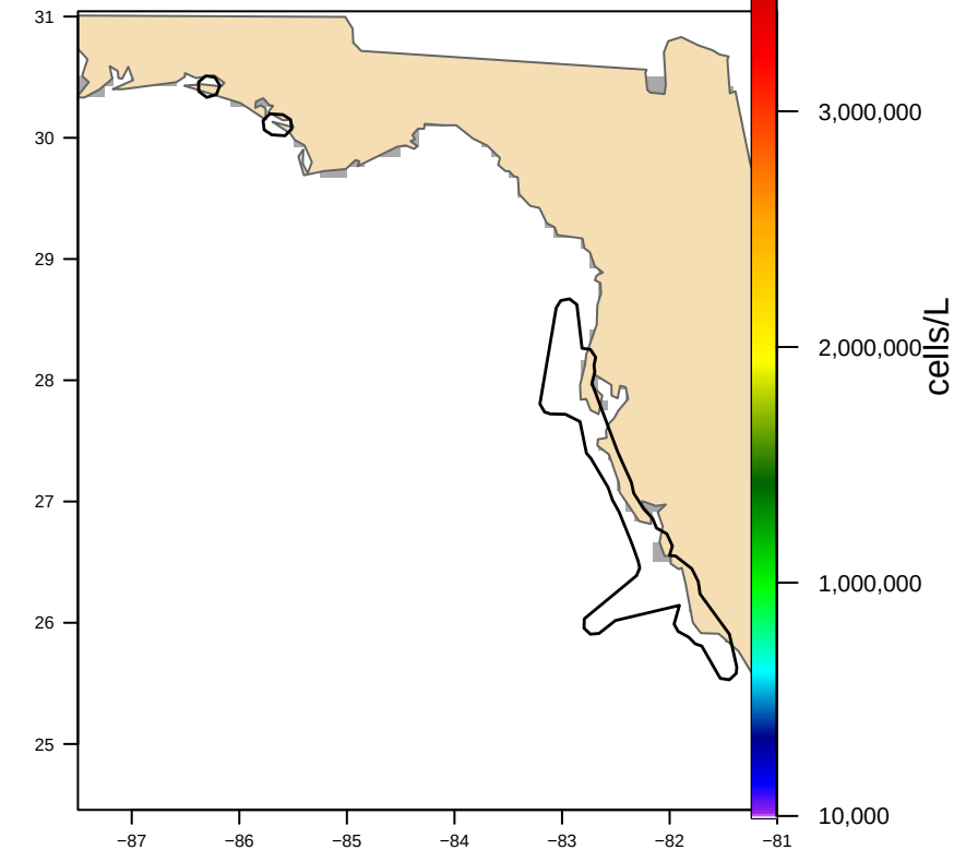
Hull-clipped (3 footprint(s), 14,326 km 2 ) bloom area 0 km 2
