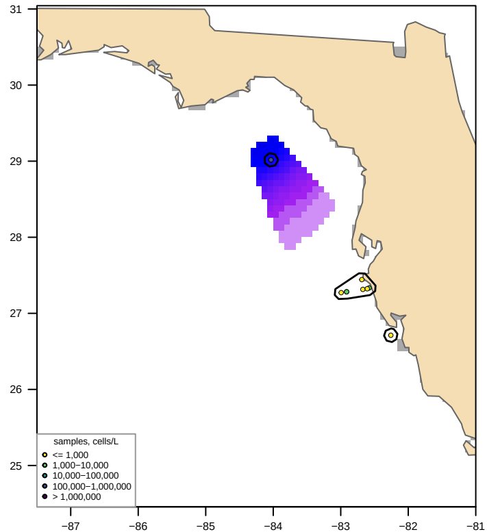
Unclipped sdmTMB (fitted, converged = TRUE) bloom area 11,117 km2, max 188,198 cells/L
