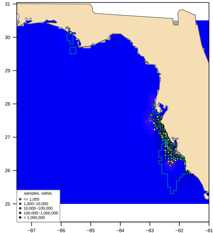
Unclipped sdmTMB (fitted, converged = TRUE) bloom area 291,361 km 2 , max 1,705,330 cells/L
