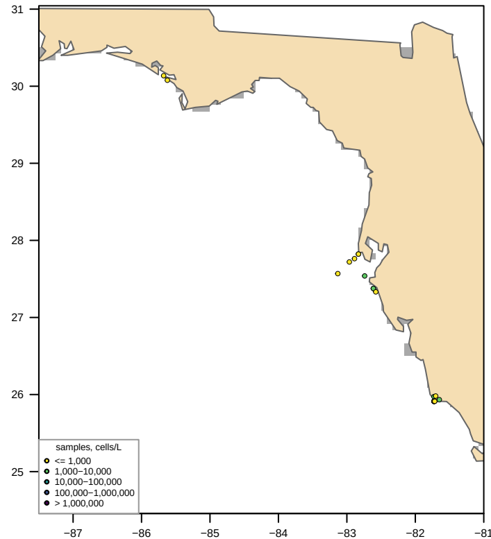
Unclipped sdmTMB (fitted, converged = TRUE) bloom area 0 km 2 , max 1,520 cells/L
