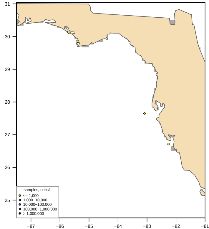
Unclipped sdmTMB (fitted, converged = TRUE) bloom area 0 km 2 , max 540 cells/L
