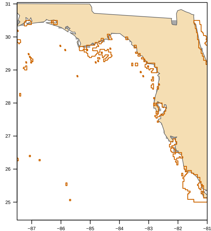
MODIS nFLH-clipped (61 polygon(s)) bloom area 0 km 2
