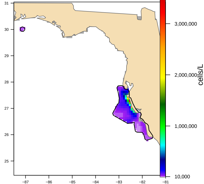
Hull-clipped (2 footprint(s), 14,920 km 2 ) bloom area 12,888 km 2
