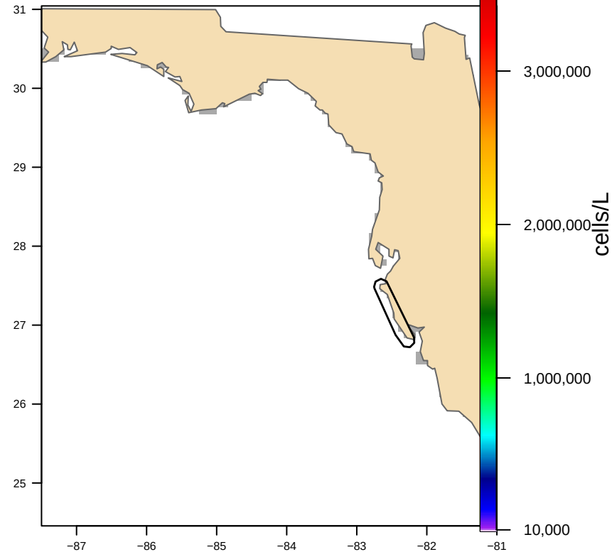
Hull-clipped (1 footprint(s), 2,164 km2) bloom area 0 km2
