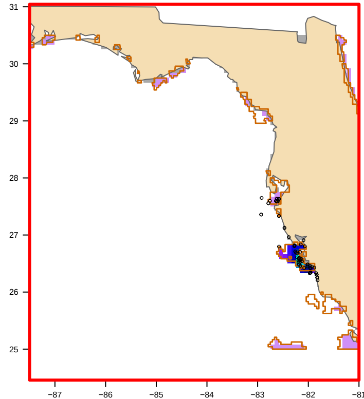
USED: MODIS nFLH-clipped (29 polygon(s)) bloom area 6,671 km 2
