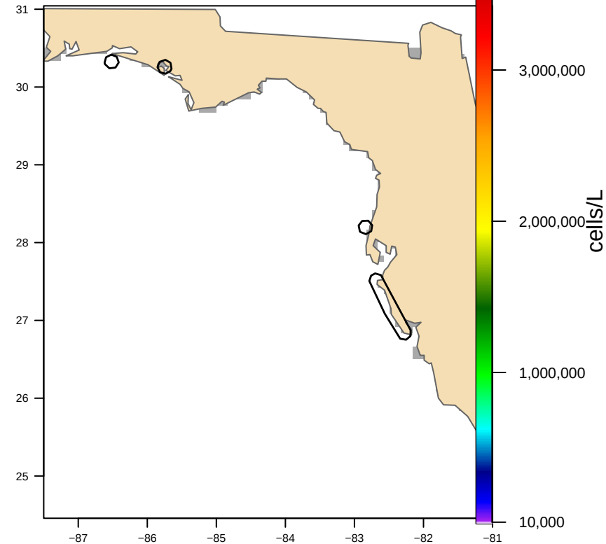
Hull-clipped (4 footprint(s), 3,013 km2) bloom area 0 km2
