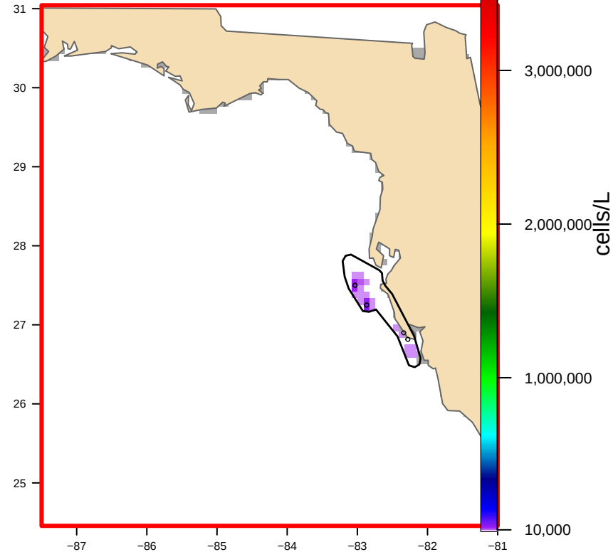
USED: Hull-clipped (1 footprint(s), 5,727 km 2 ) bloom area 1,597 km 2
