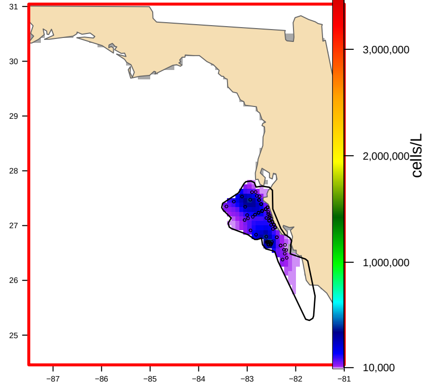
USED: Hull-clipped (1 footprint(s), 17,144 km 2 ) bloom area 12,195 km 2
