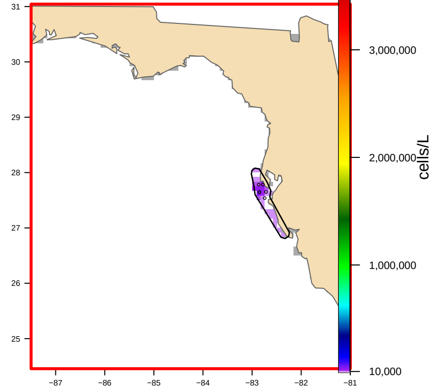
USED: Hull-clipped (1 footprint(s), 3,561 km2) bloom area 2,124 km2
