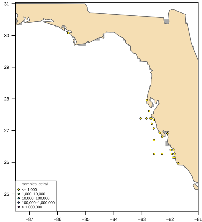
Unclipped sdmTMB (fitted, converged = TRUE) bloom area 0 km 2 , max 526 cells/L
