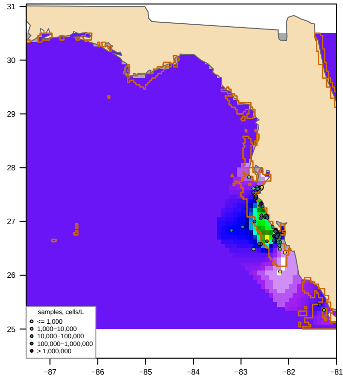
Unclipped sdmTMB (fitted, converged = TRUE) bloom area 290,902 km 2 , max 2,112,130 cells/L
