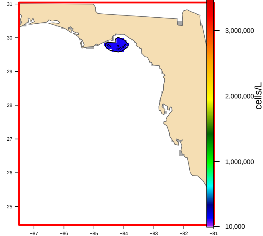
USED: Hull-clipped (1 footprint(s), 2,292 km 2 ) bloom area 2,228 km 2
