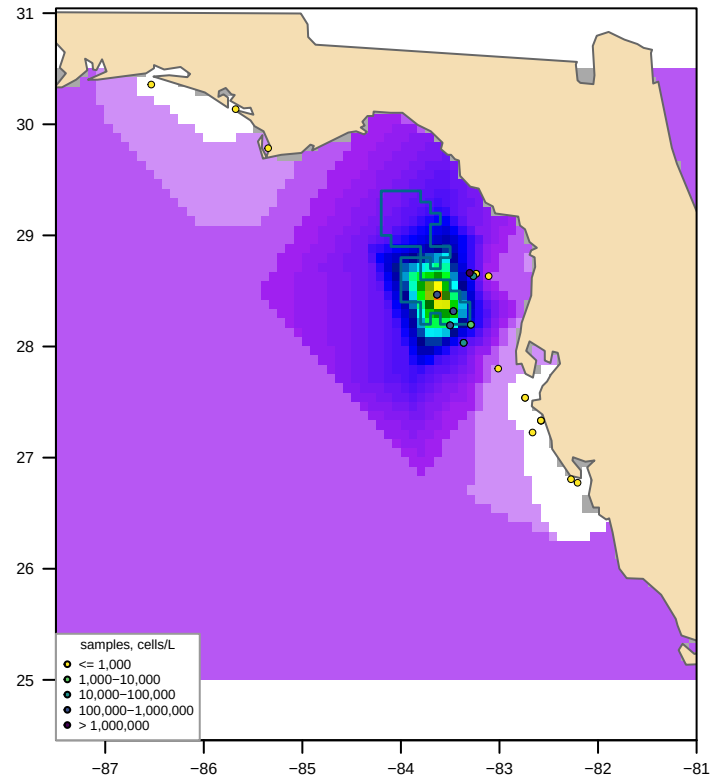
Unclipped sdmTMB (fitted, converged = TRUE) bloom area 280,205 km 2 , max 2,765,506 cells/L
