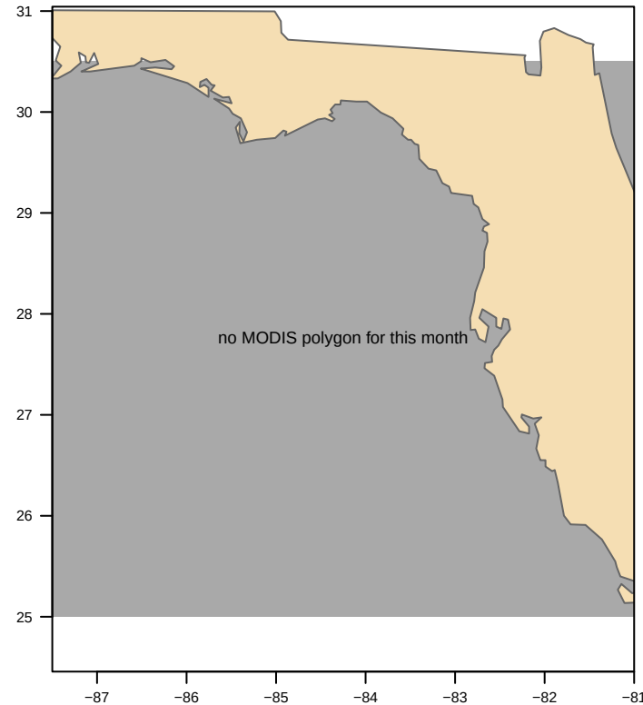
MODIS nFLH-clipped
