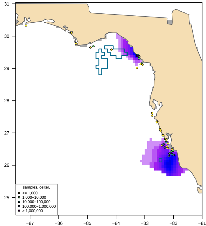
Unclipped sdmTMB (fitted, converged = TRUE) bloom area 16,378 km 2 , max 226,387 cells/L
