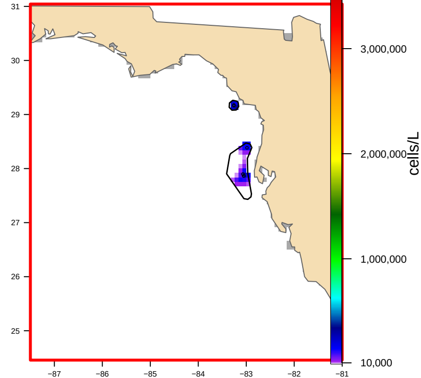
USED: Hull-clipped (2 footprint(s), 4,199 km 2 ) bloom area 2,338 km 2
