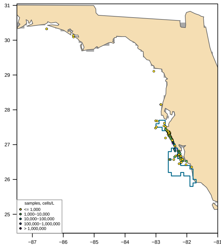
Unclipped sdmTMB (fitted, converged = TRUE) bloom area 152 km 2 , max 17,329 cells/L
