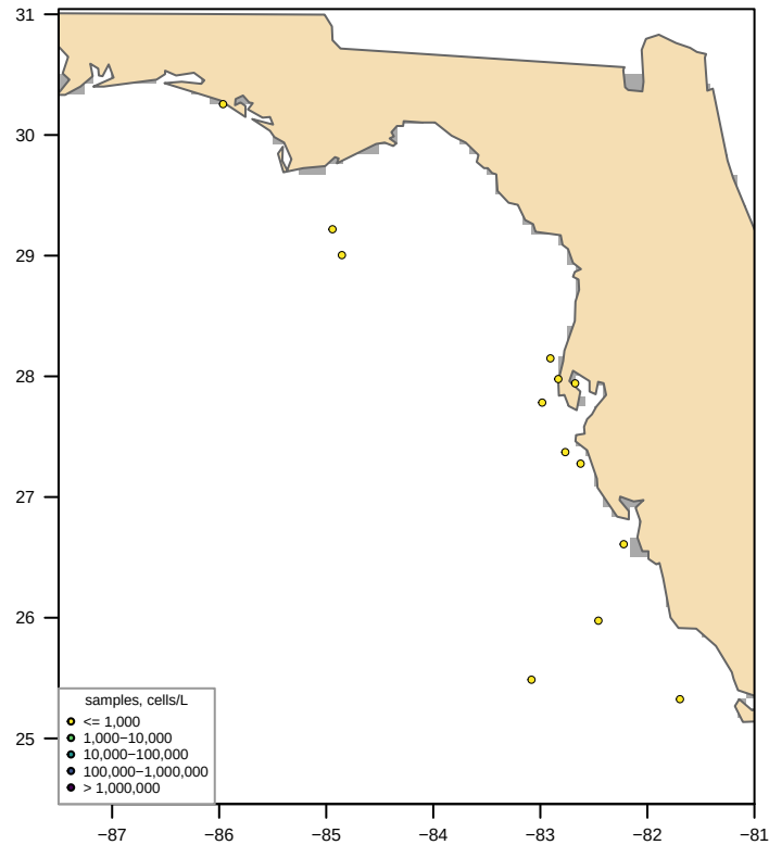
Unclipped sdmTMB (fitted, converged = TRUE) bloom area 0 km 2 , max 420 cells/L
