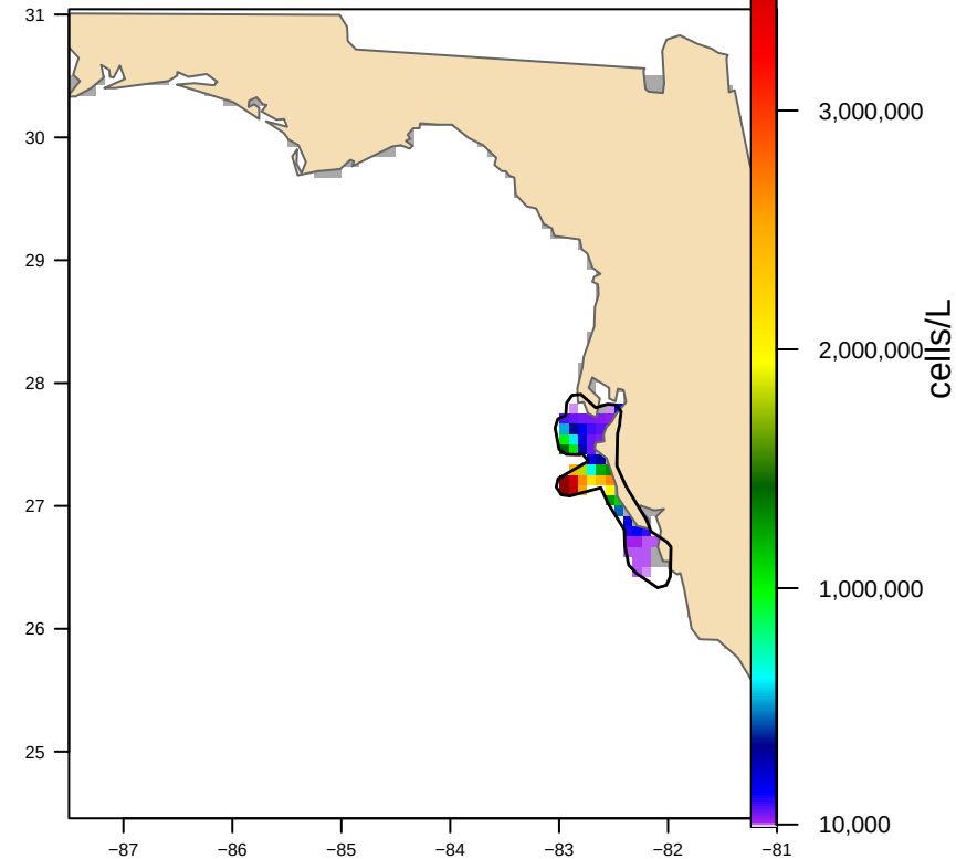
Hull-clipped (1 footprint(s), 6,732 km 2 ) bloom area 4,487 km 2
