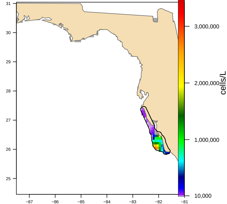
Hull-clipped (1 footprint(s), 6,371 km 2 ) bloom area 4,213 km 2
