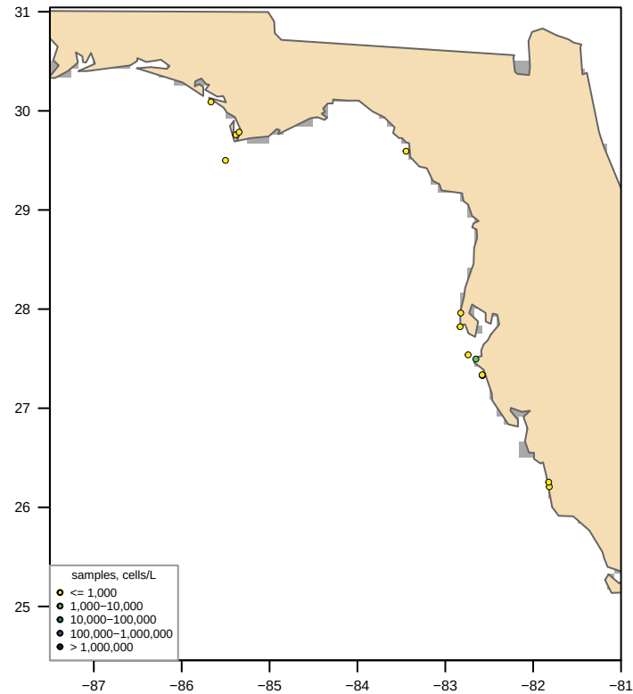
Unclipped sdmTMB (fitted, converged = TRUE) bloom area 0 km 2 , max 1,179 cells/L
