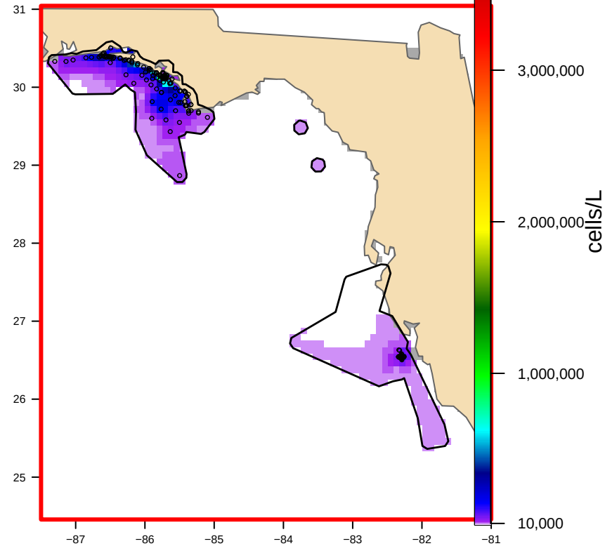
USED: Hull-clipped (4 footprint(s), 38,855 km2) bloom area 28,430 km2
