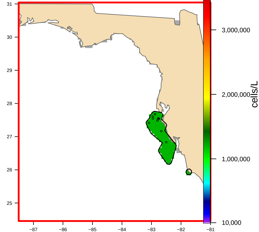
USED: Hull-clipped (2 footprint(s), 8,564 km 2 ) bloom area 8,310 km 2
