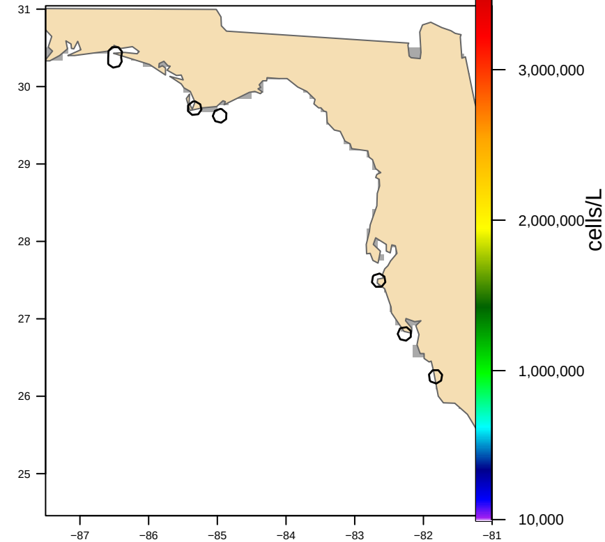
Hull-clipped (6 footprint(s), 2,085 km 2 ) bloom area 0 km 2
