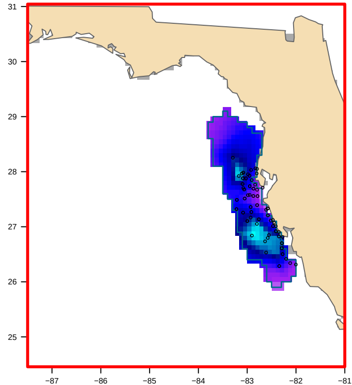
USED: VIIRS-clipped (232 positive VIIRS cells) bloom area 28,437 km 2
