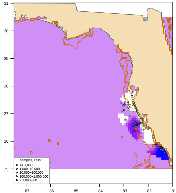
Unclipped sdmTMB (fitted, converged = TRUE) bloom area 283,731 km 2 , max 165,604 cells/L
