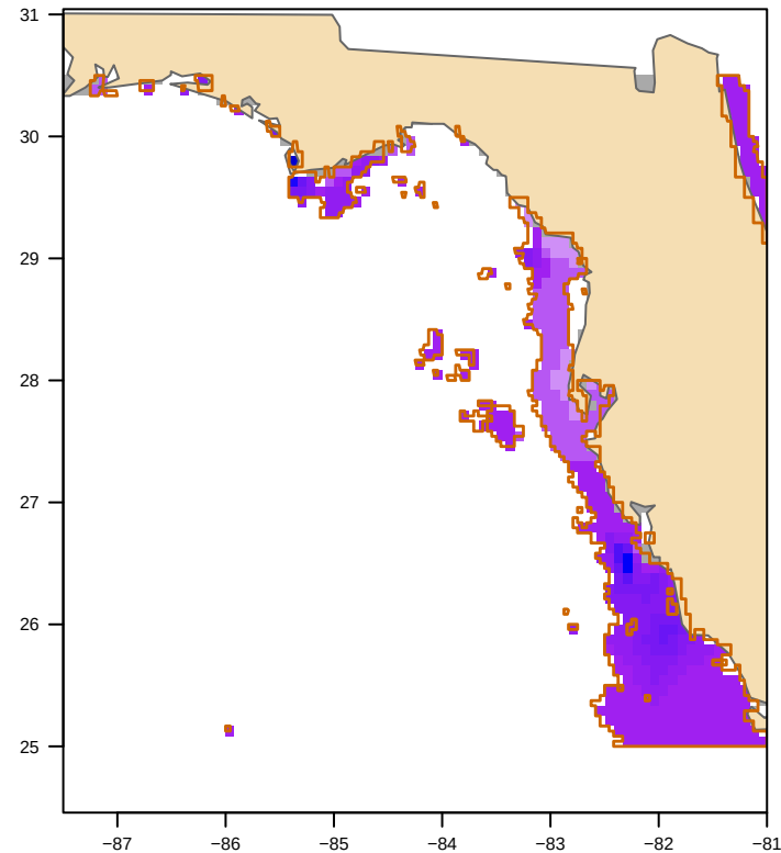
MODIS nFLH-clipped (47 polygon(s)) bloom area 35,295 km 2
