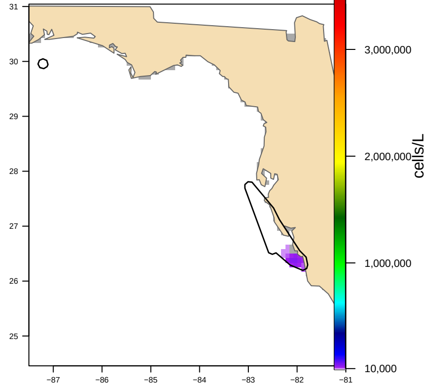
Hull-clipped (2 footprint(s), 8,244 km2) bloom area 1,456 km2
