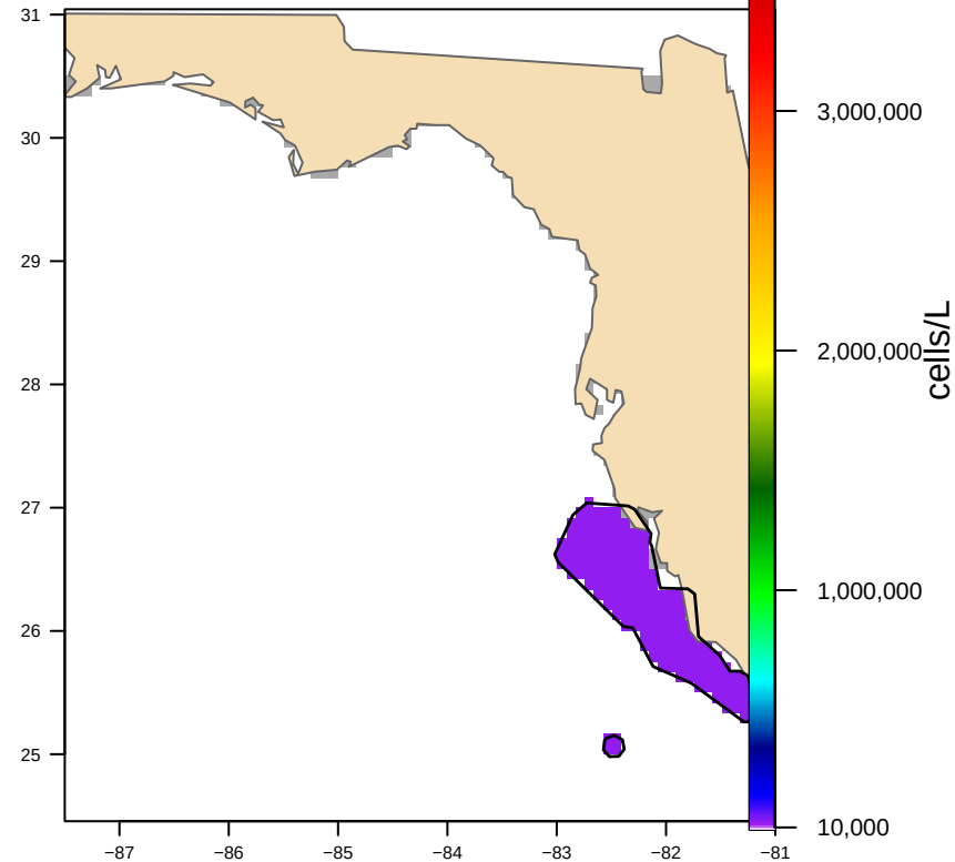
Hull-clipped (2 footprint(s), 13,522 km 2 ) bloom area 12,742 km 2
