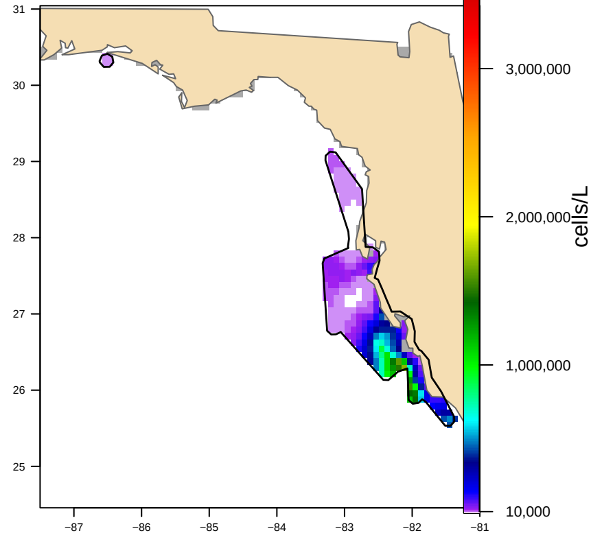
Hull-clipped (2 footprint(s), 24,193 km 2 ) bloom area 19,030 km 2
