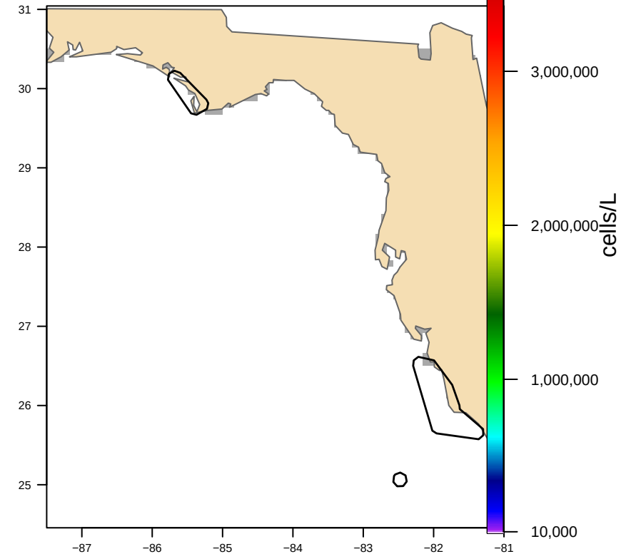
Hull-clipped (3 footprint(s), 7,549 km 2 ) bloom area 0 km 2
