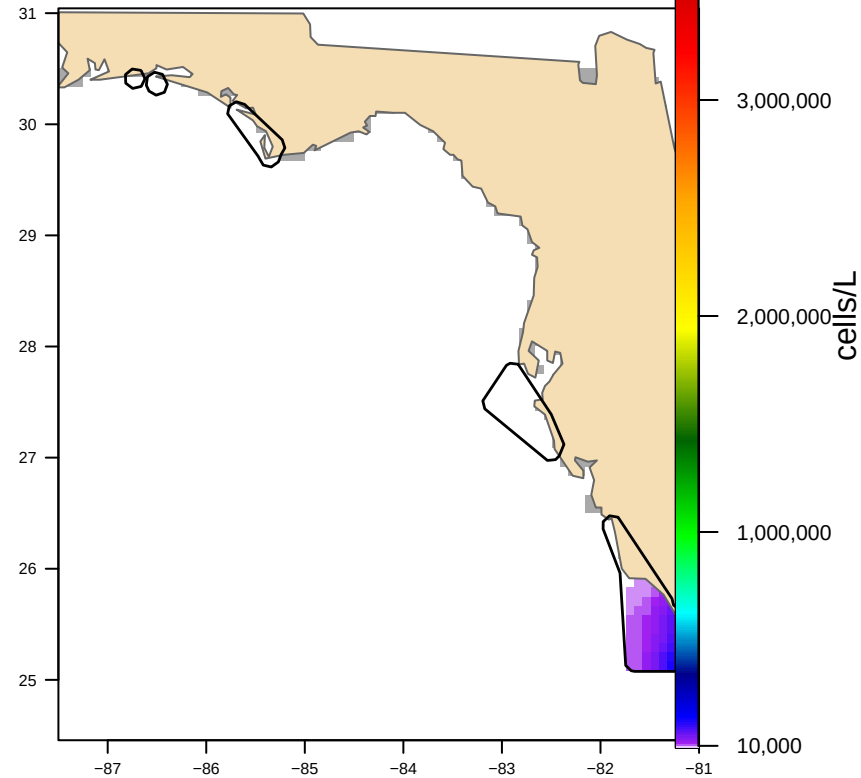
Hull-clipped (5 footprint(s), 14,023 km 2 ) bloom area 5,098 km 2
