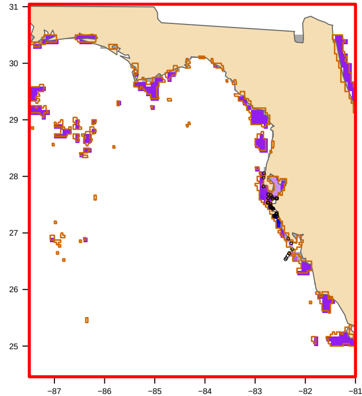
USED: MODIS nFLH-clipped (58 polygon(s)) bloom area 15,493 km 2
