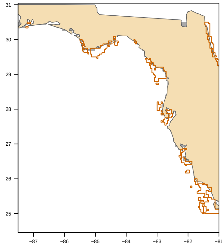
MODIS nFLH-clipped (32 polygon(s)) bloom area 0 km 2
