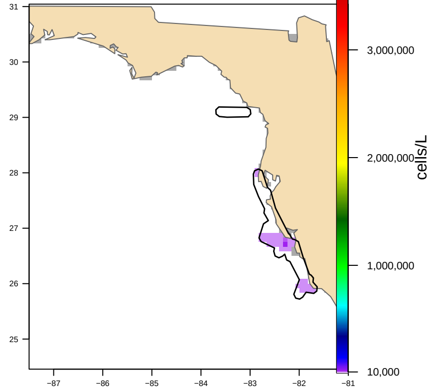
Hull-clipped (2 footprint(s), 10,605 km 2 ) bloom area 2,906 km 2
