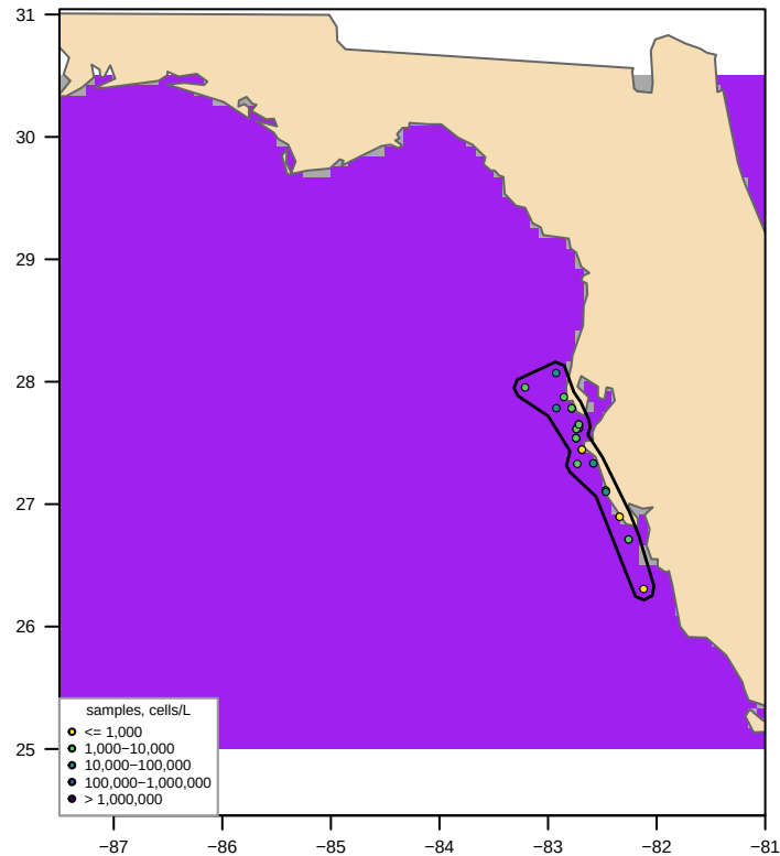
Unclipped sdmTMB (fitted, converged = TRUE) bloom area 291,361 km 2 , max 39,229 cells/L
