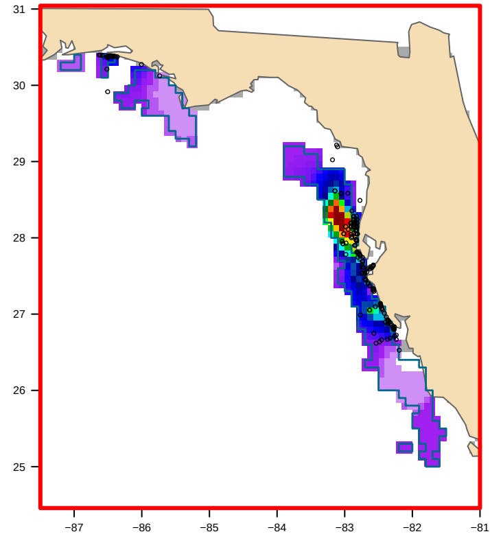
USED: VIIRS-clipped (239 positive VIIRS cells) bloom area 33,308 km 2
