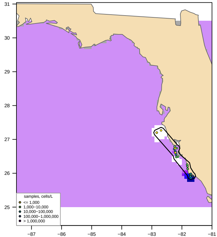
Unclipped sdmTMB (fitted, converged = TRUE) bloom area 288,388 km 2 , max 460,810 cells/L
