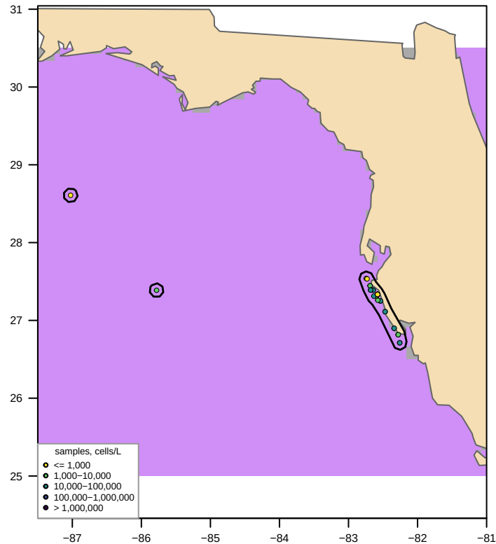
Unclipped sdmTMB (fitted, converged = TRUE) bloom area 291,361 km 2 , max 15,898 cells/L
