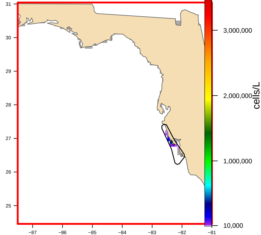
USED: Hull-clipped (1 footprint(s), 3,431 km2) bloom area 686 km2
