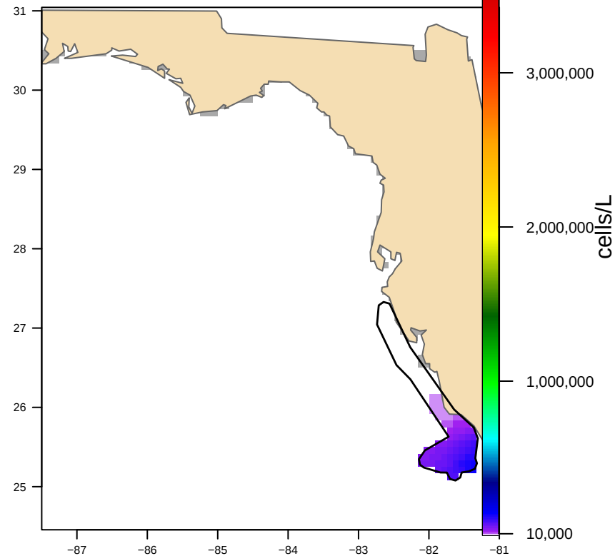
Hull-clipped (1 footprint(s), 9,848 km 2 ) bloom area 5,711 km 2
