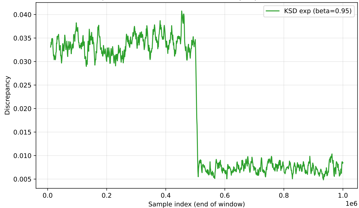
Jackson network KSD over time ( \lambda_1 jumps at T/2 )
