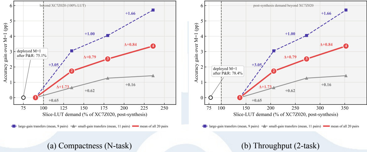
Figure 5.5: Accuracy Gain Versus Post-Synthesis LUT Demand for Multi-Branch Scaling (20 Pairs). Large-Gain Transfers: \Delta_{\text{multi}} = \text{Acc}_{M=4} - \text{Acc}_{M=1} \geq 3 \text{ pp} (9 Pairs); the Remaining 11 Pairs Form the Small-Gain Group.
