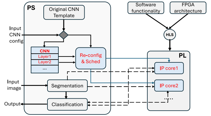
Fig. 1. Proposed acceleration and deployment methodology.
