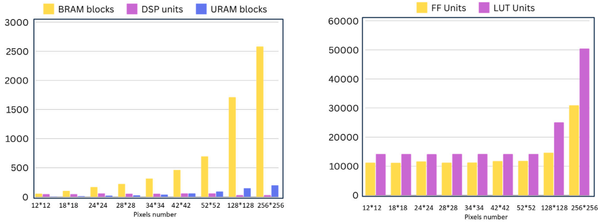
Fig. 7. PL resources utilization following input image size.
