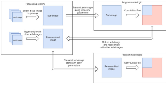
Fig. 3. Multi-module architecture for PL partition.
