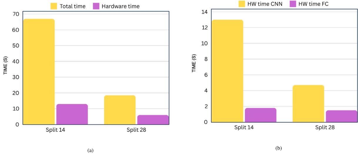
Fig. 5. Analysis of execution and acceleration time.
