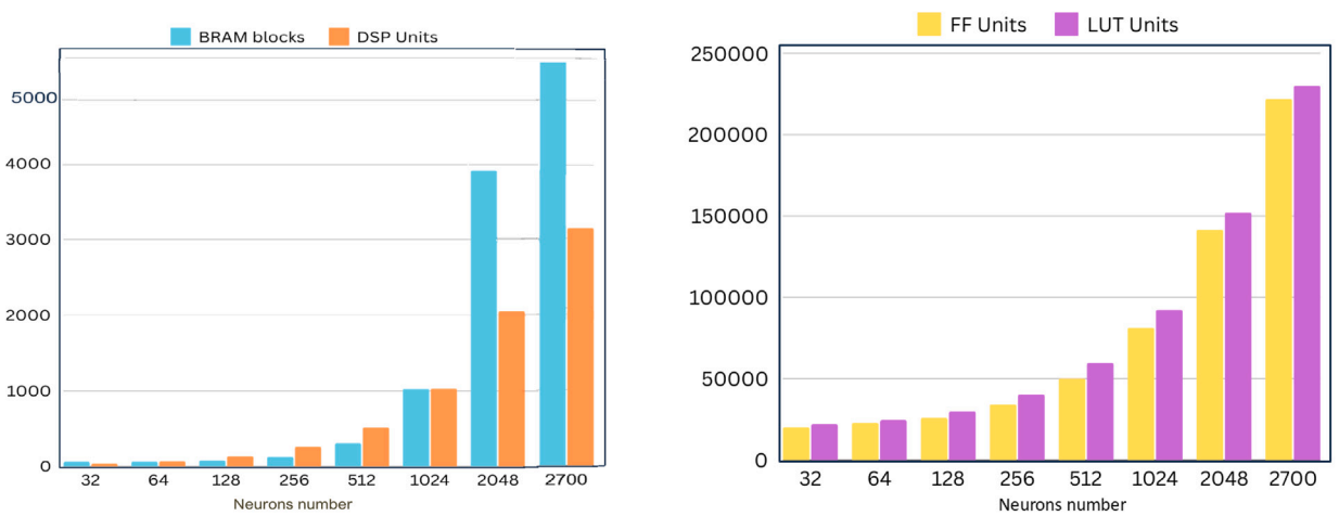
Fig. 6. PL resources utilization and scalability.
