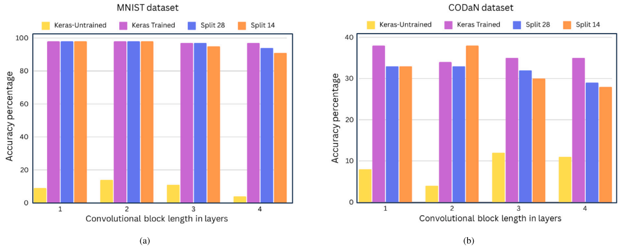
Fig. 4. Accuracy analysis on MNIST and CODaN datasets.
