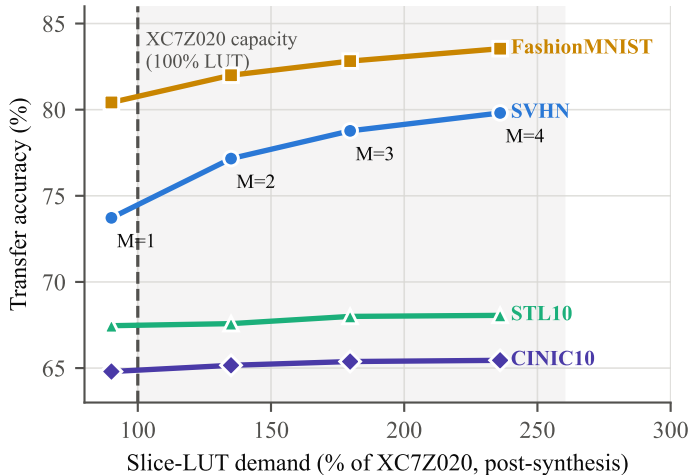
(a) Accuracy vs. resource cost (Compact build)
