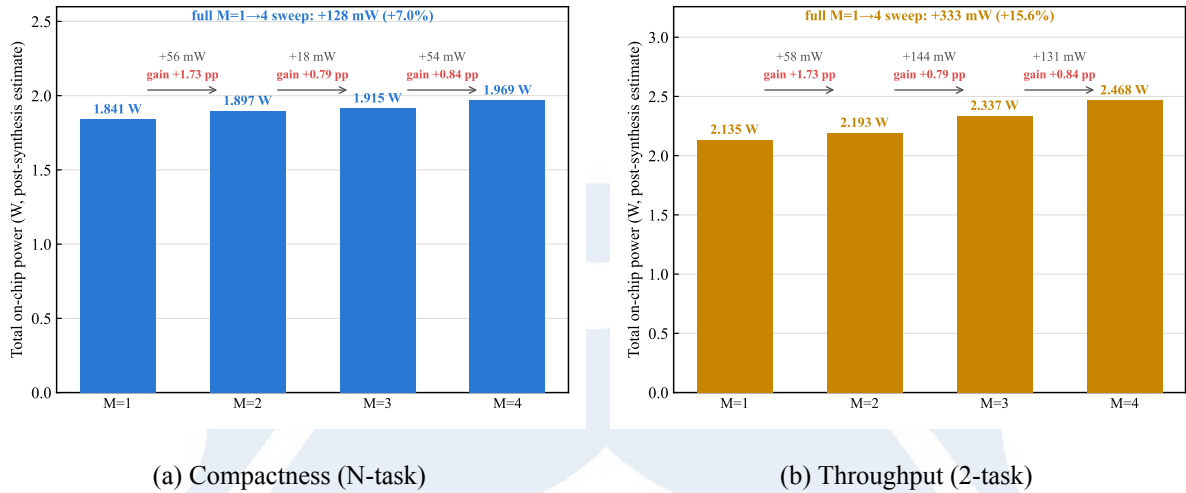
Figure 5.6: Total On-Chip Power Across Branch Counts (Post-Synthesis Estimates).
