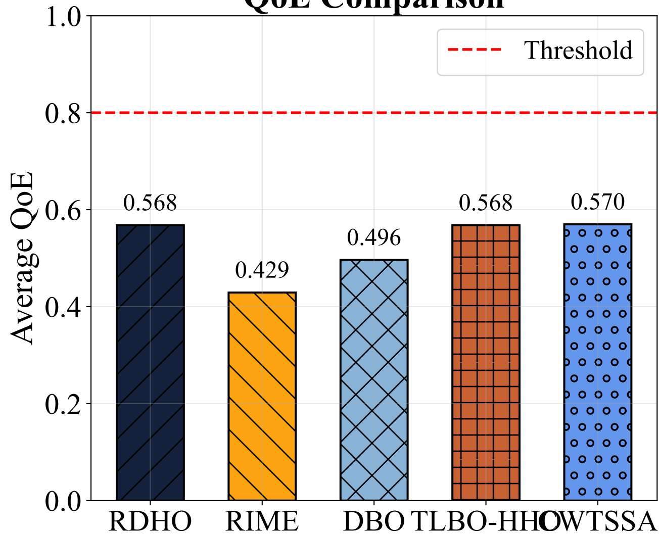
QoE Comparison
