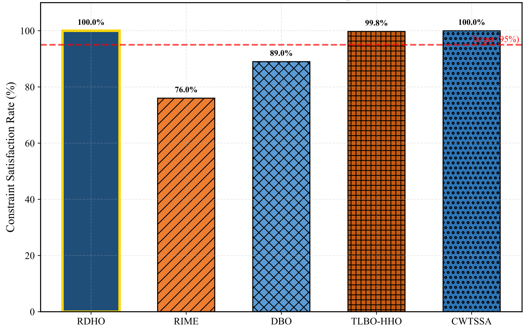
Constraint Satisfaction Rate Comparison
