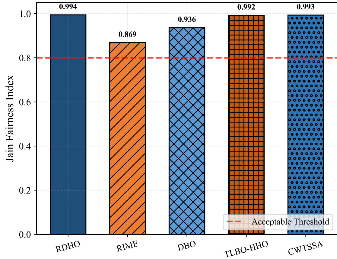
Fairness Comparison
