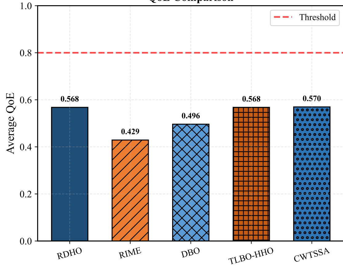
QoE Comparison
