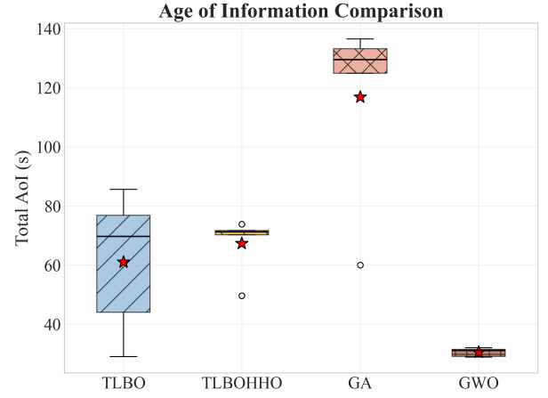
Fig. 6. Age of Information Comparison.
