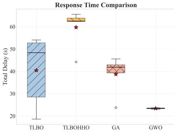
Fig. 3. Response Time Comparison.
