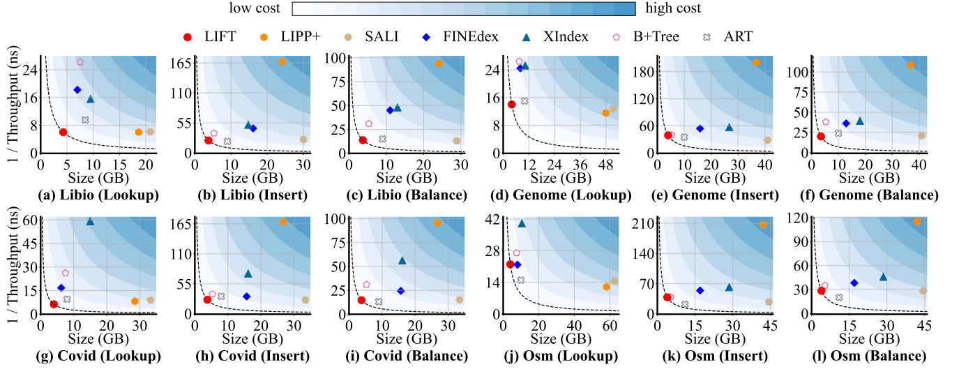
Figure 5: Time-space tradeoff evaluation with 64 threads on the Libio, Covid, Osm, and Genome datasets.
