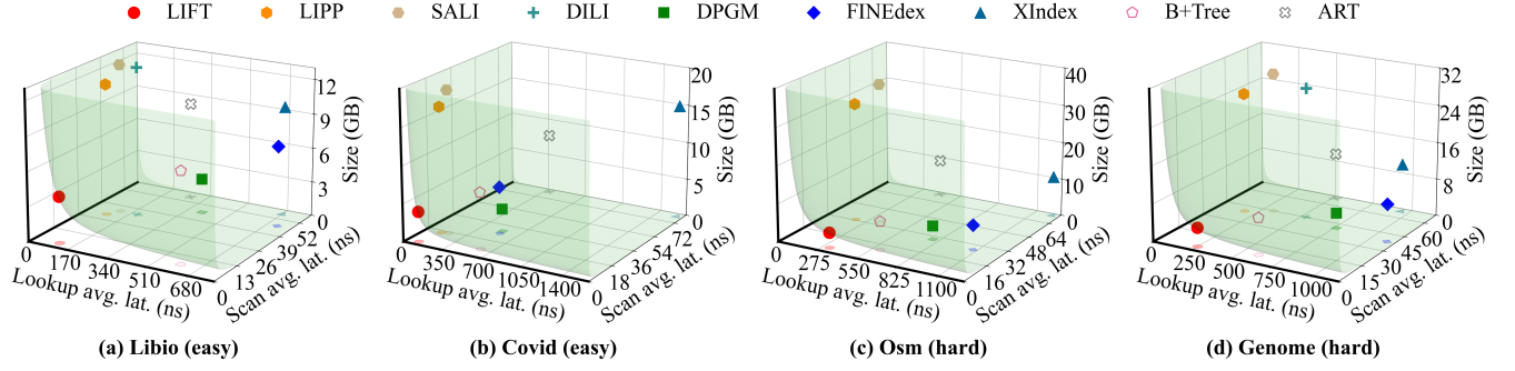
Figure 1: Look-up-scan-size tradeoff evaluation on the Libio, Covid, Osm, and Genome datasets.
