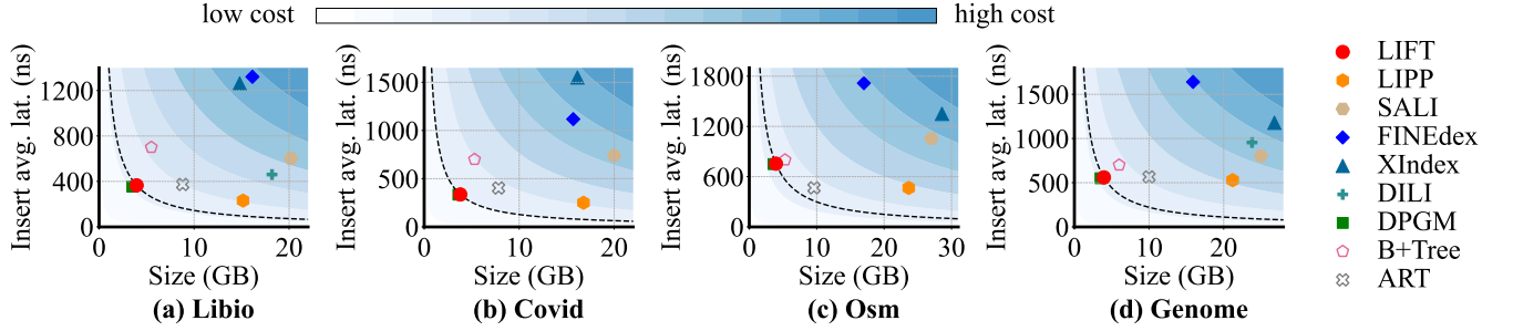
Figure 2: Insert-size tradeoff evaluation on the Libio, Covid, Osm, and Genome datasets.
