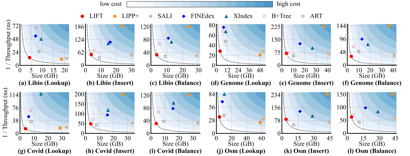
Figure 3: Time-space tradeoff evaluation with 16 threads on the Libio, Covid, Osm, and Genome datasets.
