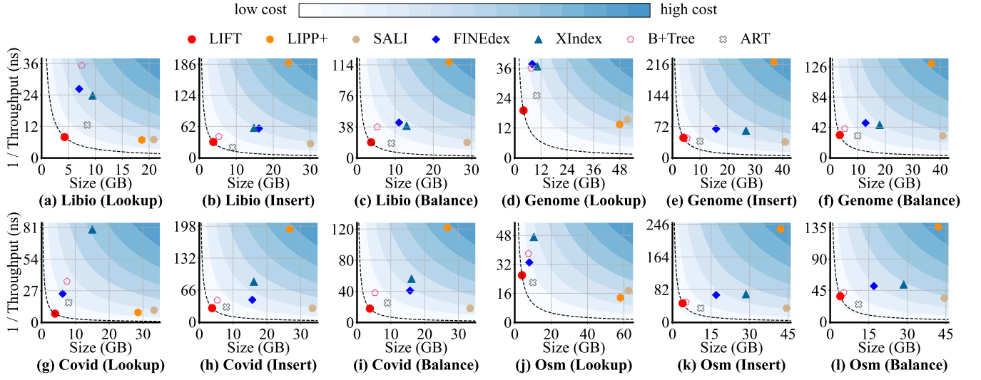
Figure 4: Time-space tradeoff evaluation with 32 threads on the Libio, Covid, Osm, and Genome datasets.
