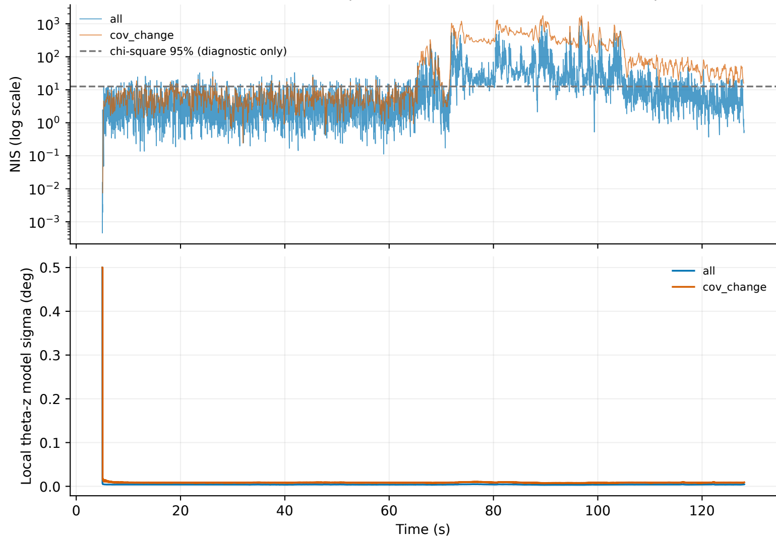
Correlation violates the independent-observation confidence interpretation
