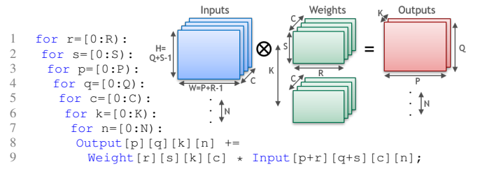
Fig. 3. Convolutional layer 7D loop nest.
