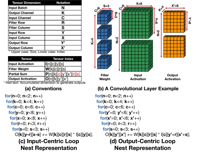
Figure 1: Convolutional layer example
