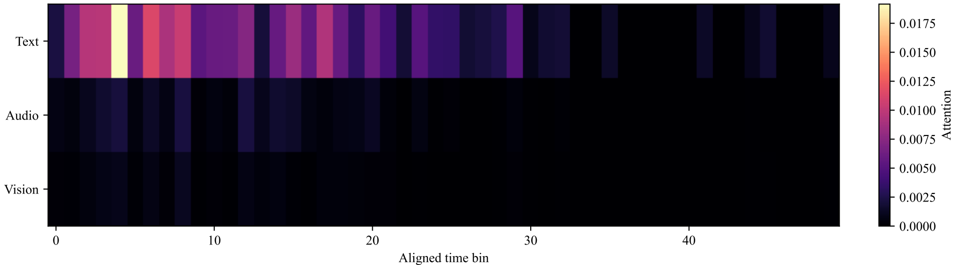
Top-evidence attention distribution
