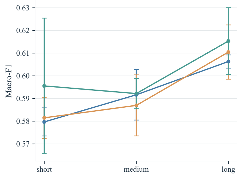
Test: Text
