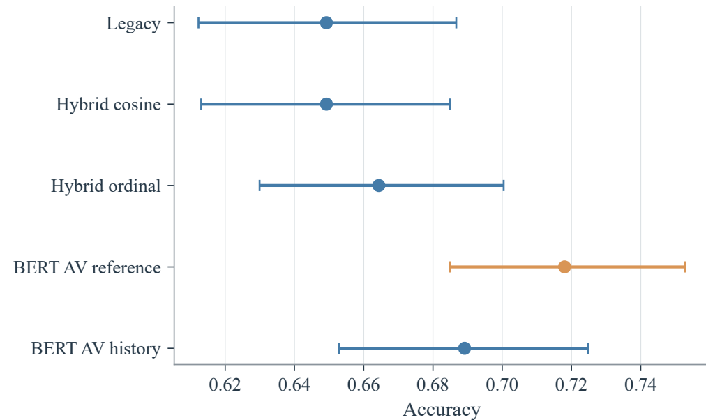
(a) Accuracy
