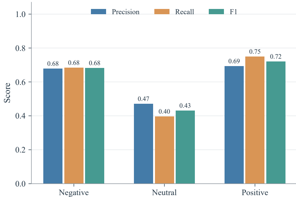
(a) Valid
