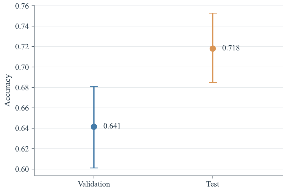
(a) Accuracy
