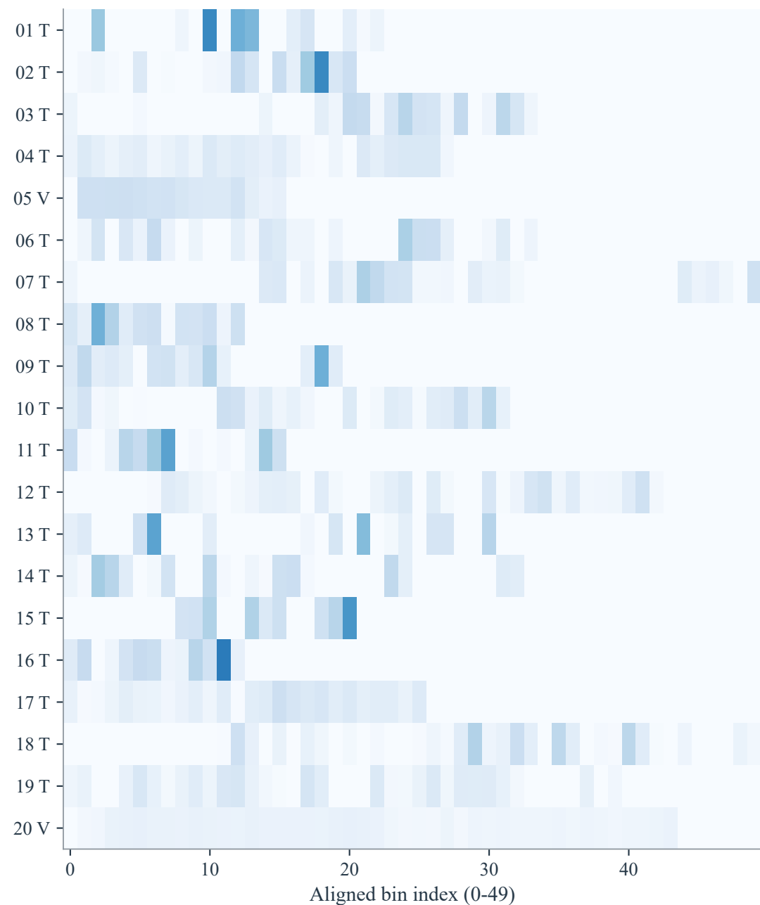
Aligned
