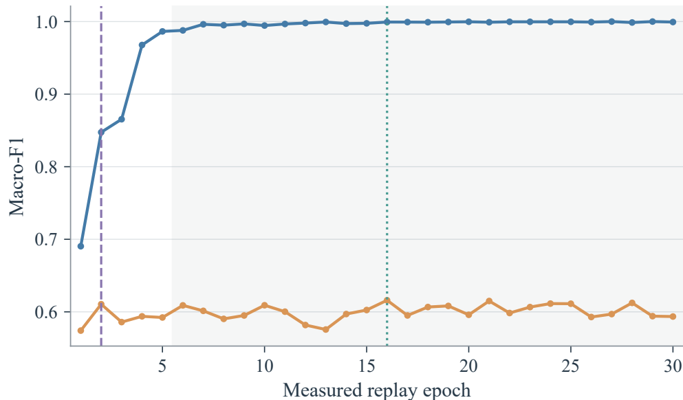
(c) Macro-F1
