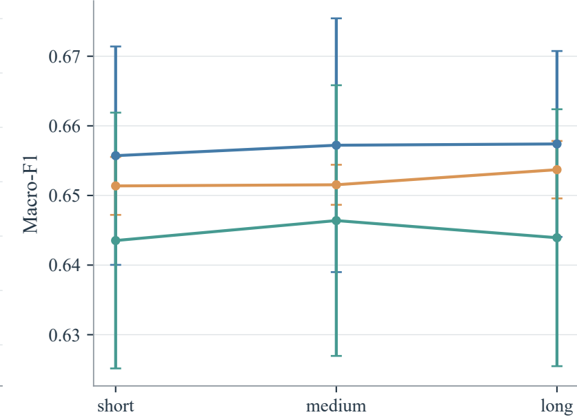
Test: Audio
