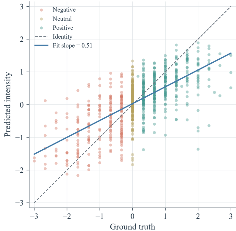
(a) Valid
