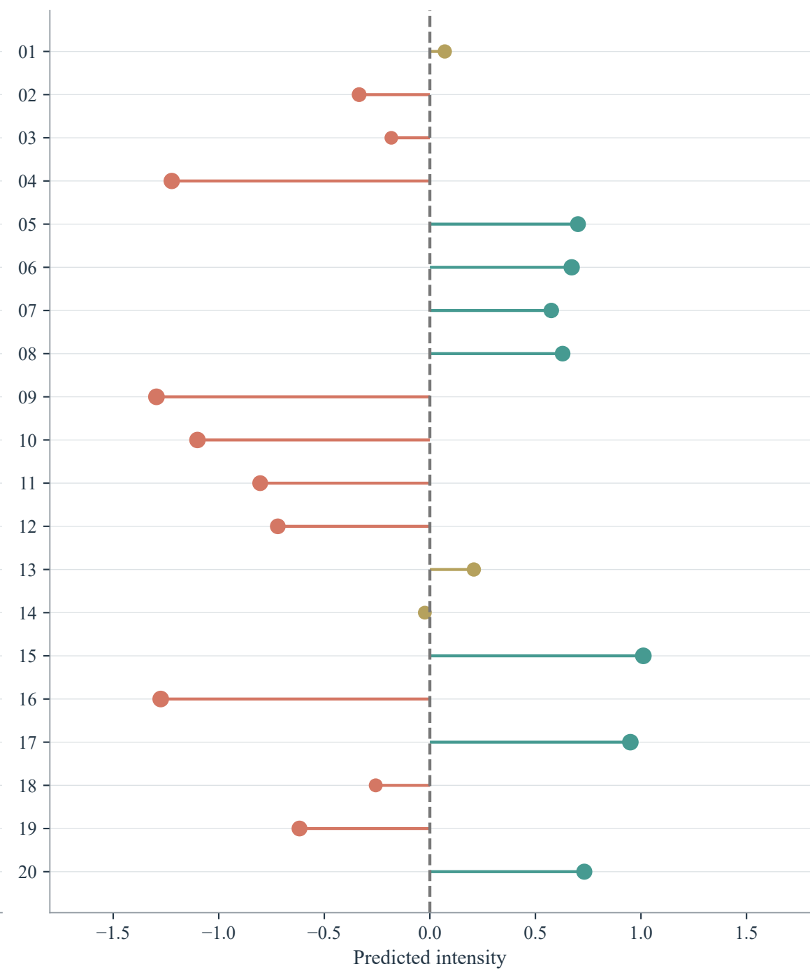
Unaligned
