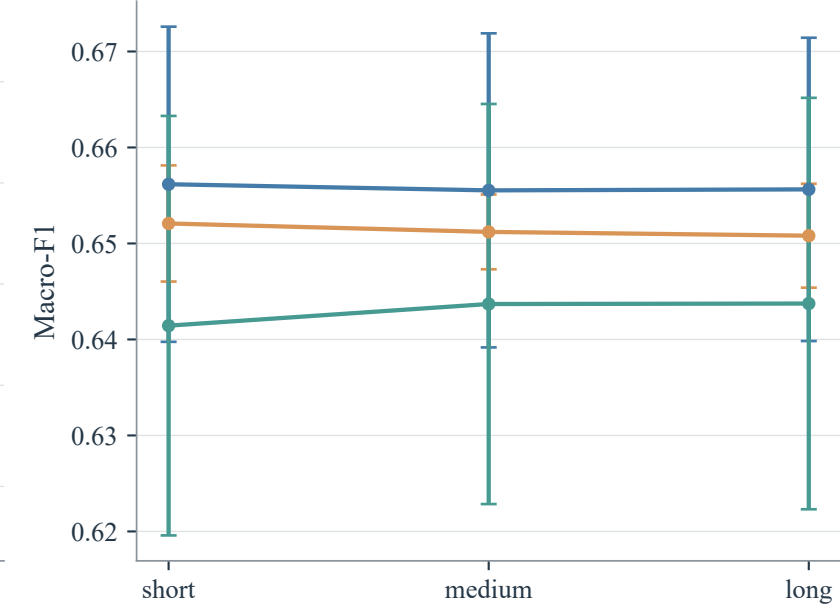
Test: Vision
