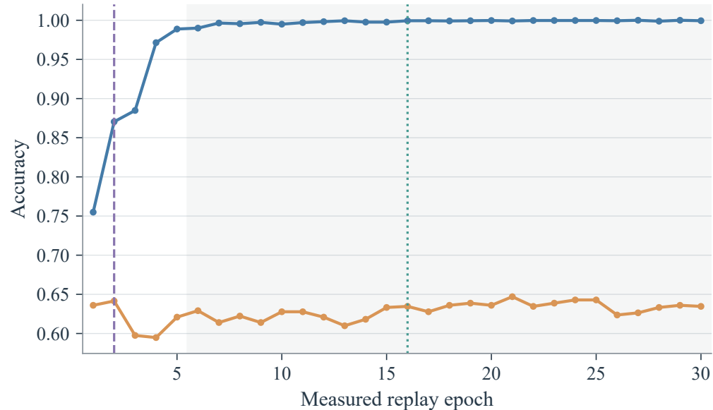
(b) Accuracy
