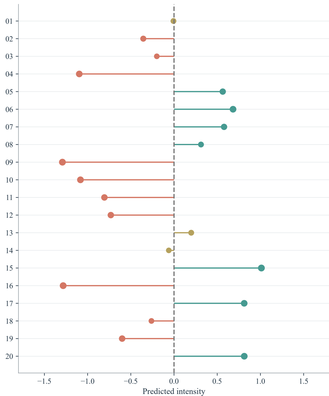
Aligned
