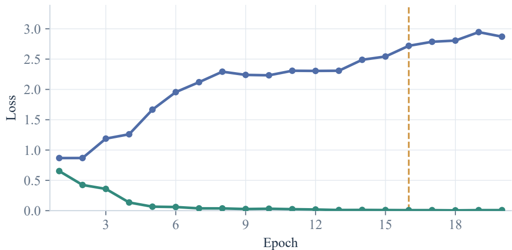
(a) Joint loss
