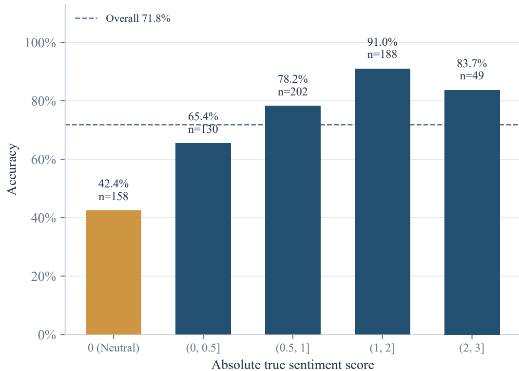
(a) Accuracy by sentiment intensity
