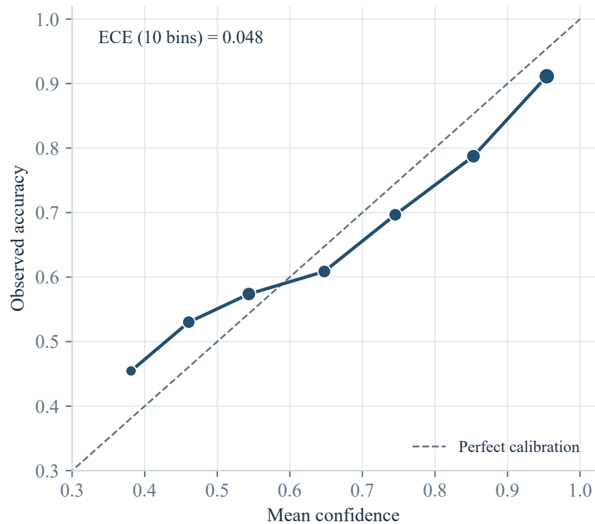
(b) Reliability diagram
