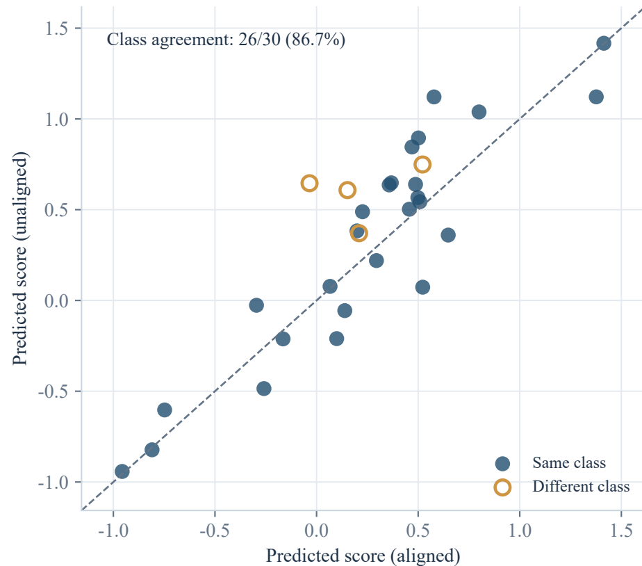
(b) Paired predictions
