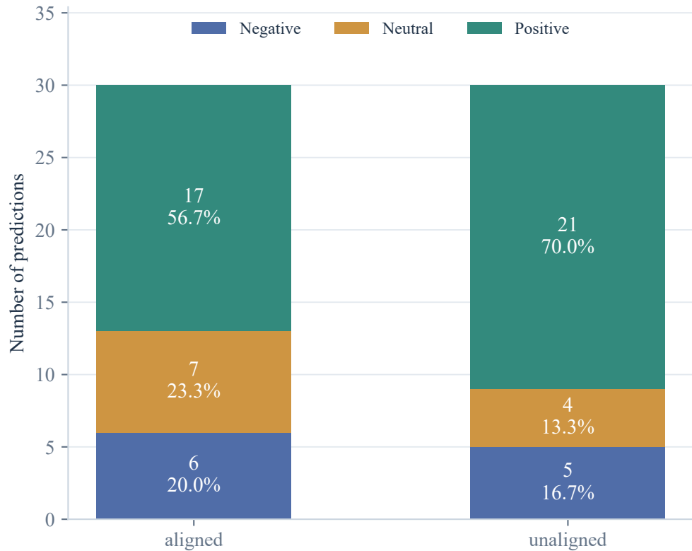
(a) Predicted class distribution
