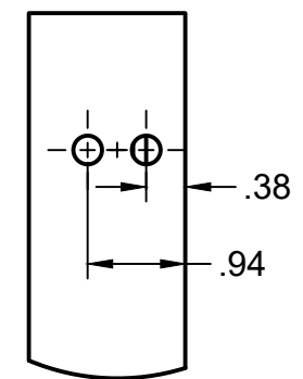
DETAIL B SCALE 1:2
