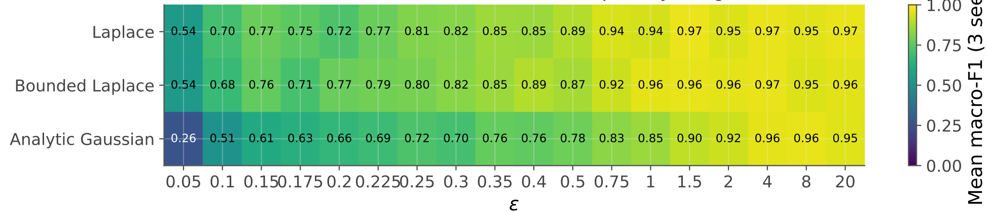
Macro-F1 across mechanism and privacy budget
