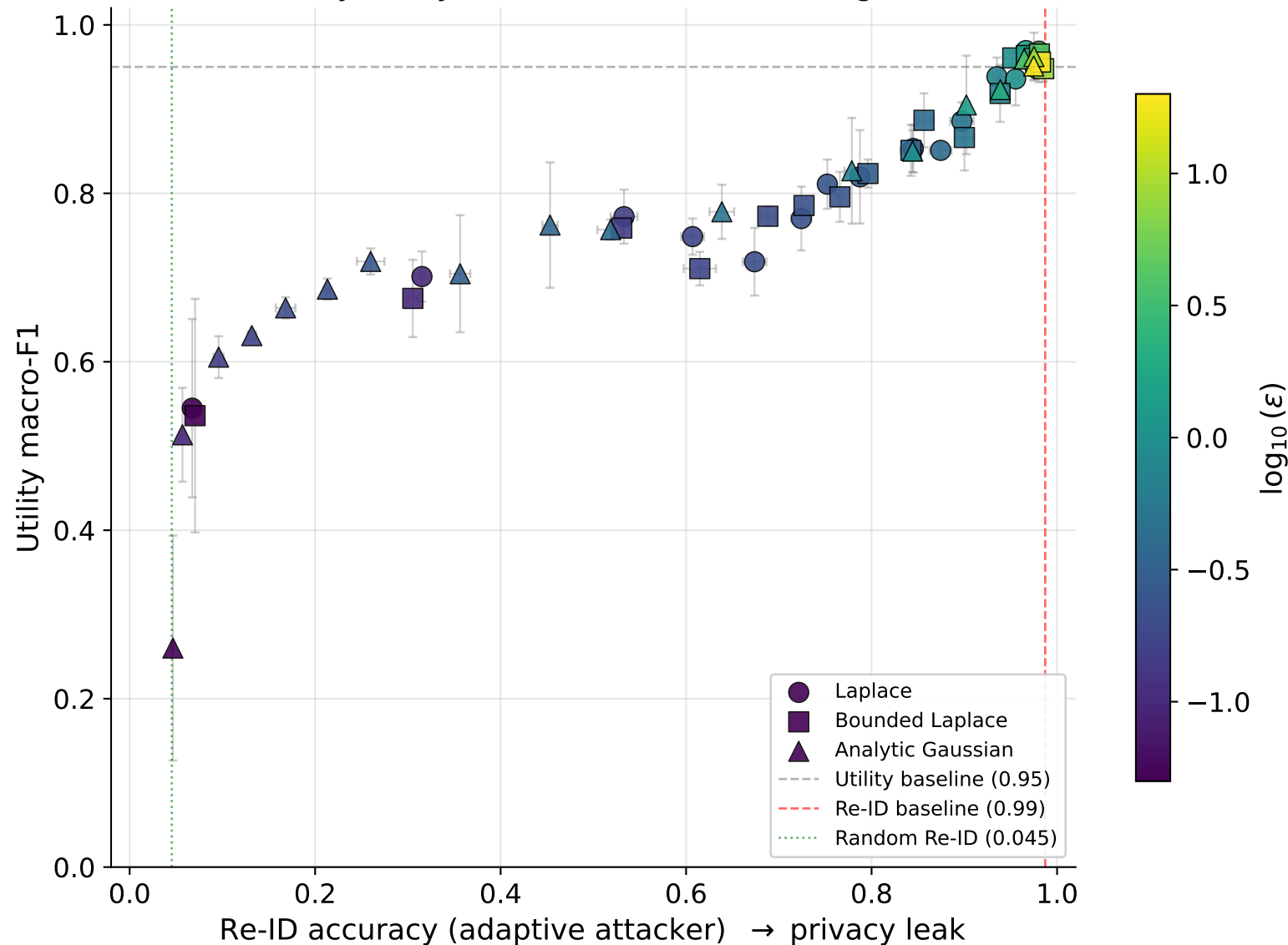
Privacy-utility trade-off, within-recording test
