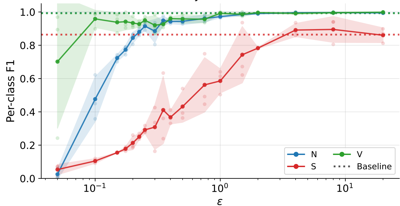
Analytic Gaussian
