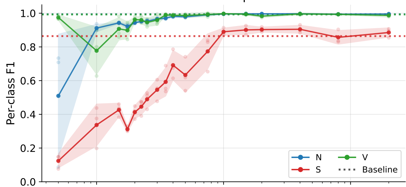
Analytic Gaussian
