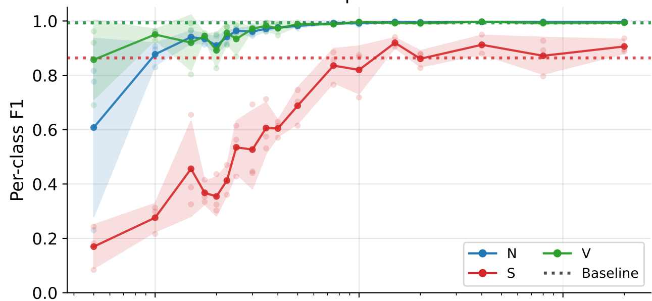
Bounded Laplace
