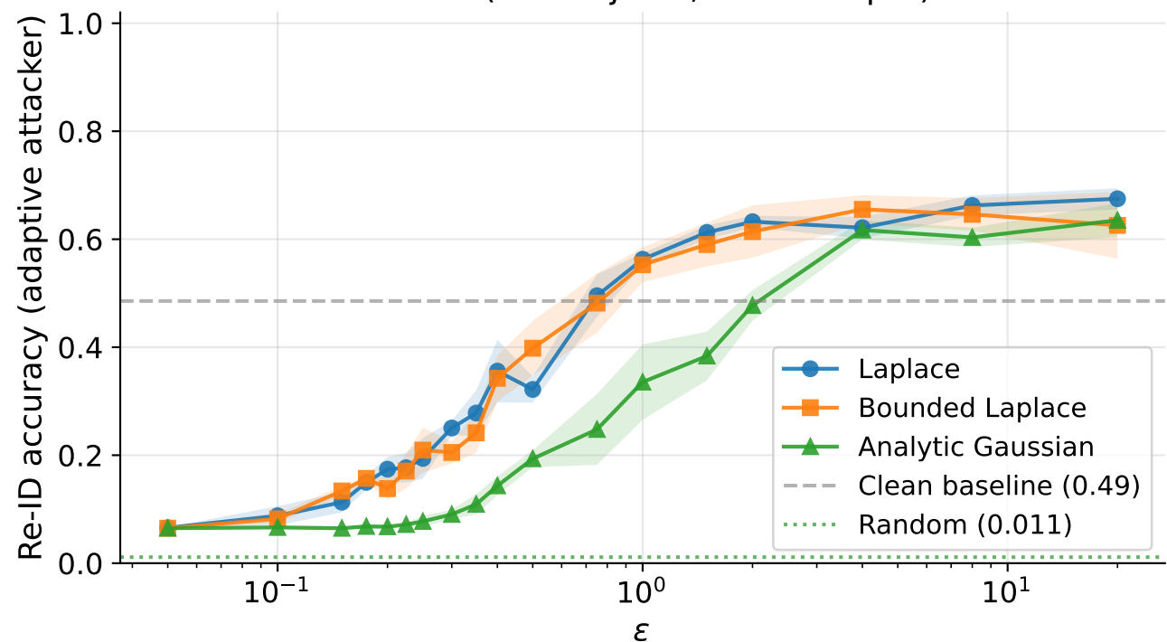
ECG-ID (89 subjects, session-split)
