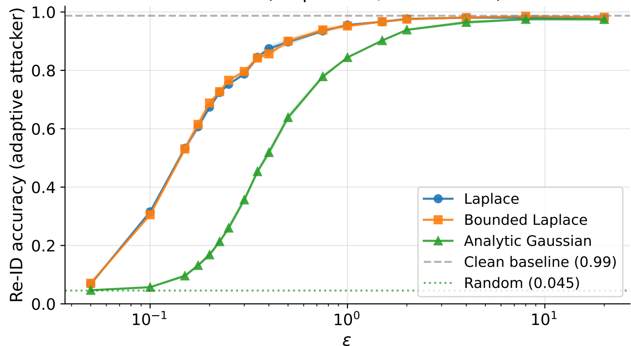
MIT-BIH (22 patients, intra-record)
