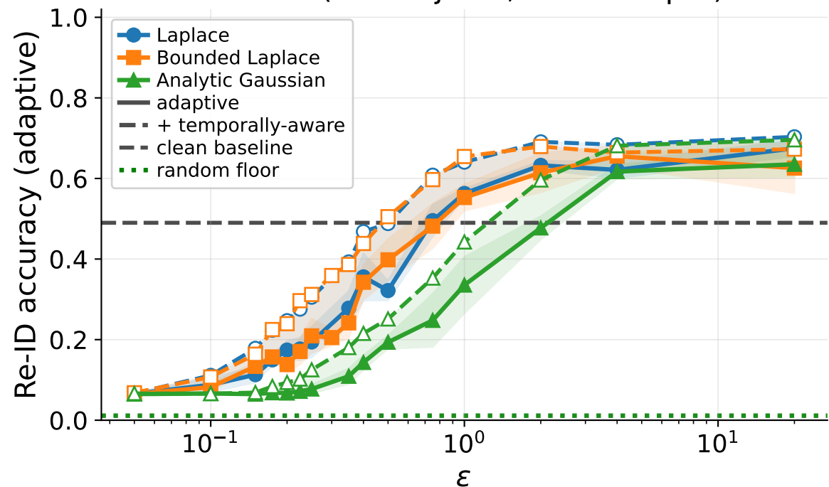
ECG-ID (89 subjects, session-split)
