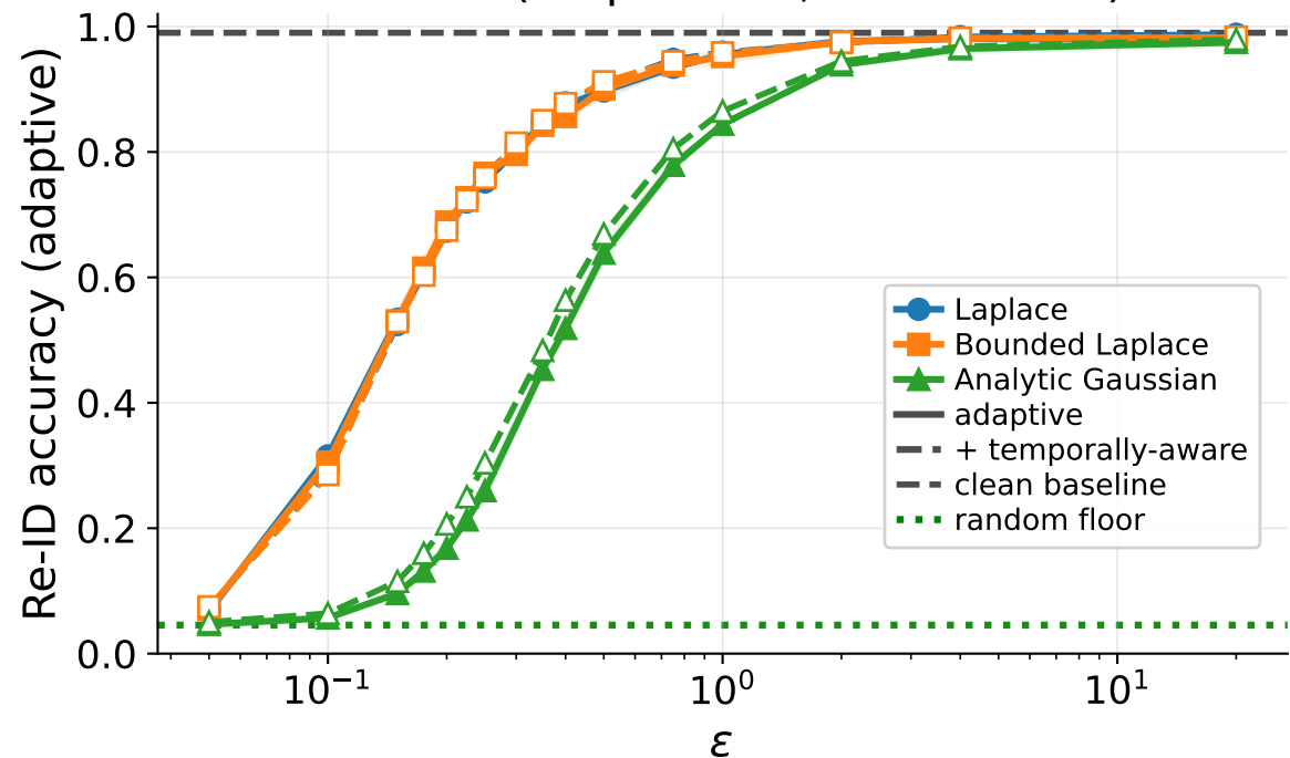
MIT-BIH (22 patients, intra-record)
