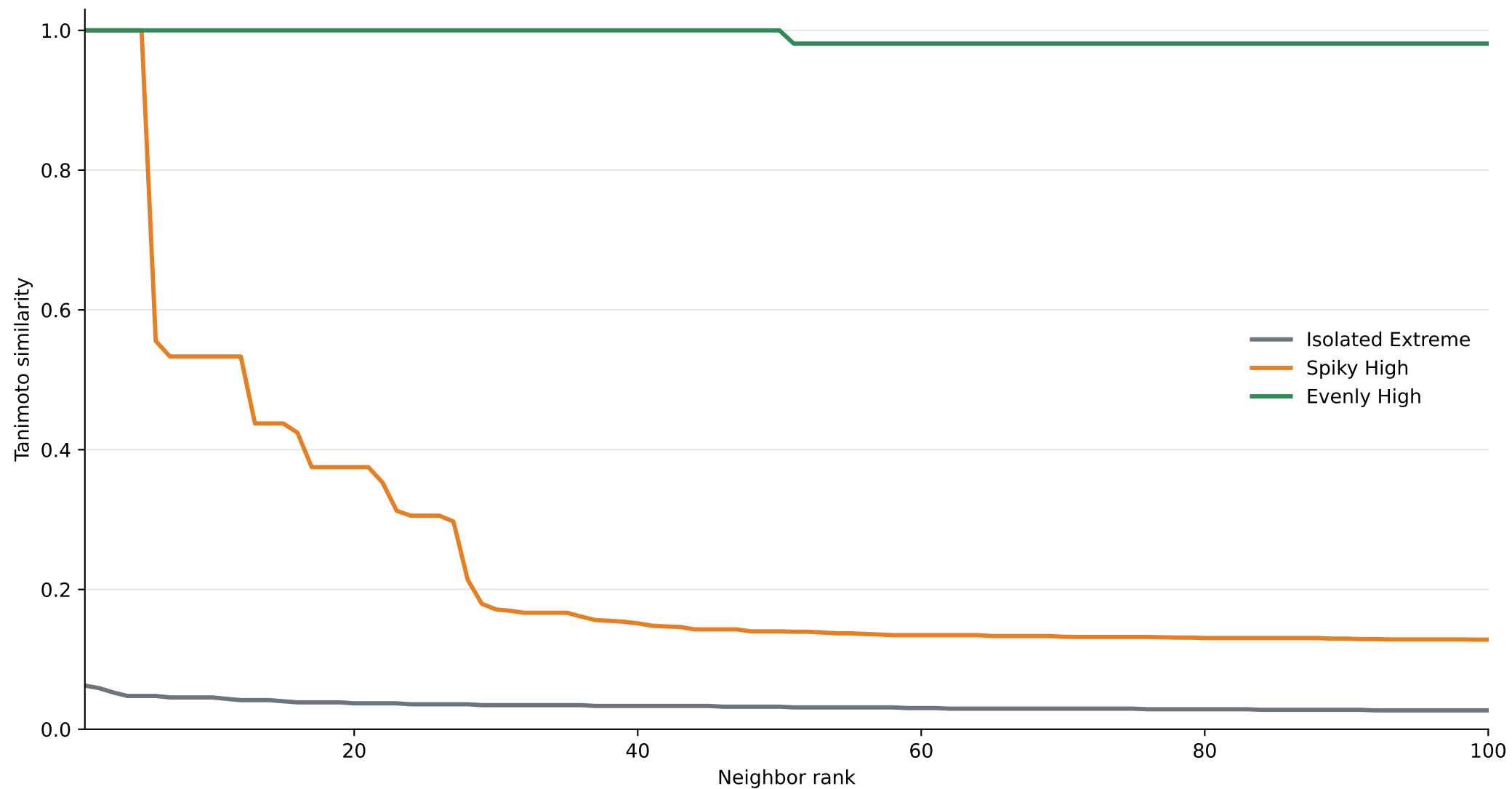
Rank Profiles of the Three Selected Molecules
